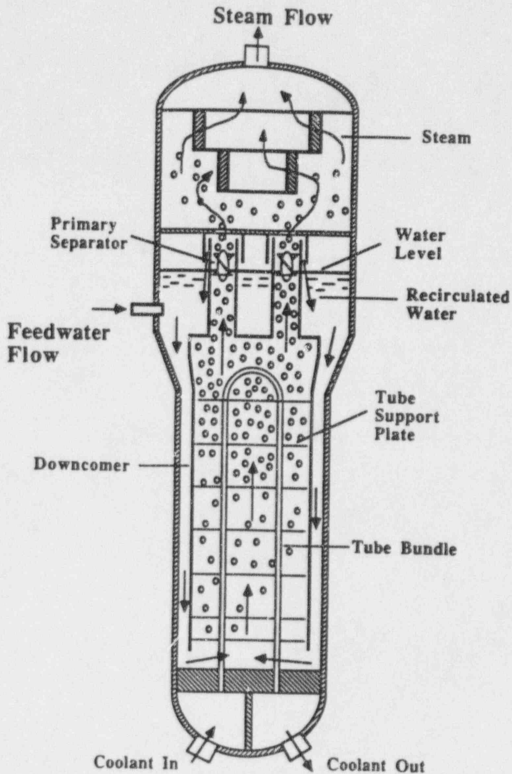
Figure 4-68. Diagram of Flow Circulation During Power Operation
