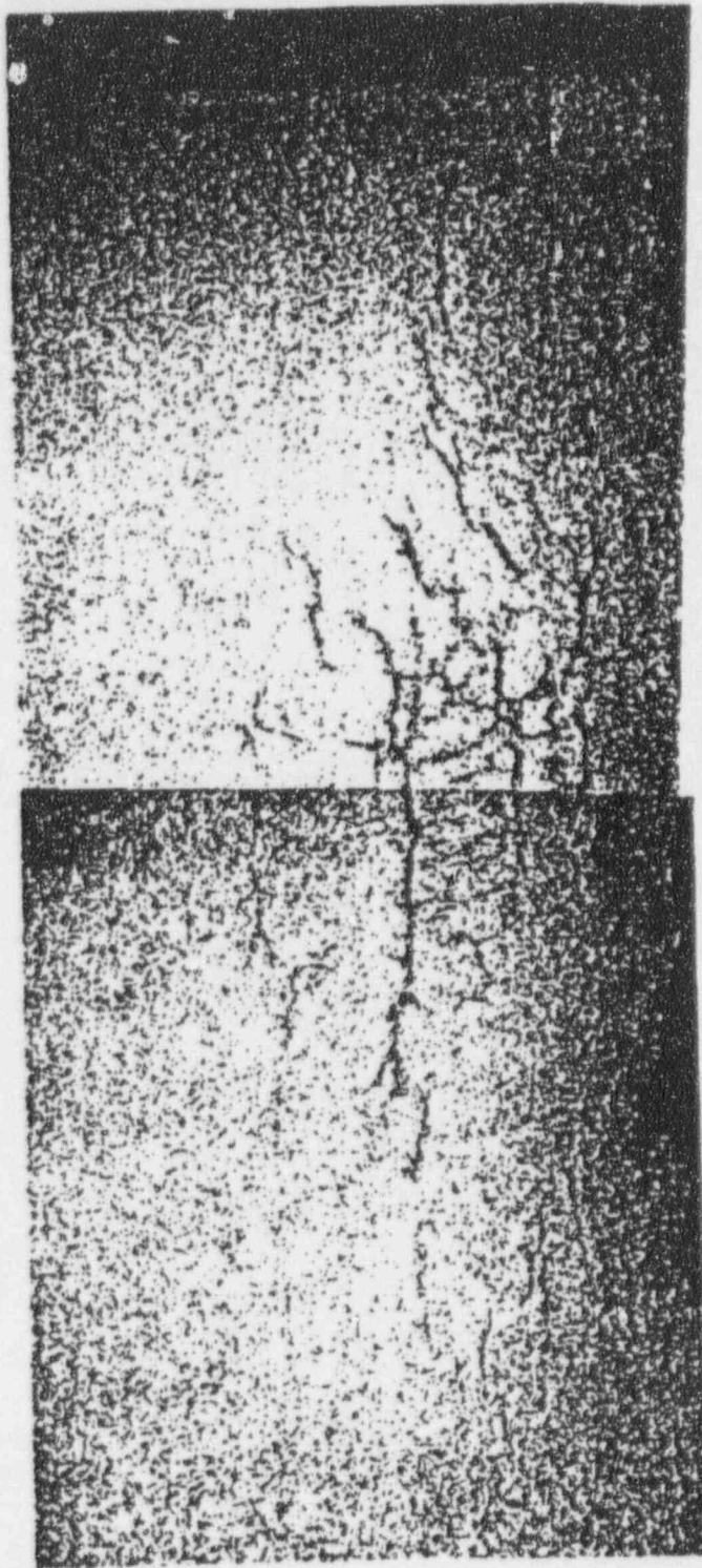
Figure 3-6 Example of intergranular cellular corrosion (ICC) as observed by radial metallography in the SP5 crevice region of tube R37-C34, 21% depth, 16X magnification.
