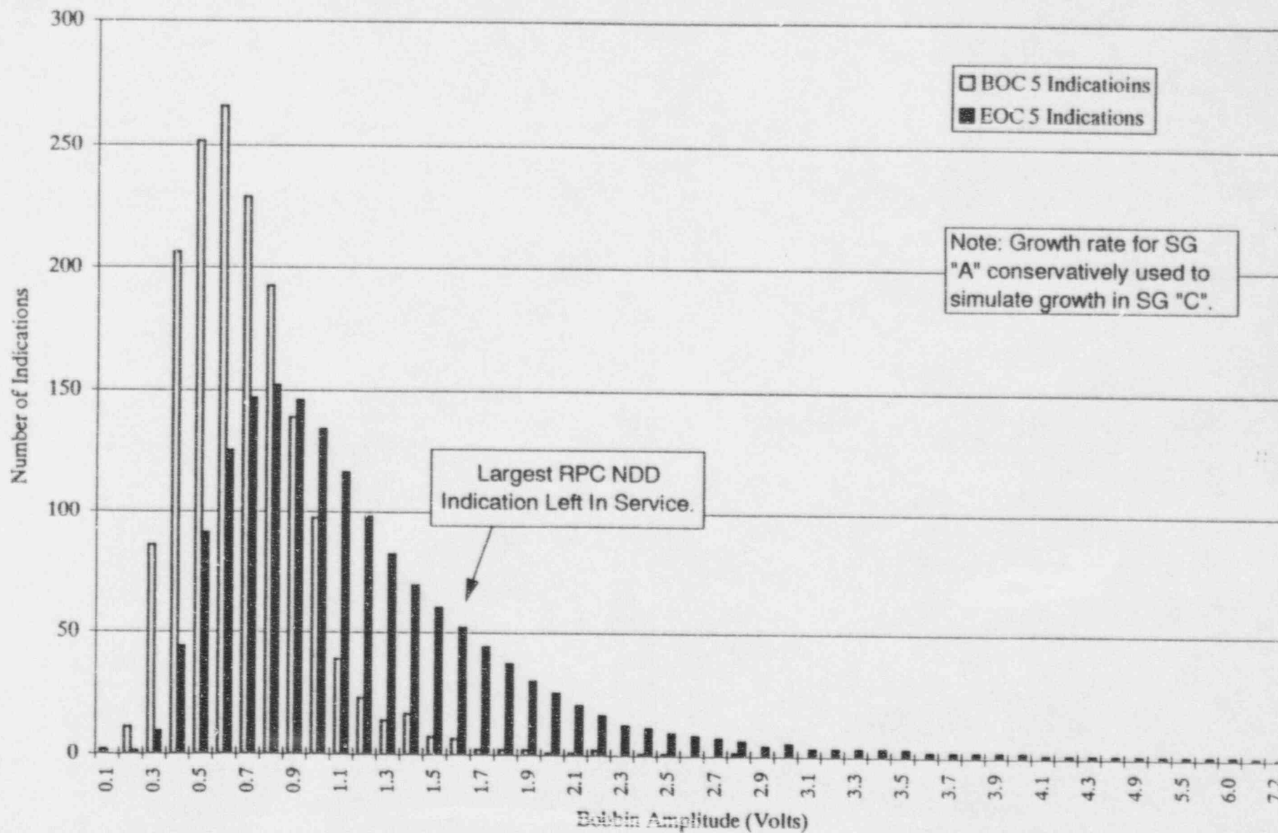
Figure 8-4: Braidwood 1, SG "C" BOC & EOC 5 Indications
