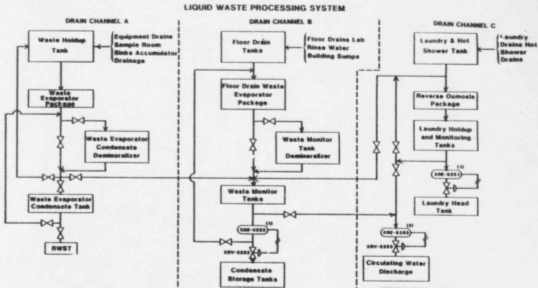
FIGURE 1.1 (page 2 of 2) LIQUID EFFLUENT DISCHARGE PATHWAYS
