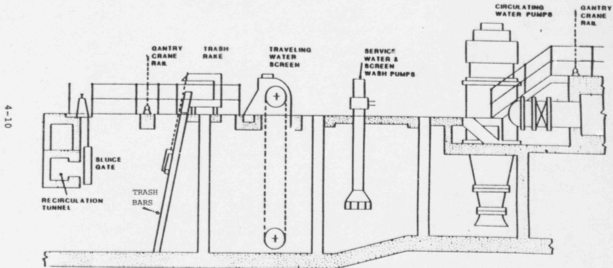
INTAKE STRUCTURE, SECTION
