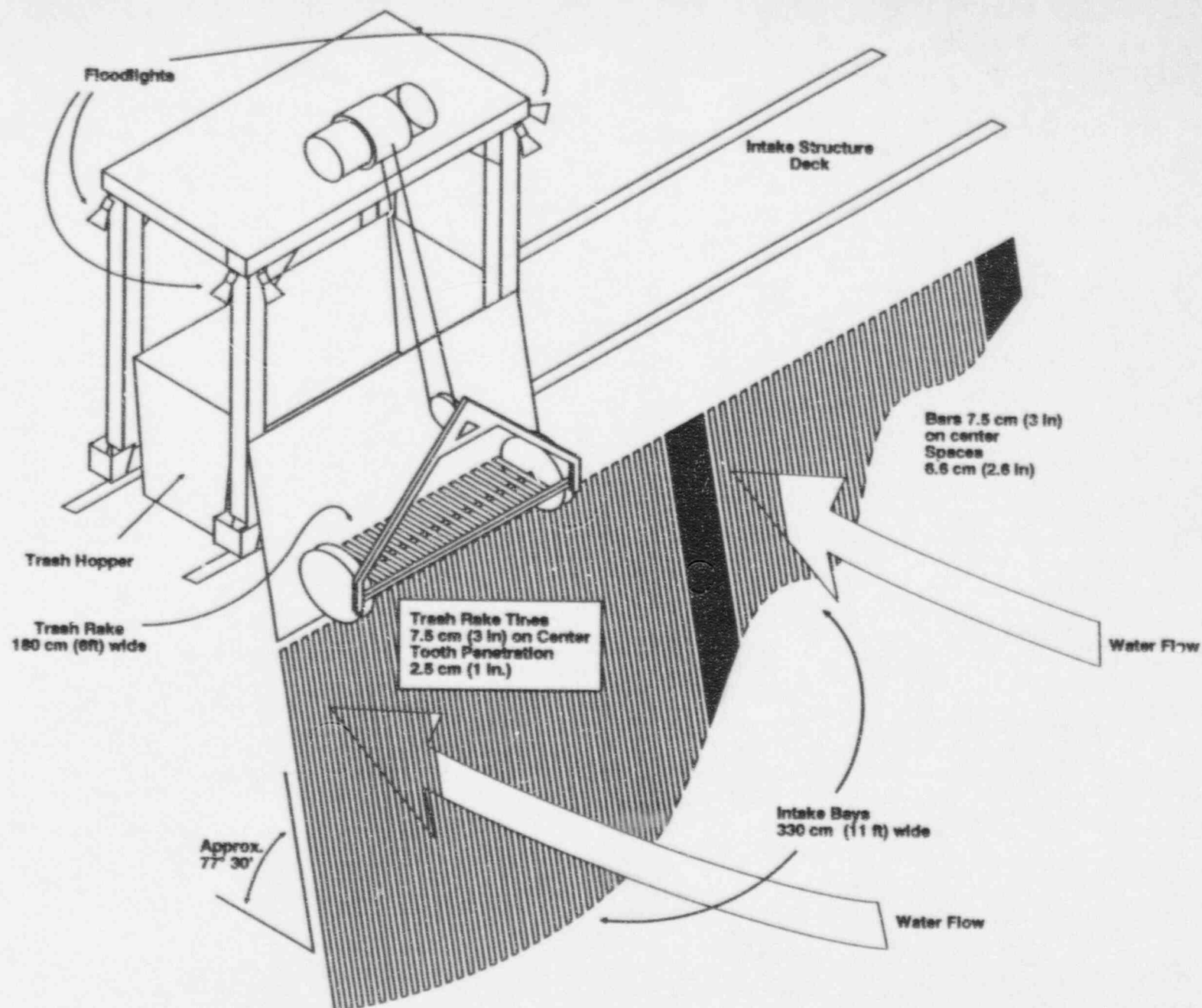
Figure 4-5. Schematic of Circulating Water System (CWS) and Dilution Water System (DWS) intake structures showing trash cart, trash rake & trash bars.
