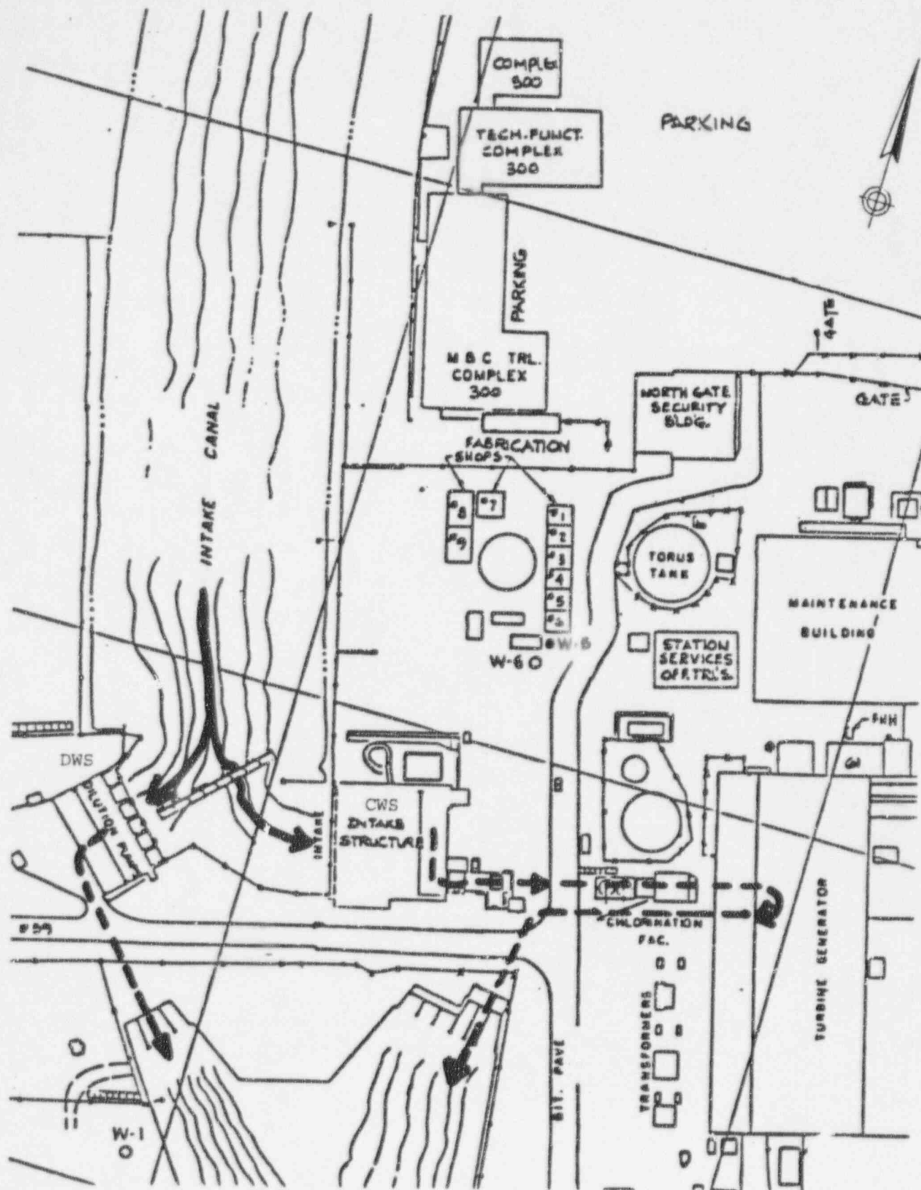
Figure 4-2. Schematic diagram of the OCNCS circulating water system (CWS) and dilution water system (DWS) flows.
