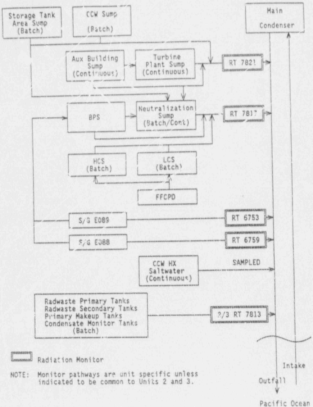
FIGURE 4-5: SONGS 2&3 RADIOACTIVE LIQUID WASTE TREATMENT SYSTEMS
