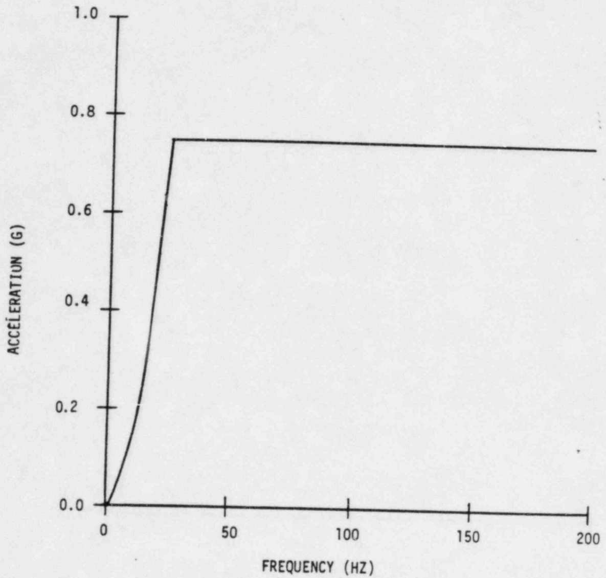
Fig. 1: Plant Induced Vibration Linear Spectra
