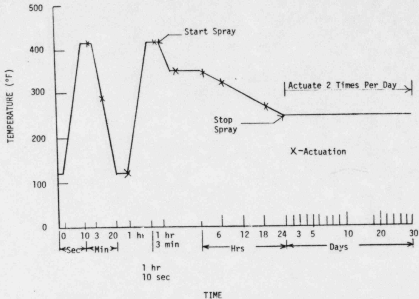
Figure 8 Test Chamber Profile for Accident Environment Simulation
