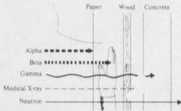
The various types of ionizing radiation have different penetrating powers. This portrays the ability of different forms of ionizing radiation to penetrate paper, the human body, wood, and concrete.
