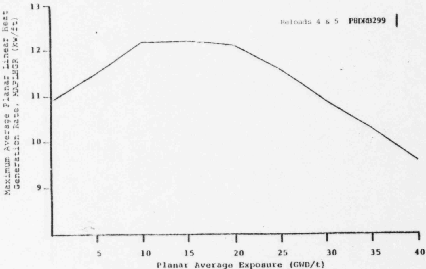
Maximum Average Planar Linear Heat Generation Rate (MAPLHGR) Versus Planar Average Exposure
