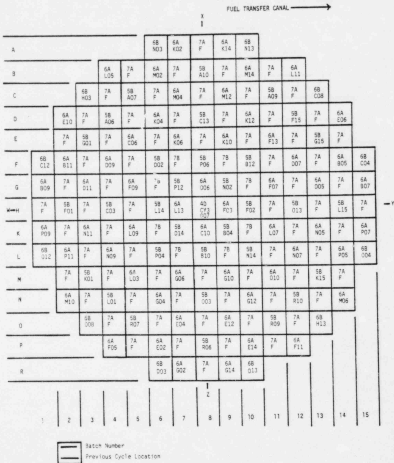
Figure 3-1. Fuel Shuffle for Crystal River 3 Cycle 5
