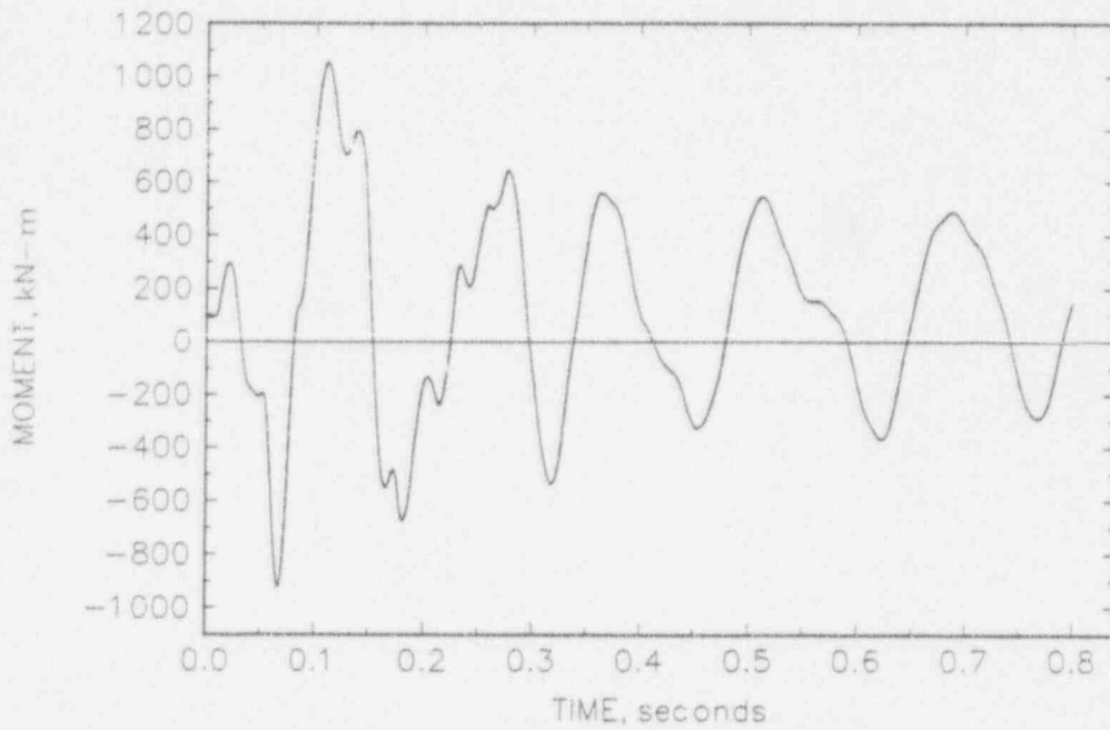
(a) Y direction
