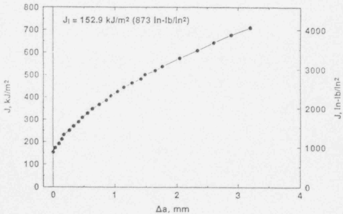
Figure 4.23 Typical J-R curve for test section material 20 MnMoNi 5 5, L-T orientation C(T) data
