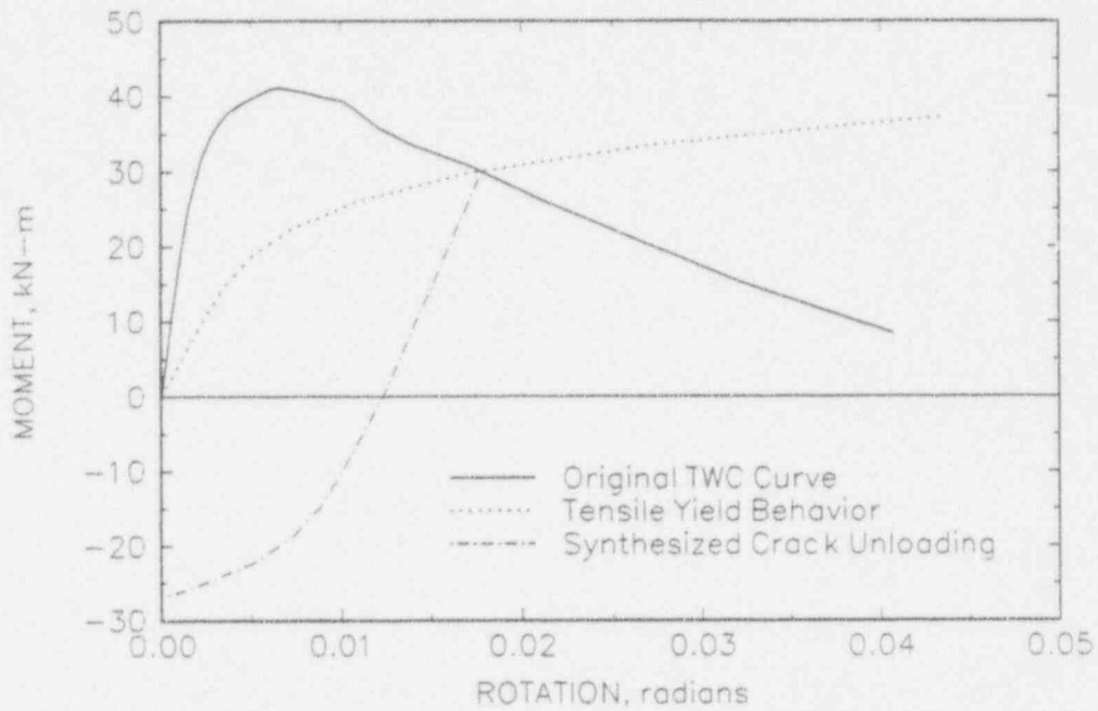
Figure 3.41 Crack unloading and compressive behavior model
