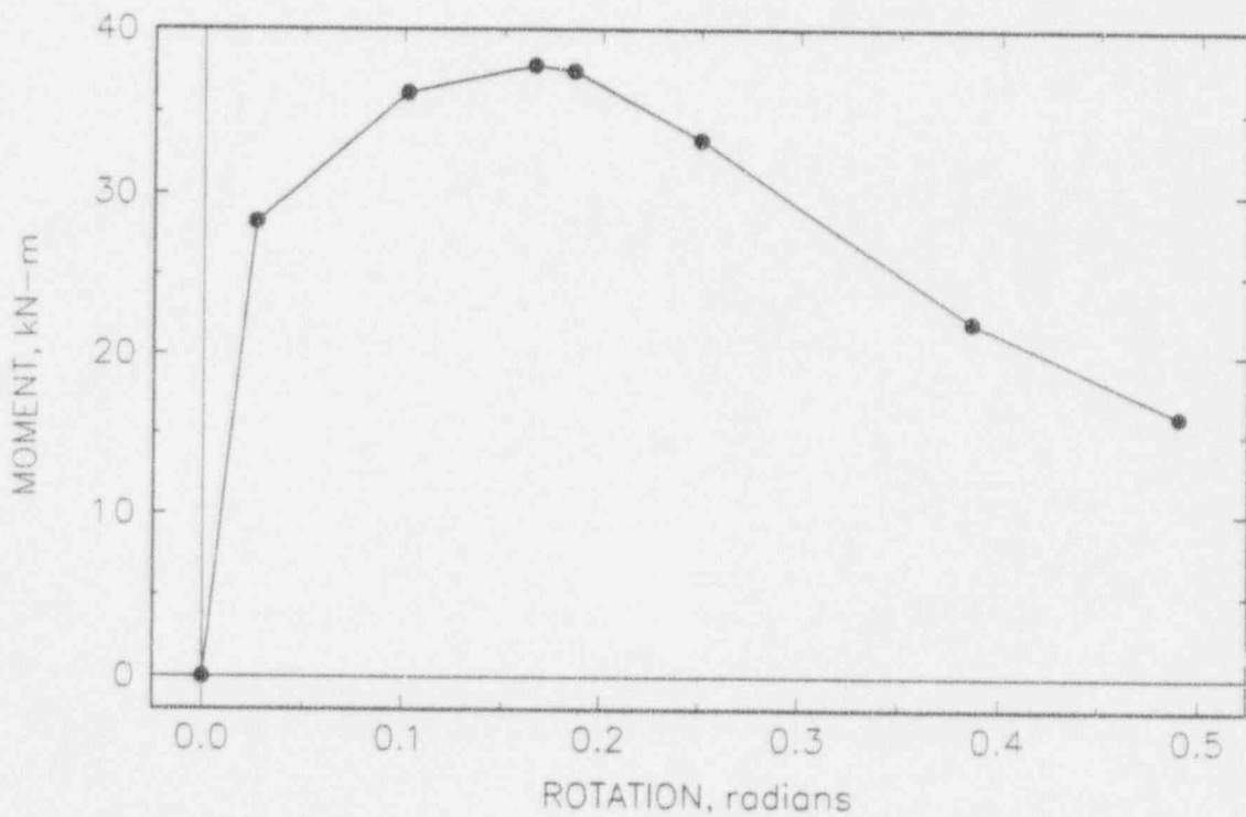
Figure 3.20 Input moment-rotation response for a through-wall crack in a pipe
