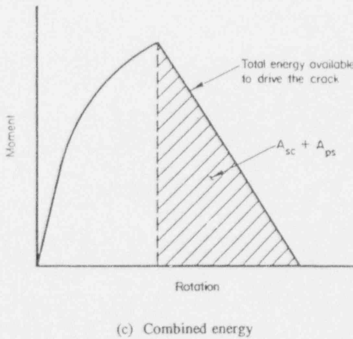
Figure 2.9 Energy available for driving an instability
