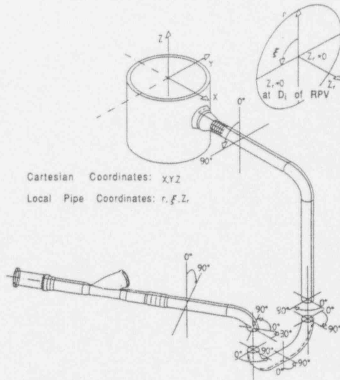
Figure 4.11 HDR-E31 piping coordinate systems
