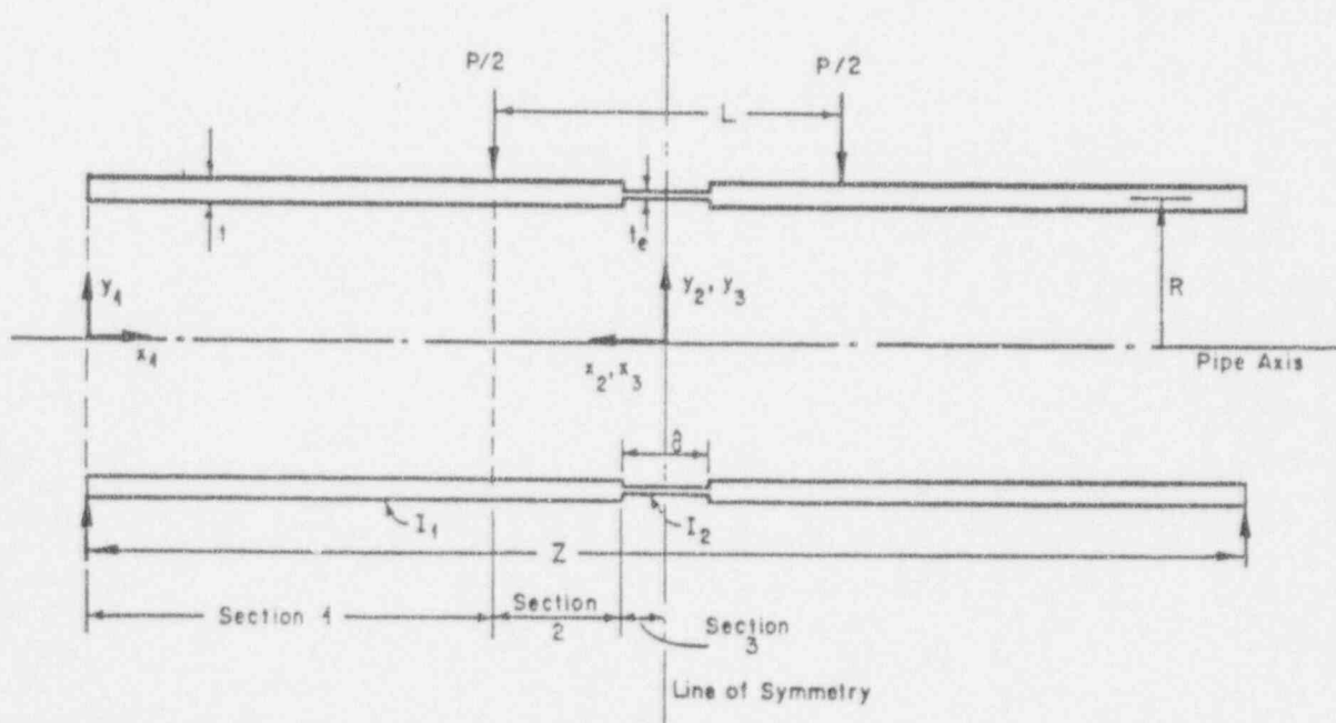
Figure 3.2 LBB.ENG reduced section for modeling cracked pipe response
