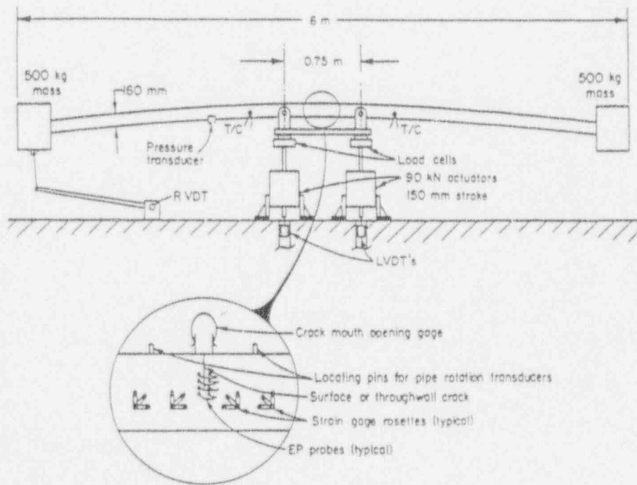
Figure 3.6 IPIRG-1 Subtask 1.1 inertial loading cracked pipe experimental facility
