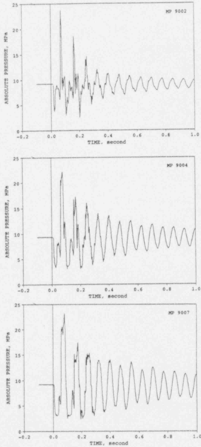
Figure 4.15 Pressures used for calculating elbow forces for HDR-E31.2
