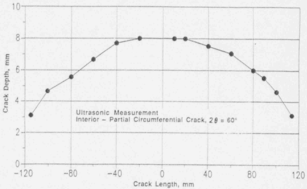
Figure 4.22 Initial flaw profile for HDR-E31.3
