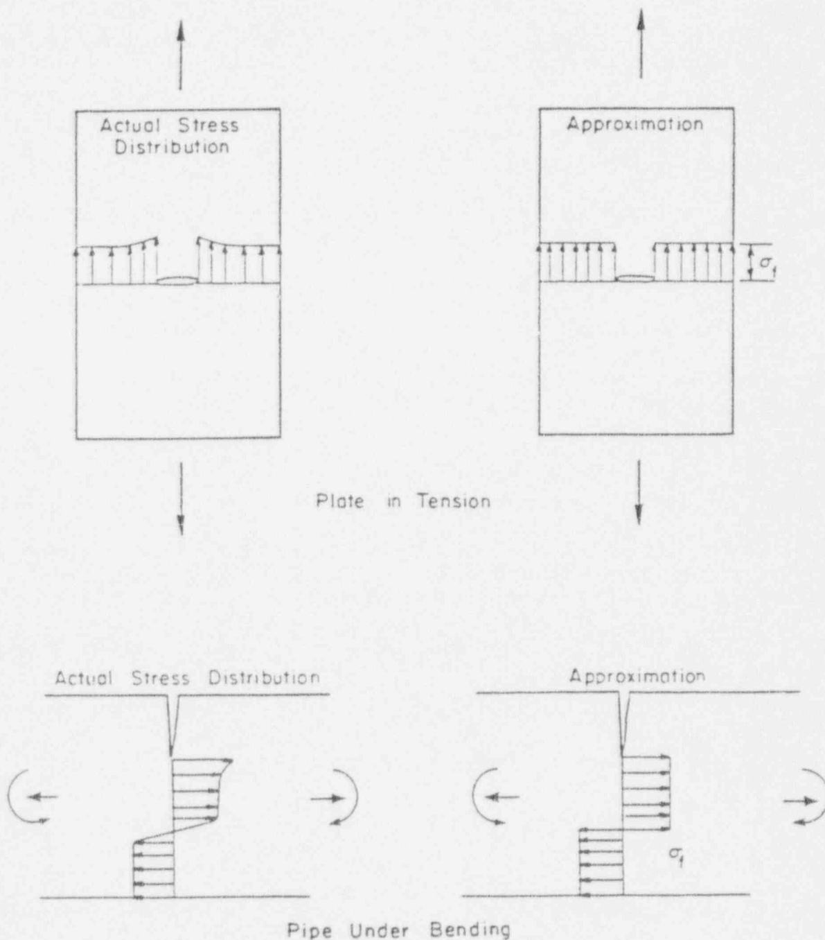
Figure 2.1 Net-Section-Collapse criteria
