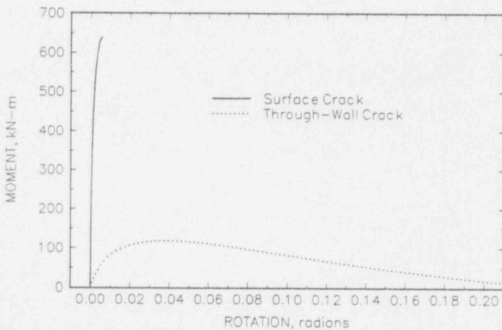
Figure 3.36 Input moment-rotation response for IPIRG-1 Experiment 1.3-7 from J-estimation scheme analyses
