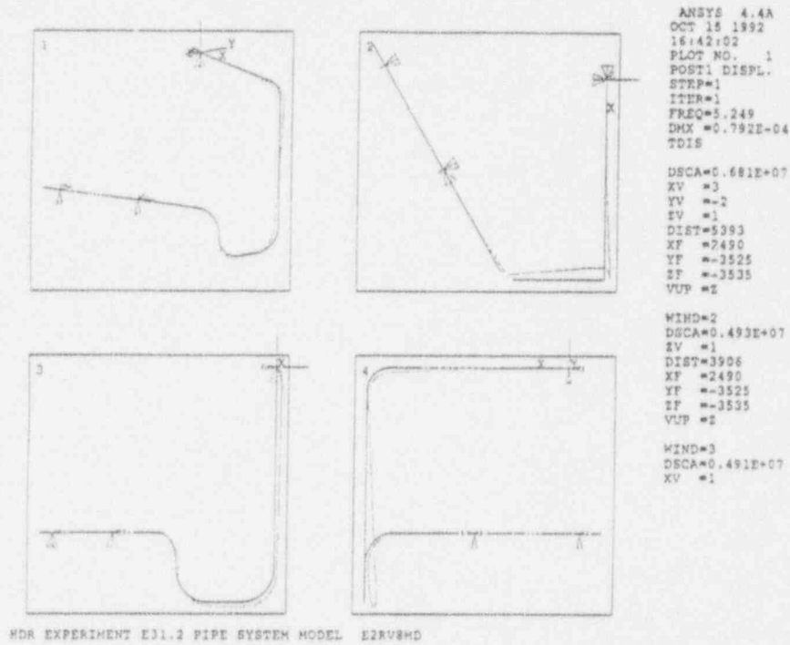
Figure 5.3 Mode 1 of the HDR-E31 test system
