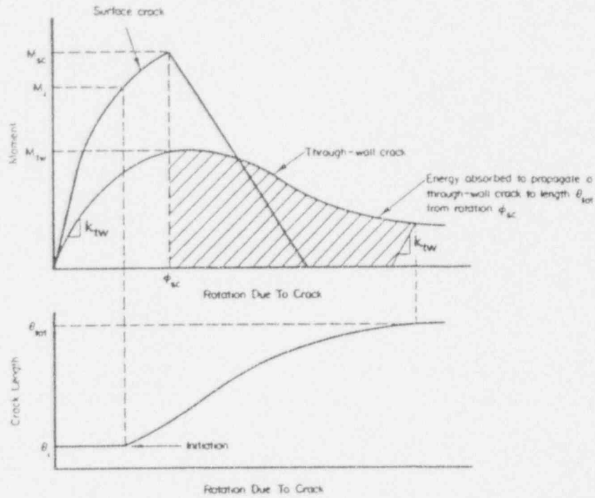
Figure 2.10 Crack propagation behavior
