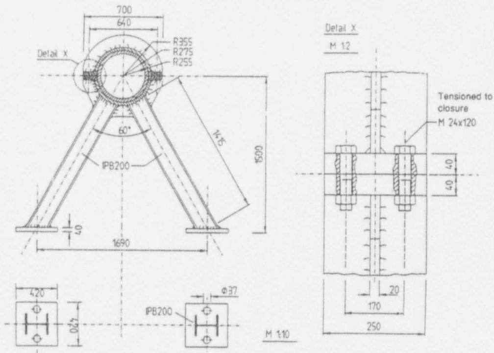
Figure 4.5 Pipe restraint section at the Fixed Point (Units in mm)
