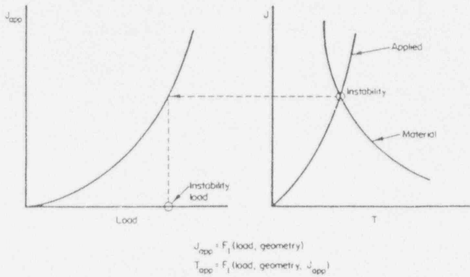
Figure 2.7 J/T stability assessment methodology
