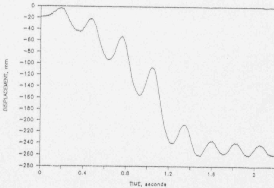
(b) Inertial mass displacements from experiment
