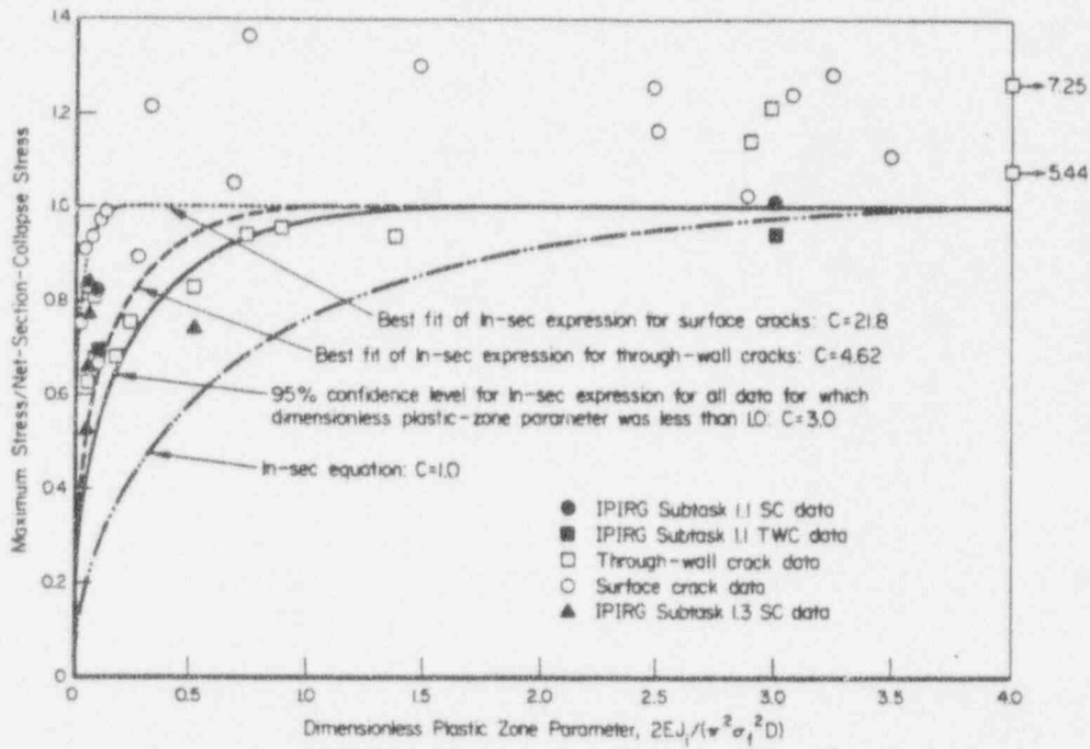
Figure 2.5 Dimensionless Plastic-Zone Parameter data [ \sigma_f = (\sigma_y + \sigma_w)/2 ]
