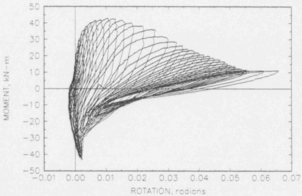
Figure 3.42 IPIRG-1 Experiment 1.2-4 (displacement controlled loading, carbon steel through-wall crack) R=-1 moment-rotation response
