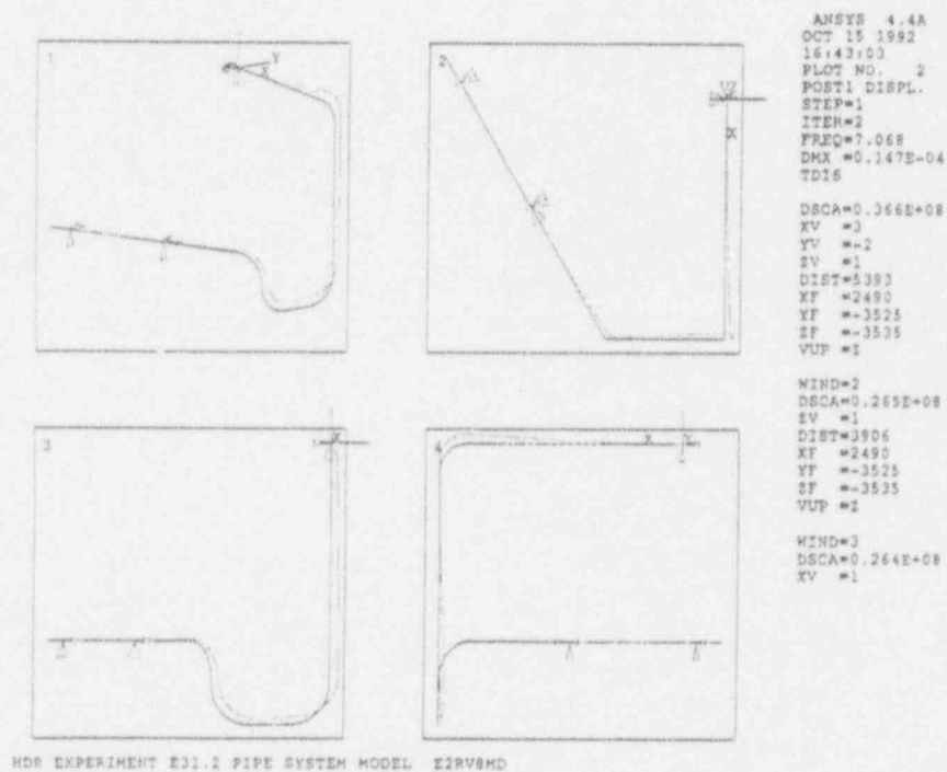
Figure 5.4 Mode 2 of the HDR-E31 test system
