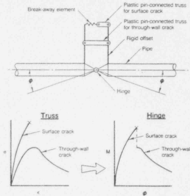
Figure 3.33 Model of surface crack to through-wall crack transition using plastic trusses
