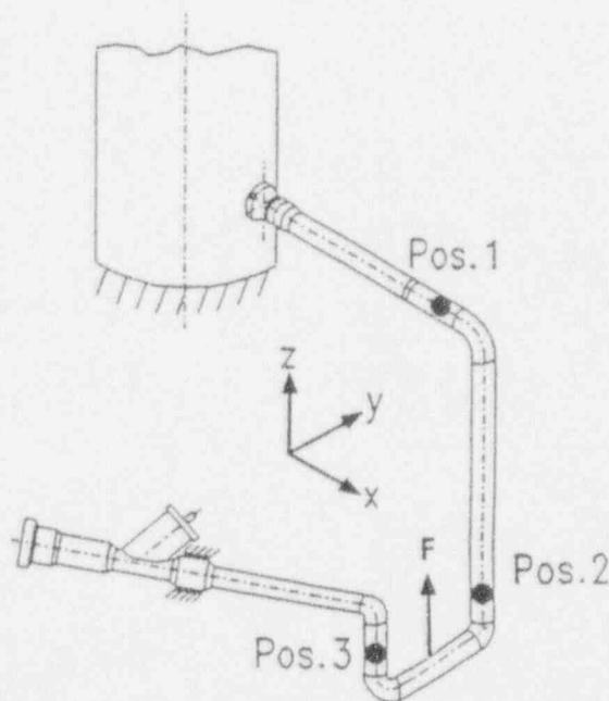
Figure 4.13 Displacement measurement locations for the HDR-E31 tests and point of static load application (F)
