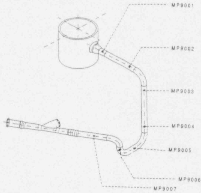
Figure 4.12 Pressure gage locations for HDR-E31 tests
