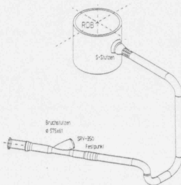
Figure 5.1 HDR-E31 experimental facility schematic (Units in mm)
