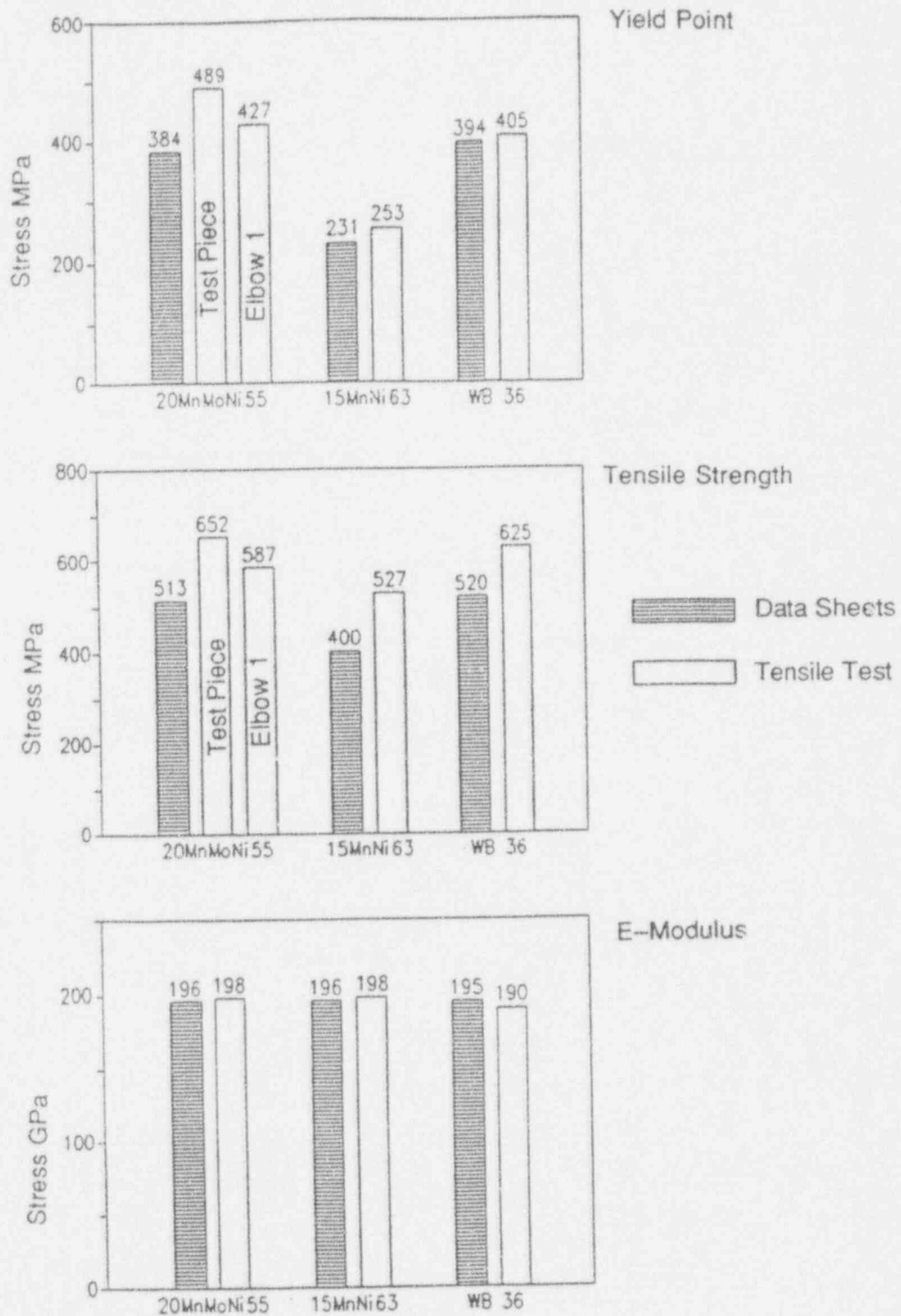
Figure 4.7 Comparison of measured mechanical properties of the HDR-E31 pipe components with data sheet values at 240 C (464 F)
