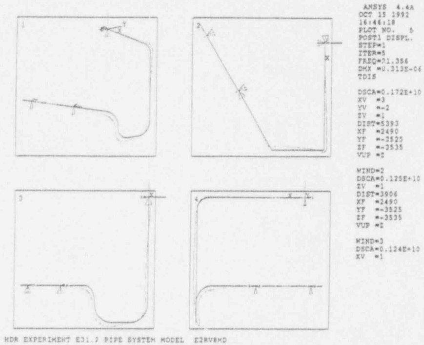
Figure 5.7 Mode 5 of the HDR-E31 test system
