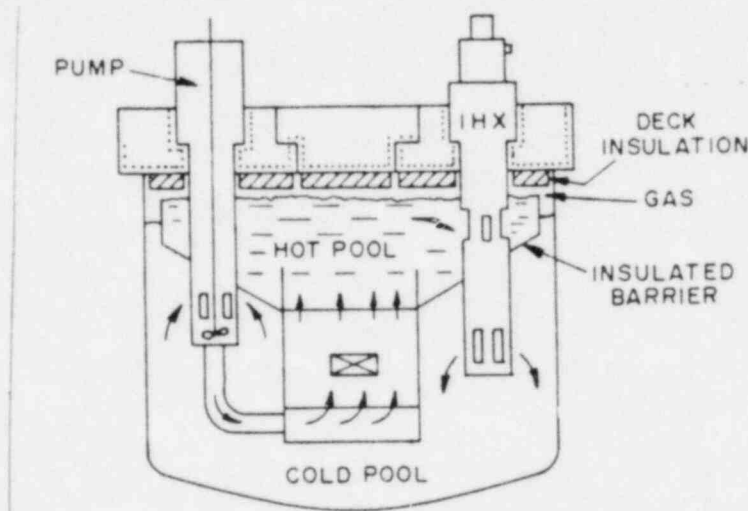
Fig. 1 Primary system configuration for a pool-type LMFBR
