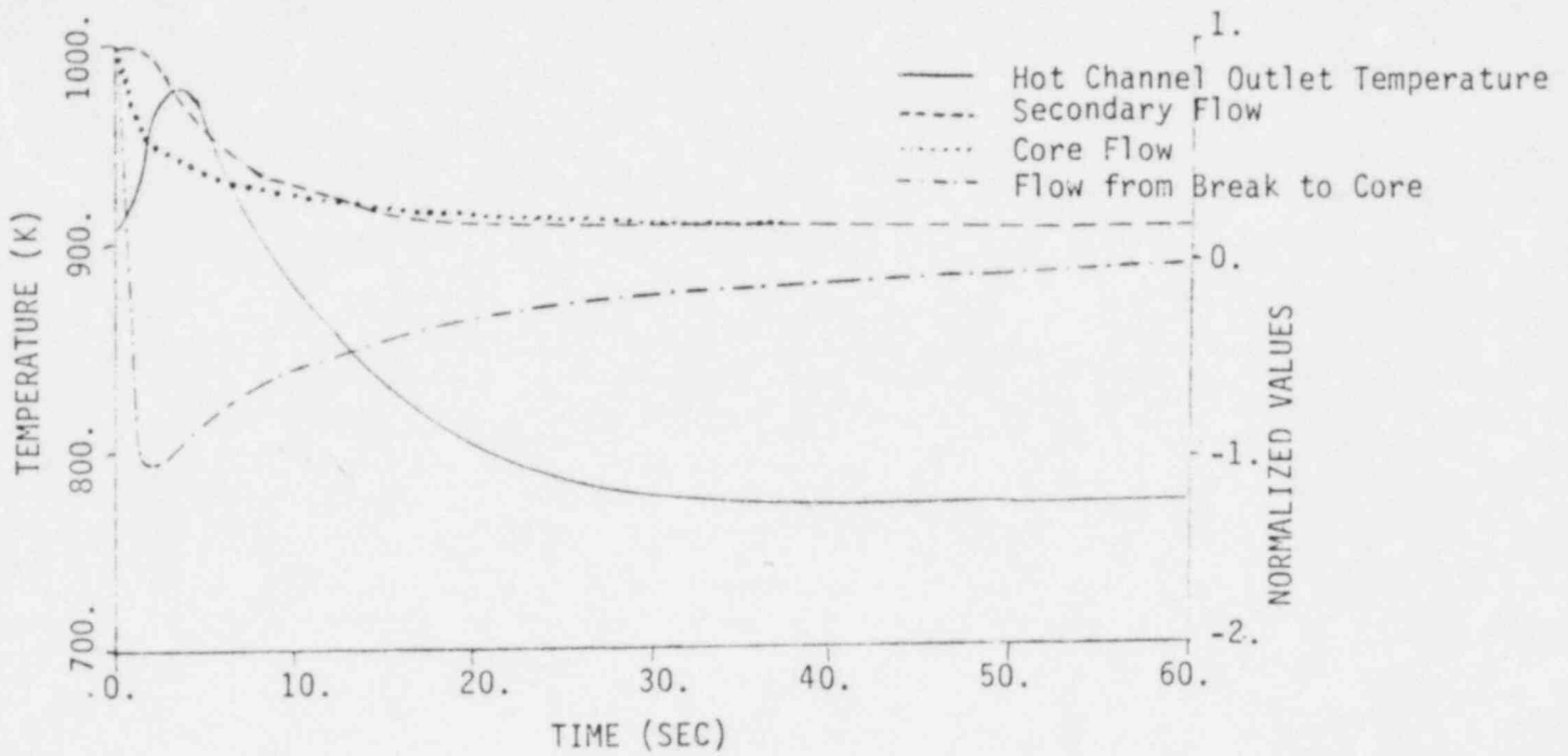
Fig. 3 - System response to a protected pipe rupture accident in a primary pump discharge line
