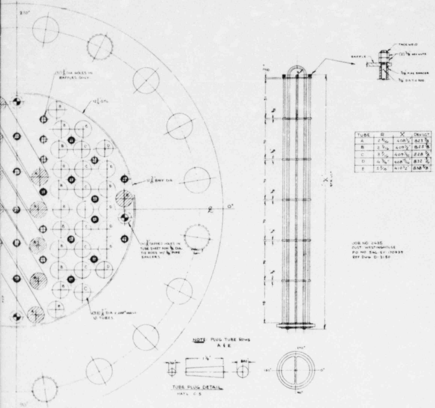
Figure 6-12. FLECHT SEASET Natural Circulation Unbroken Loop Steam Generator Construction Details (sheet 1 of 2)
