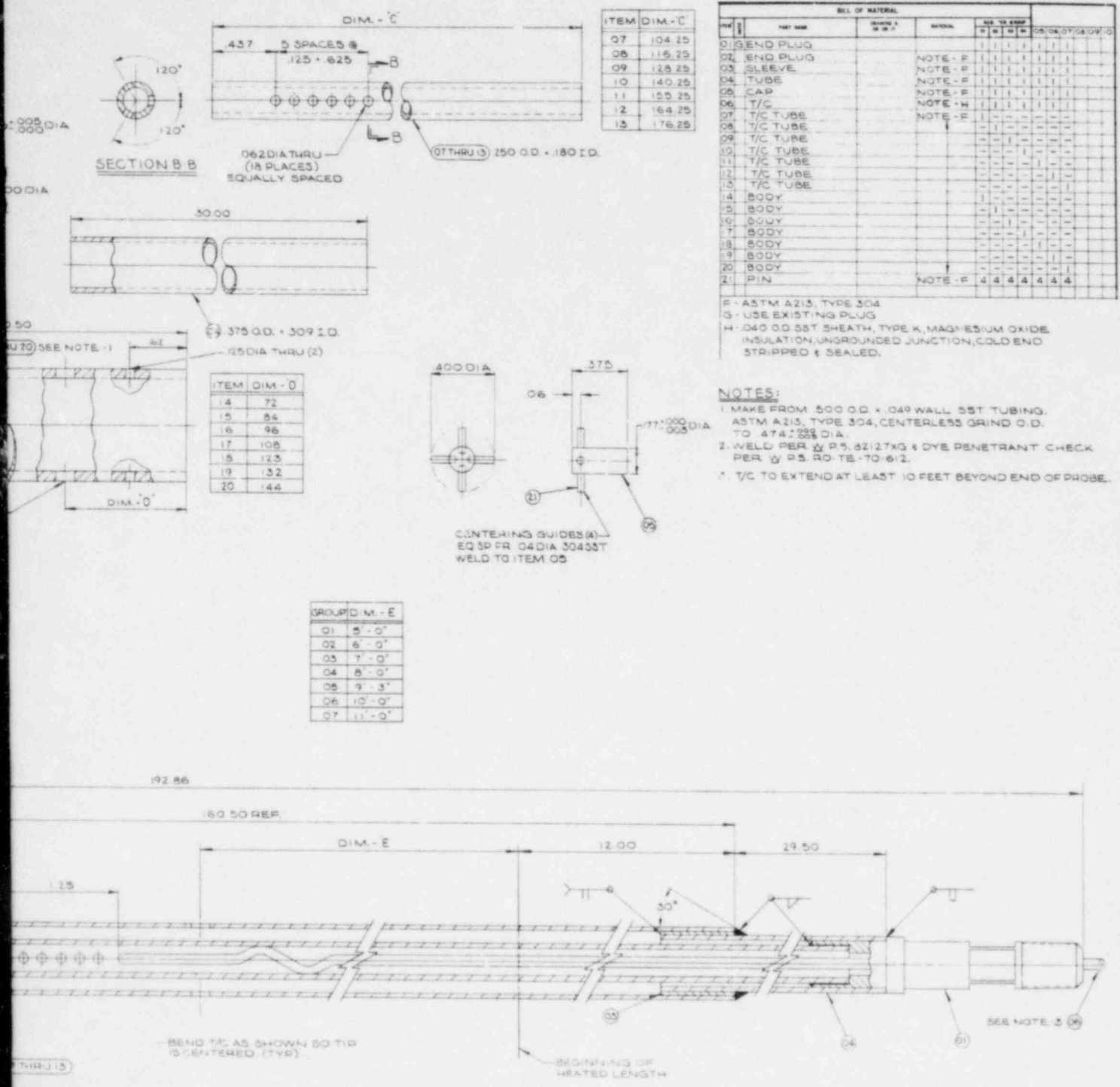
Figure 6-23. FLECHT SEASET Natural Circulation Rod Bundle Aspirating Steam Probe
