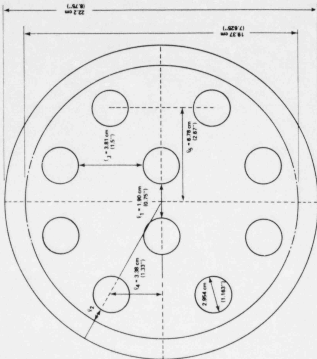
Figure D-12. Rod Arrangement
