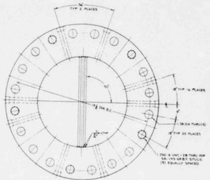
DETAIL E (MAYL 3A-285 GFC OR EQUIV) SCALE 1:1
