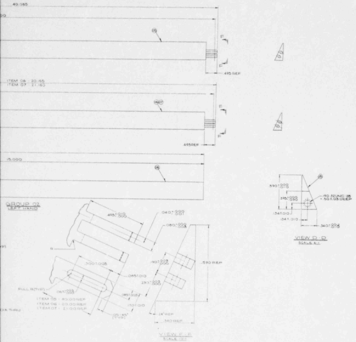
Figure E-5. FLECHT SEASET Natural Circulation Bundle Filler Details (sheet 2 of 2)
