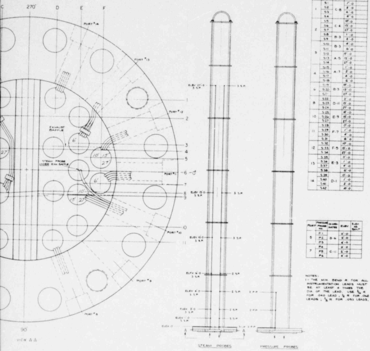
Figure 6-34. FLECHT SEASET Natural Circulation Broken Loop Steam Generator Noncondensable Gas Sampling Locations
