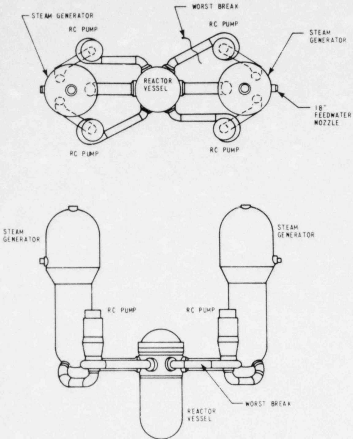
Figure 4-2. Combustion Engineering Reactor Coolant Loop Configuration and Calculated Worst Break Location (Large Cold Leg Break)
