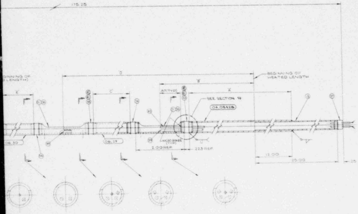
Figure 6-25. FLECHT SEASET Natural Circulation Rod Bundle Heated Thermocouple Steam Probe
