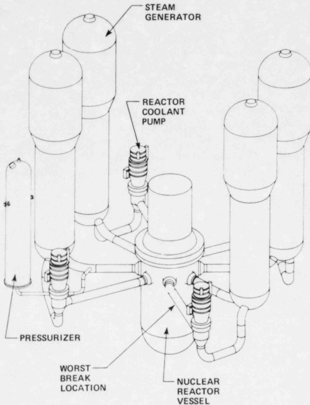
Figure 4-1. Westinghouse Reactor Coolant Loop Configuration and Calculated Worst Break Location (Large Cold Leg Break)
