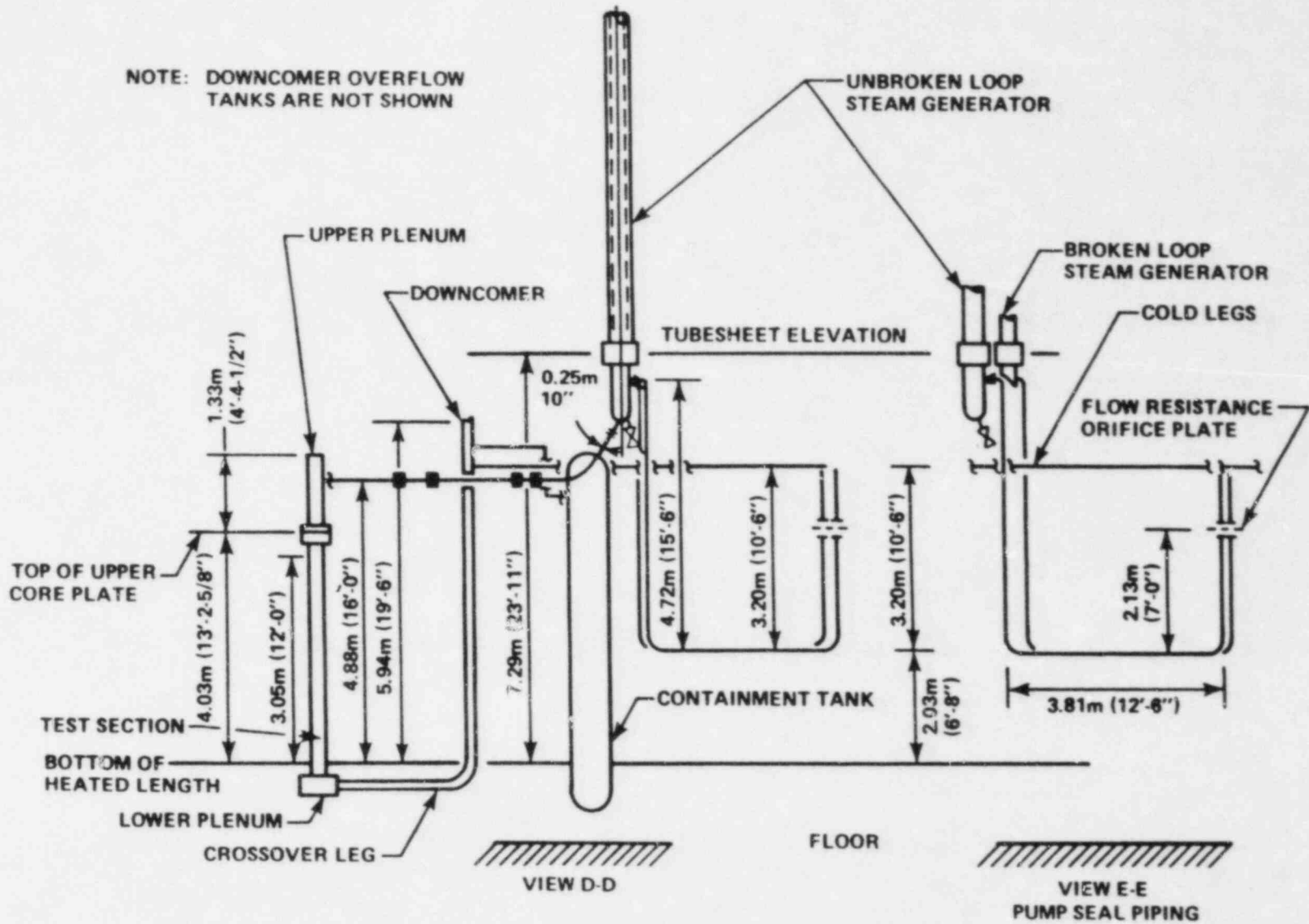
Figure B-2. FLECHT SEASET Systems Effects Test Loop Elevation View
