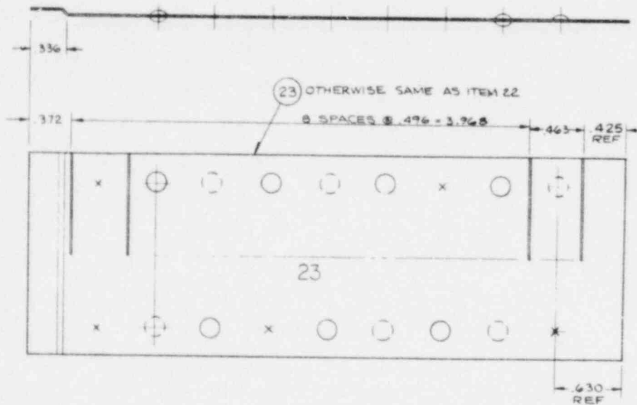
Figure E-7. FLECHT SEASET Natural Circulation Bundle Grid Details (sheet 6 of 7)
