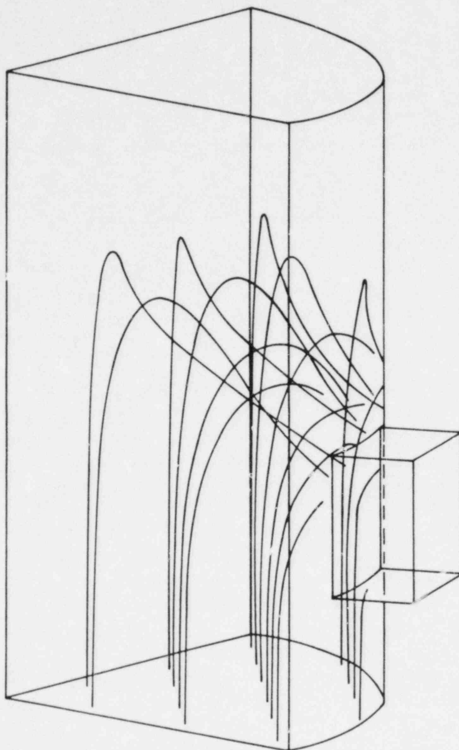
Figure D-1. Calculated Particle Trajectories in a Quadrant of Trojan Upper Plenum
