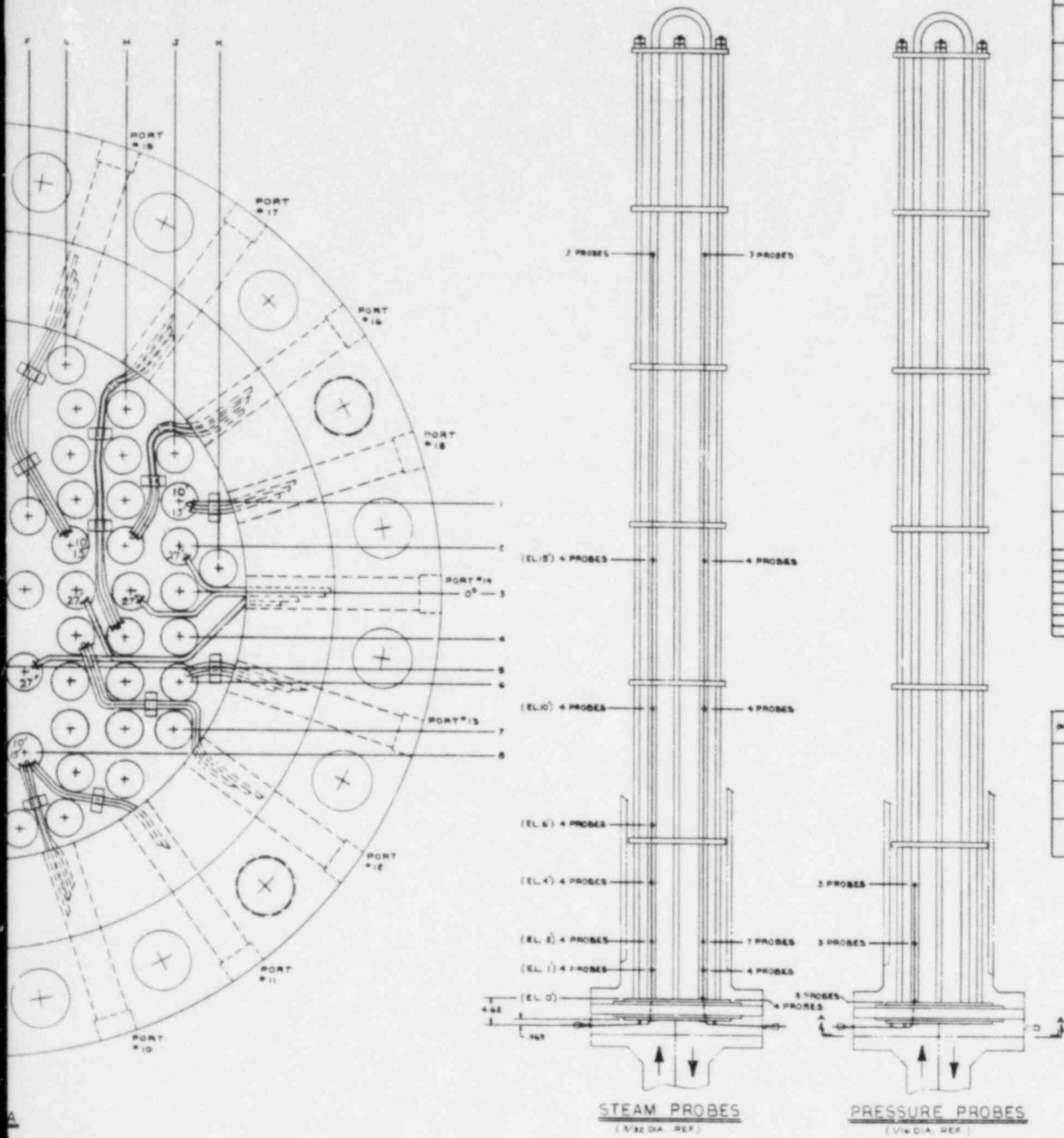
Figure 6-33. FLECHT SEASET Natural Circulation Unbroken Loop Steam Generator Noncondensable Gas Sampling Locations
