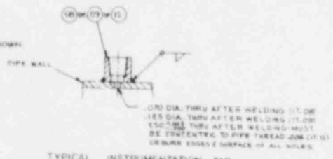
TYPICAL INSTRUMENTATION TAP
