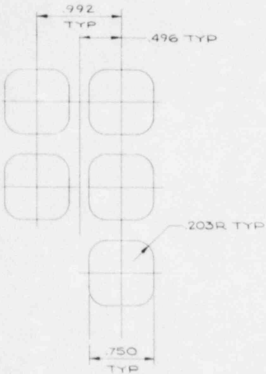
DETAIL - D (20 PLACES)
