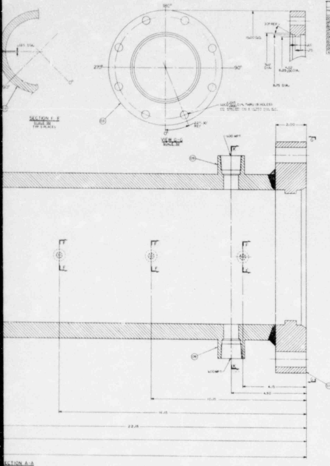
Figure 6-7. FLECHT SEASET Natural Circulation Upper Plenum (sheet 1 of 3)
