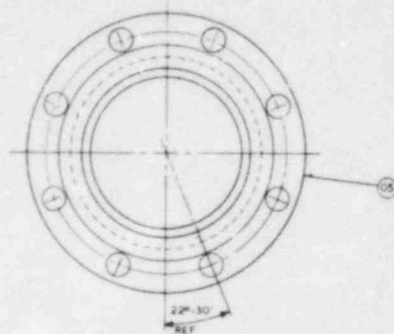
VIEW B-B SCALE 1/4"
