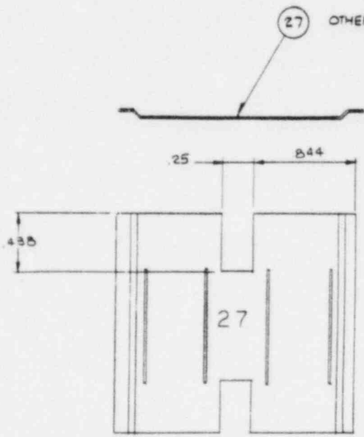
Figure E-7. FLECHT SEASET Natural Circulation Bundle Grid Details (sheet 7 of 7)
