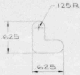
DETAIL - A (4 PLACES)
