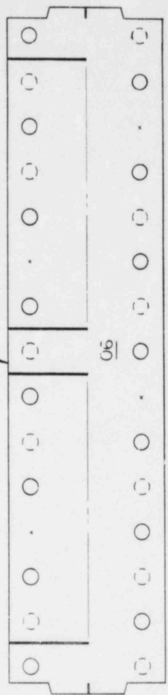
Figure E-7. FLECHT SEASET Natural Circulation Bundle Grid Details (sheet 2 of 7)
