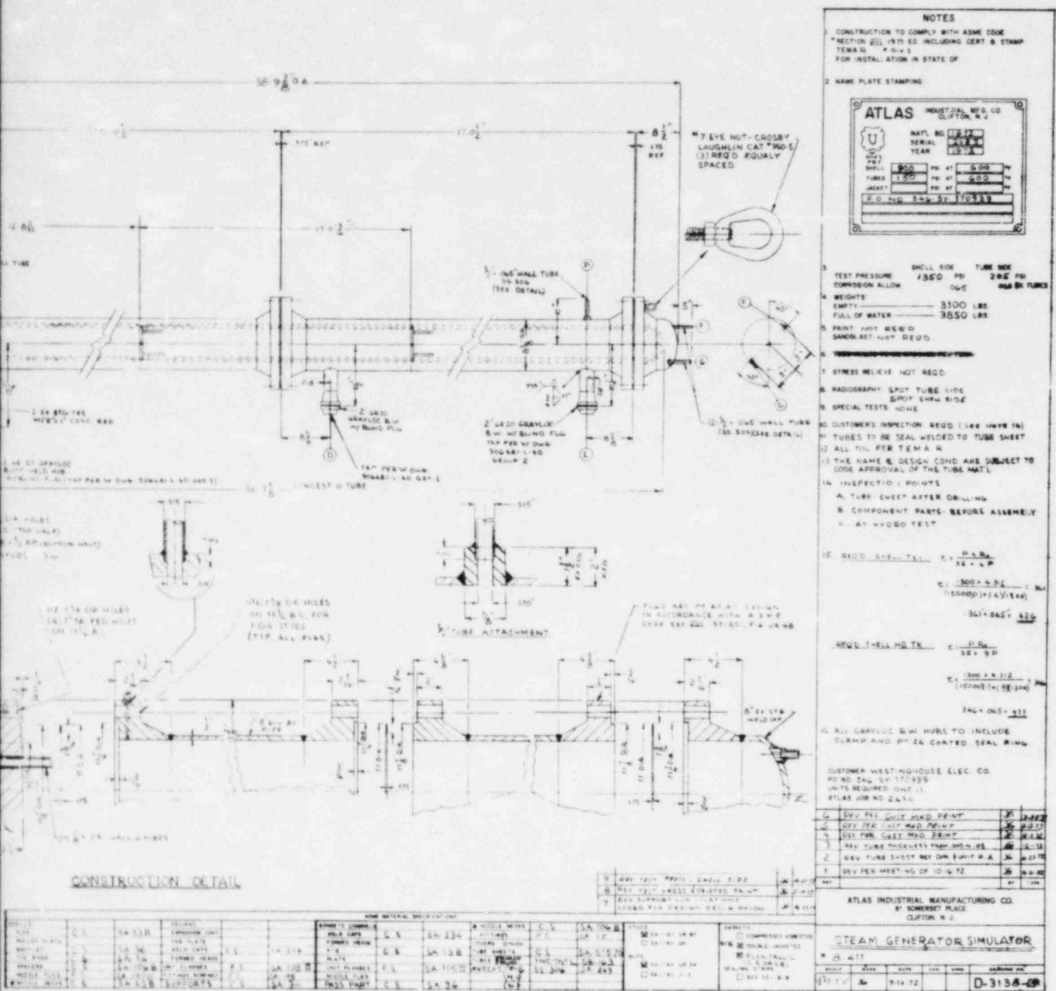
Figure 6-12. FLECHT SEASET Natural Circulation Unbroken Loop Steam Generator Construction Details (sheet 2 of 2)
