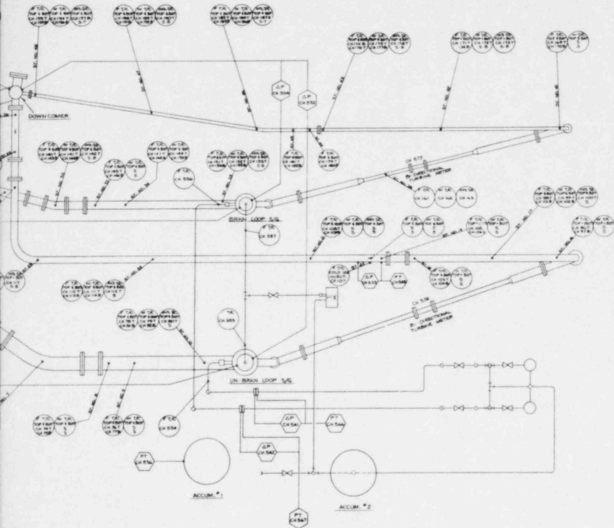
Figure 6-19. FLECHT SEASET Natural Circulation Facility Instrumentation Schematic Diagram (sheet 1 of 2)
