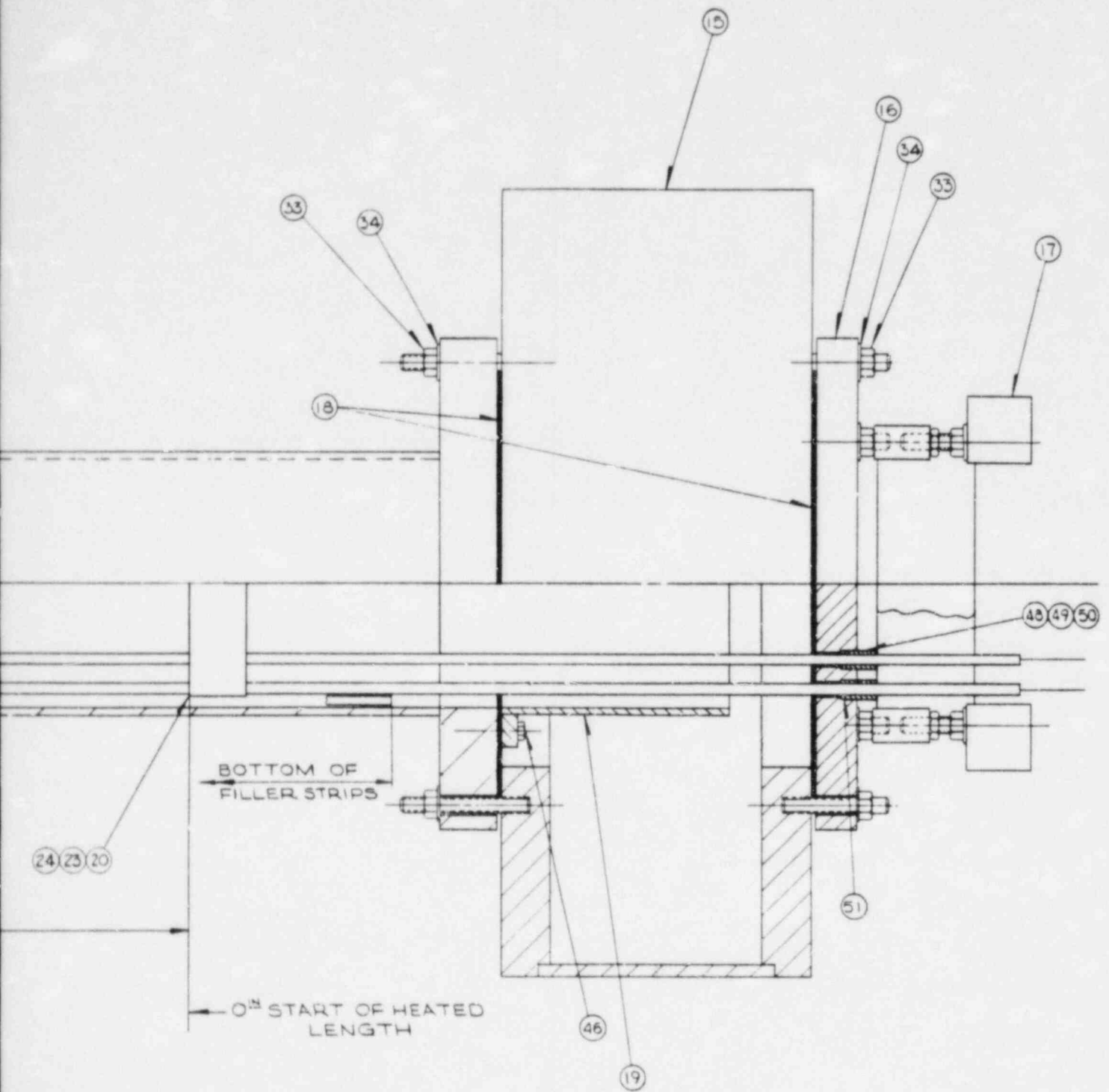
Figure 6-3. FLECHT SEASET Natural Circulation Test Section Assembly (sheet 4 of 4)
