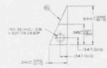
VIEW A-A SCALE 4:1
