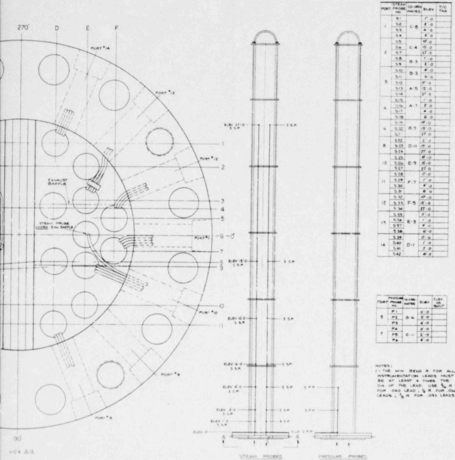
Figure 6-31. FLECHT SEASET Natural Circulation Broken Loop Steam Generator Instrumentation Steam and Pressure Probes
