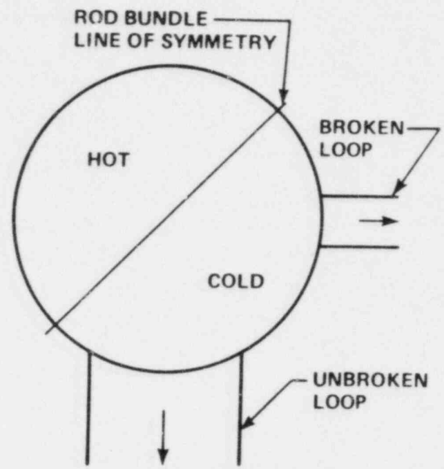
(a) SIMULATED UPPER PLENUM WITH SINGLE HOT LEG
