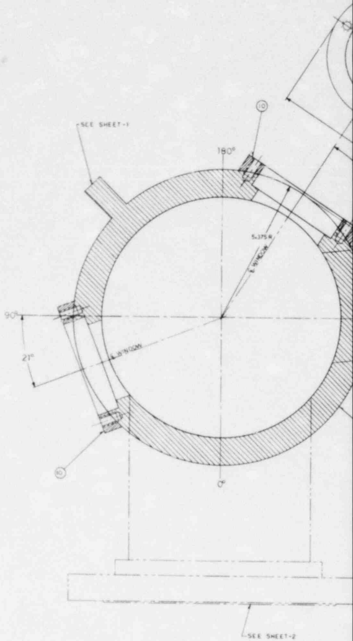
SECTION H-H AT ELEV. 17.00
