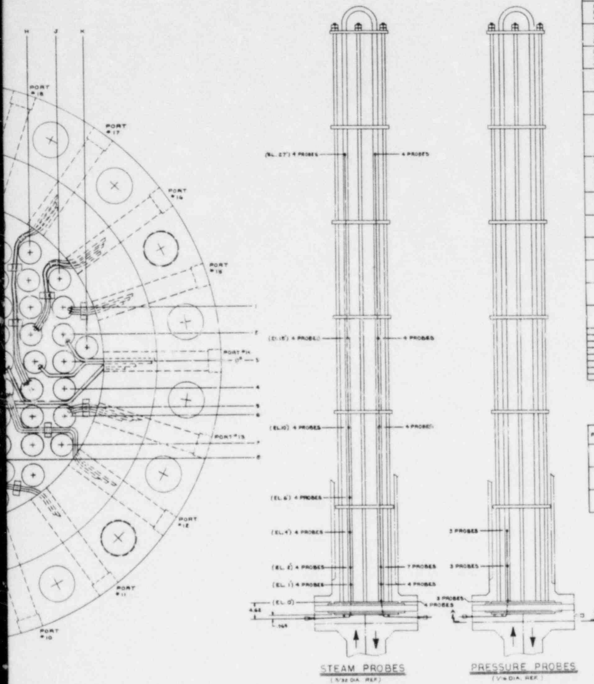
Figure 6-29. FLECHT SEASET Natural Circulation Unbroken Loop Steam Generator Instrumentation Steam and Pressure Probes
