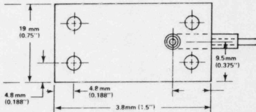
Figure 6-27. FLECHT SEASET Natural Circulation Insulation Thermocouple Support Fixture
