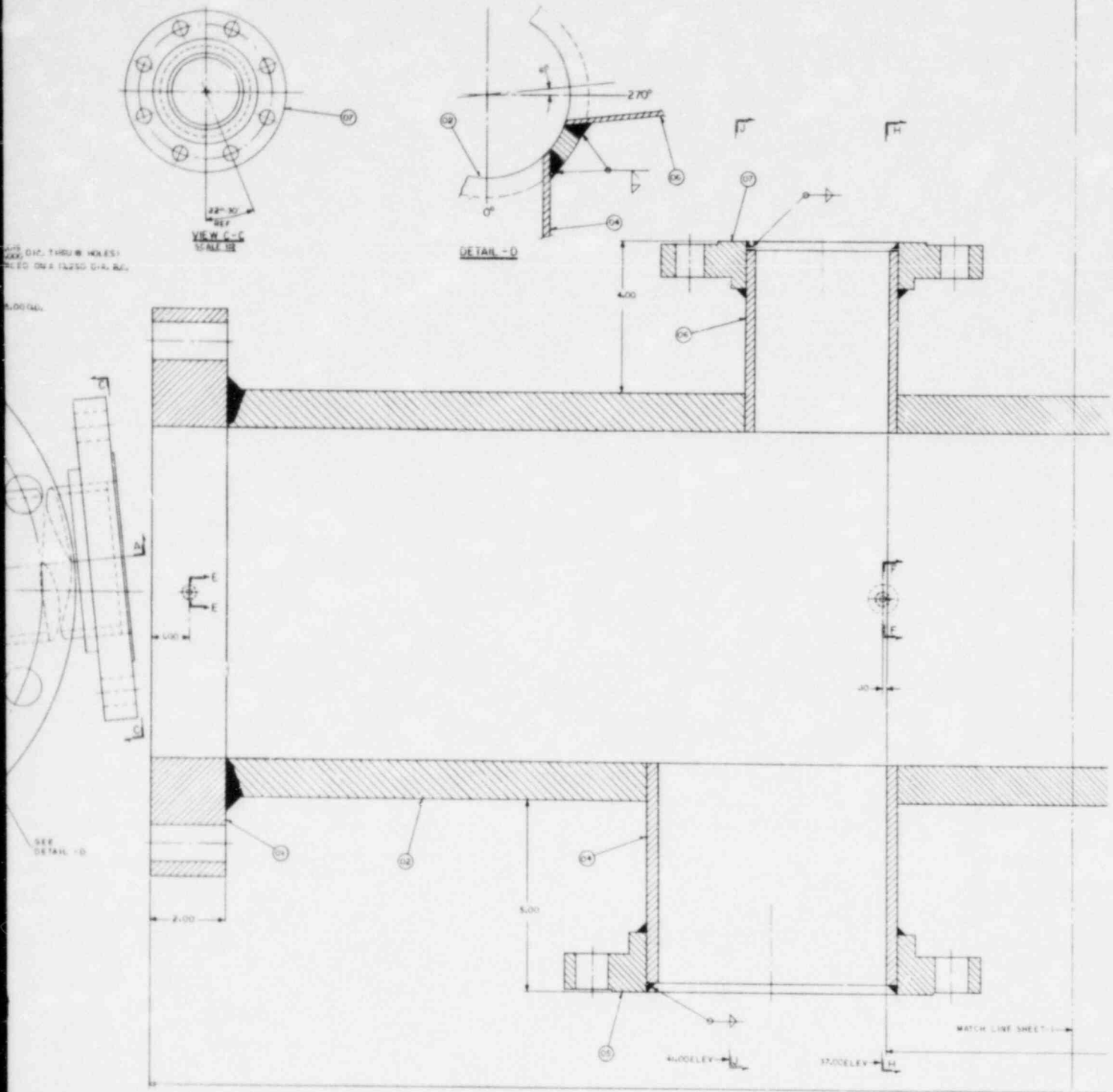
Figure 6-7. FLECHT SEASET Natural Circulation Upper Plenum (sheet 2 of 3)
