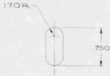
DETAIL - C (6 PLACES)
