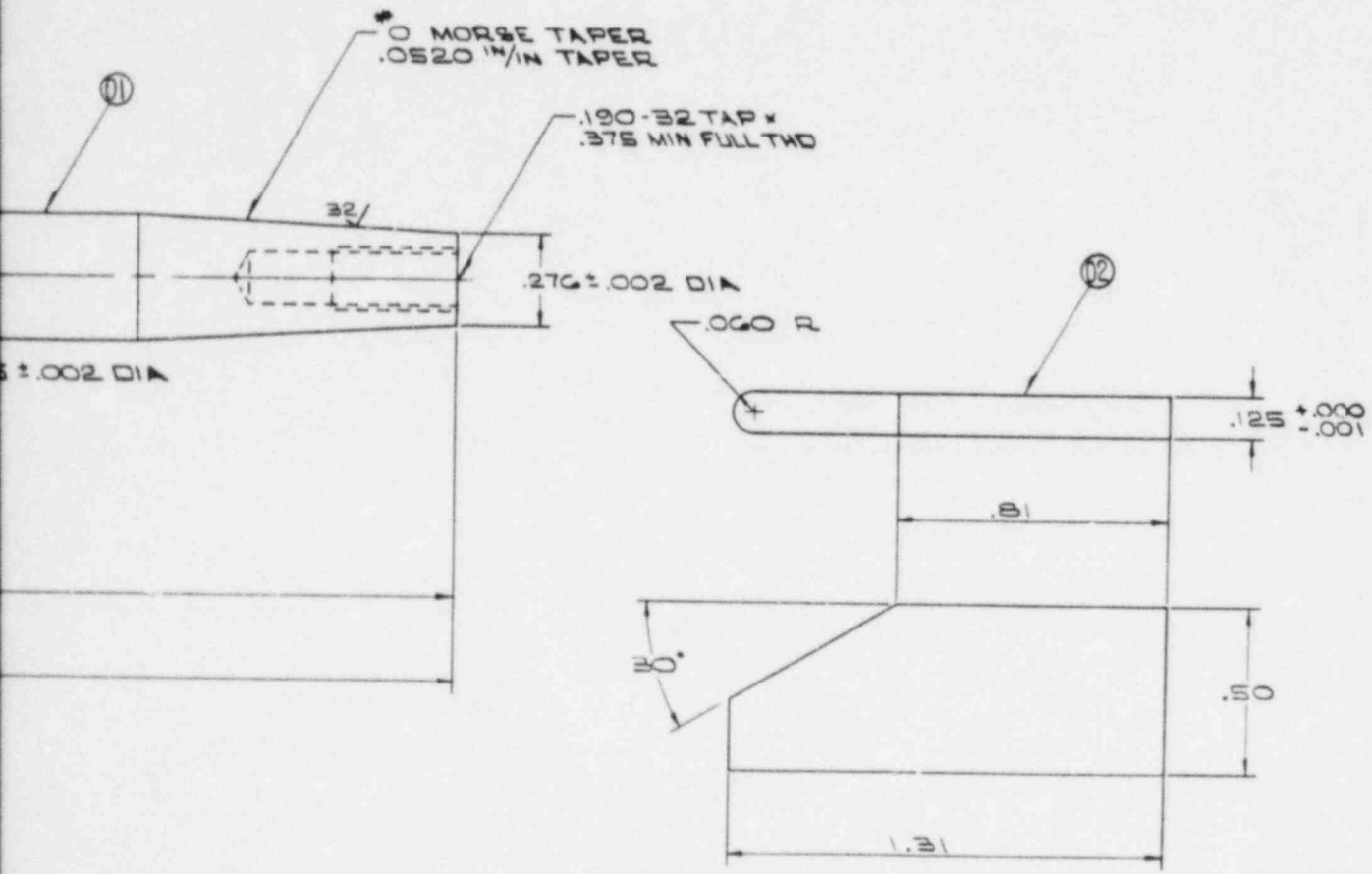
Figure E-10. FLECHT SEASET Natural Circulation Four-Heater-Rod Terminal Assembly (sheet 1 of 2)
