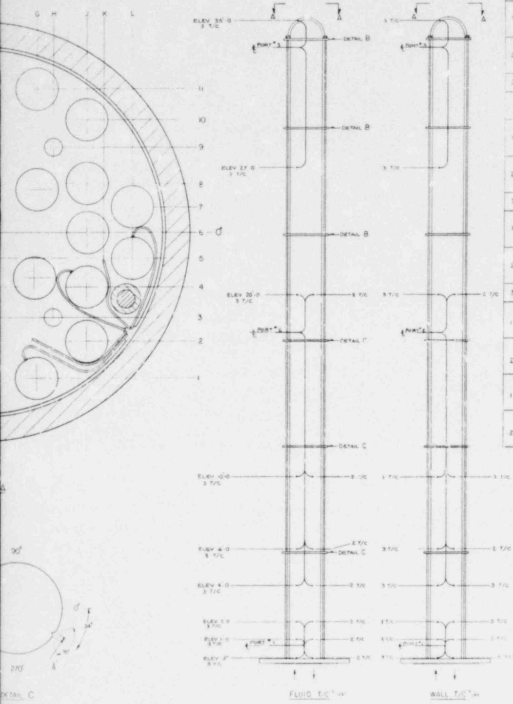
Figure 6-30. FLECHT SEASET Natural Circulation Broken Loop Steam Generator Fluid and Tube Wall Thermocouples
