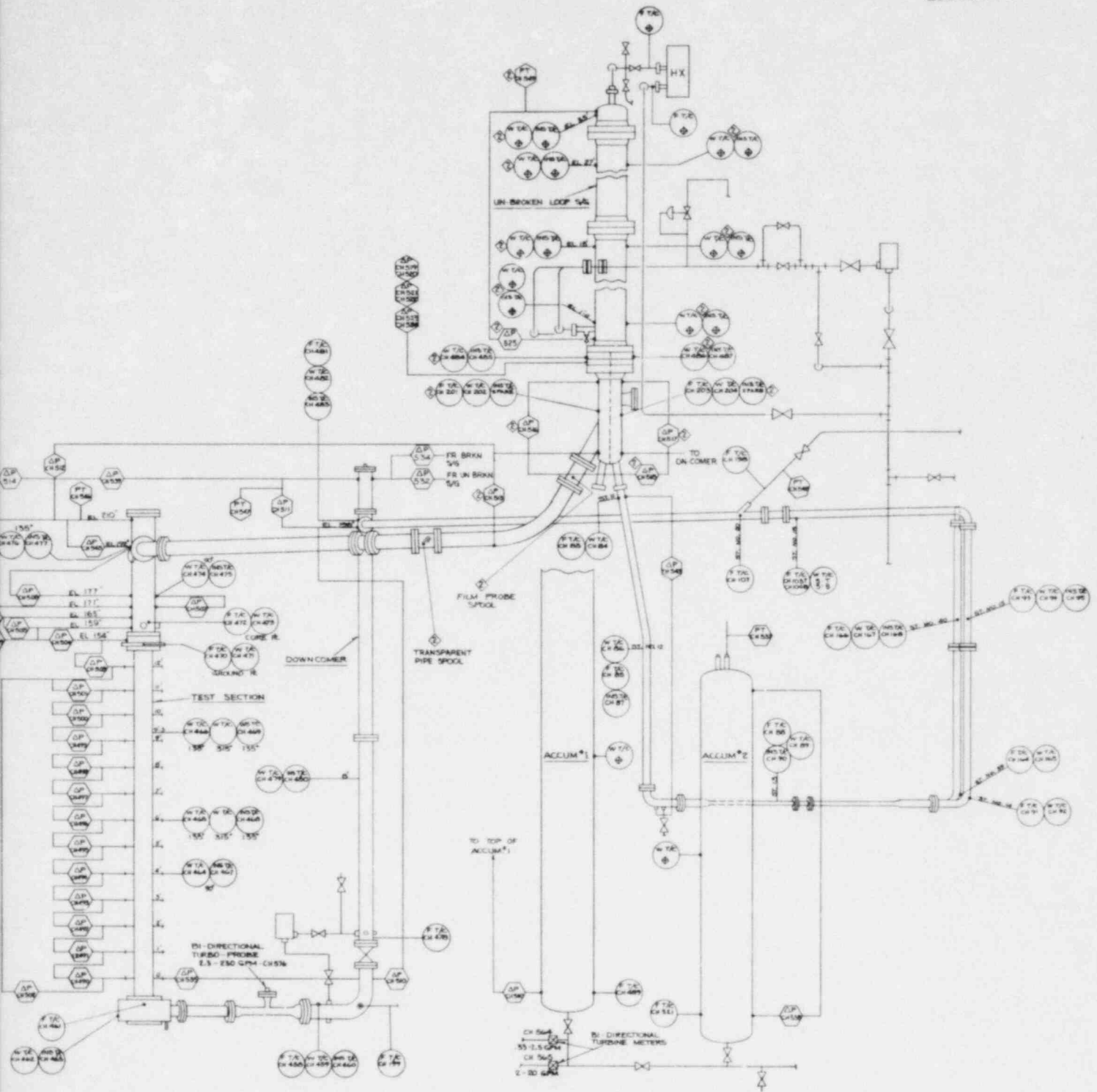
Figure 6-19. FLECHT SEASET Natural Circulation Facility Instrumentation Schematic Diagram (sheet 2 of 2)
