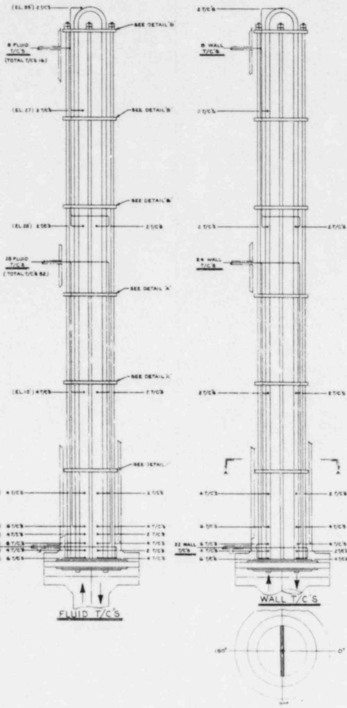
Figure 6-28. FLECHT SEASET Natural Circulation Unbroken Loop Steam Generator Instrumentation Fluid and Tube Wall Thermocouples
