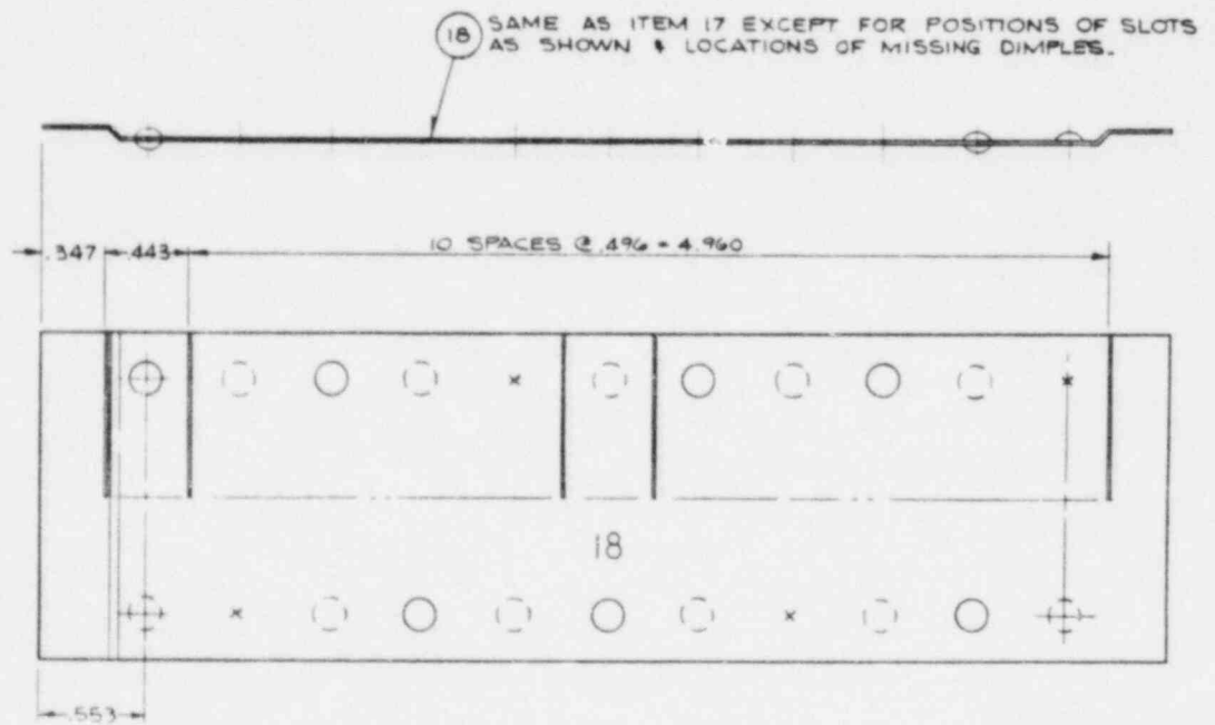
Figure E-7. FLECHT SEASET Natural Circulation Bundle Grid Details (sheet 5 of 7)
