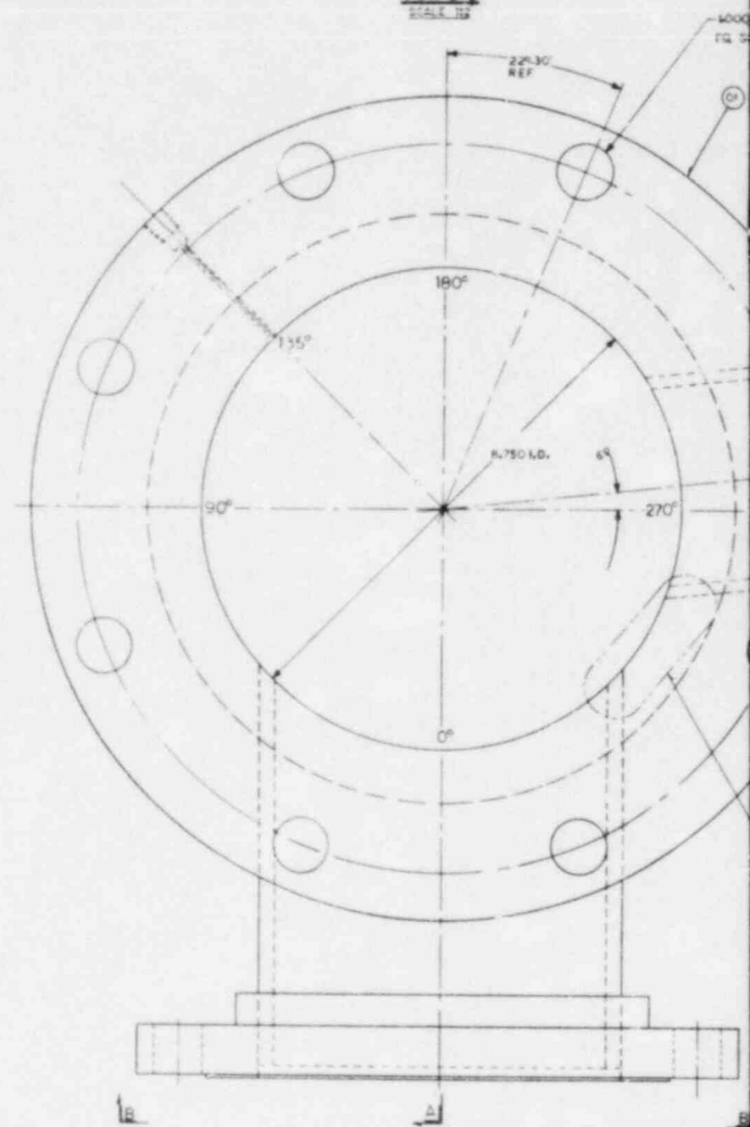
VIEW B-B SCALE 1/4"
