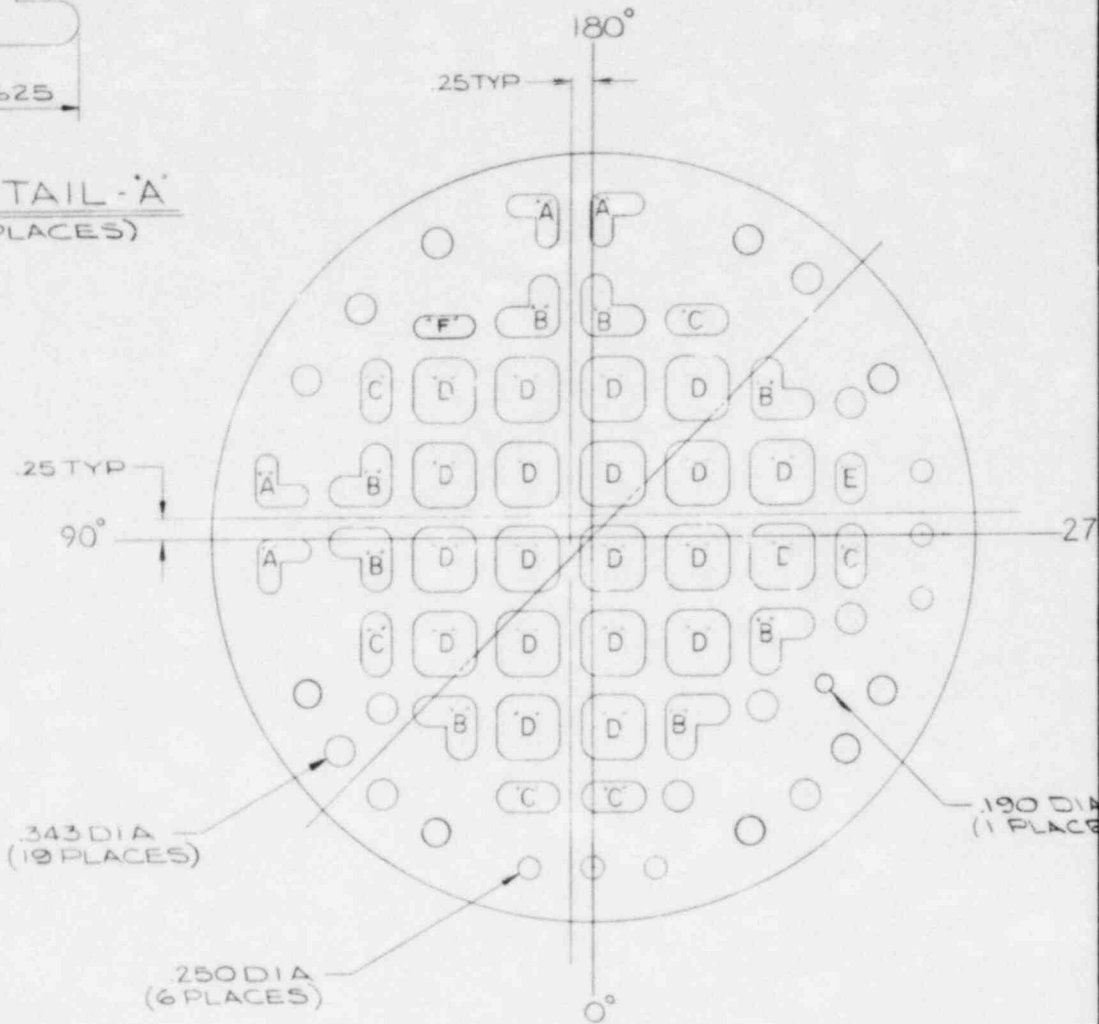
GROUND PLATE FLOW AREA 153 ELEV
