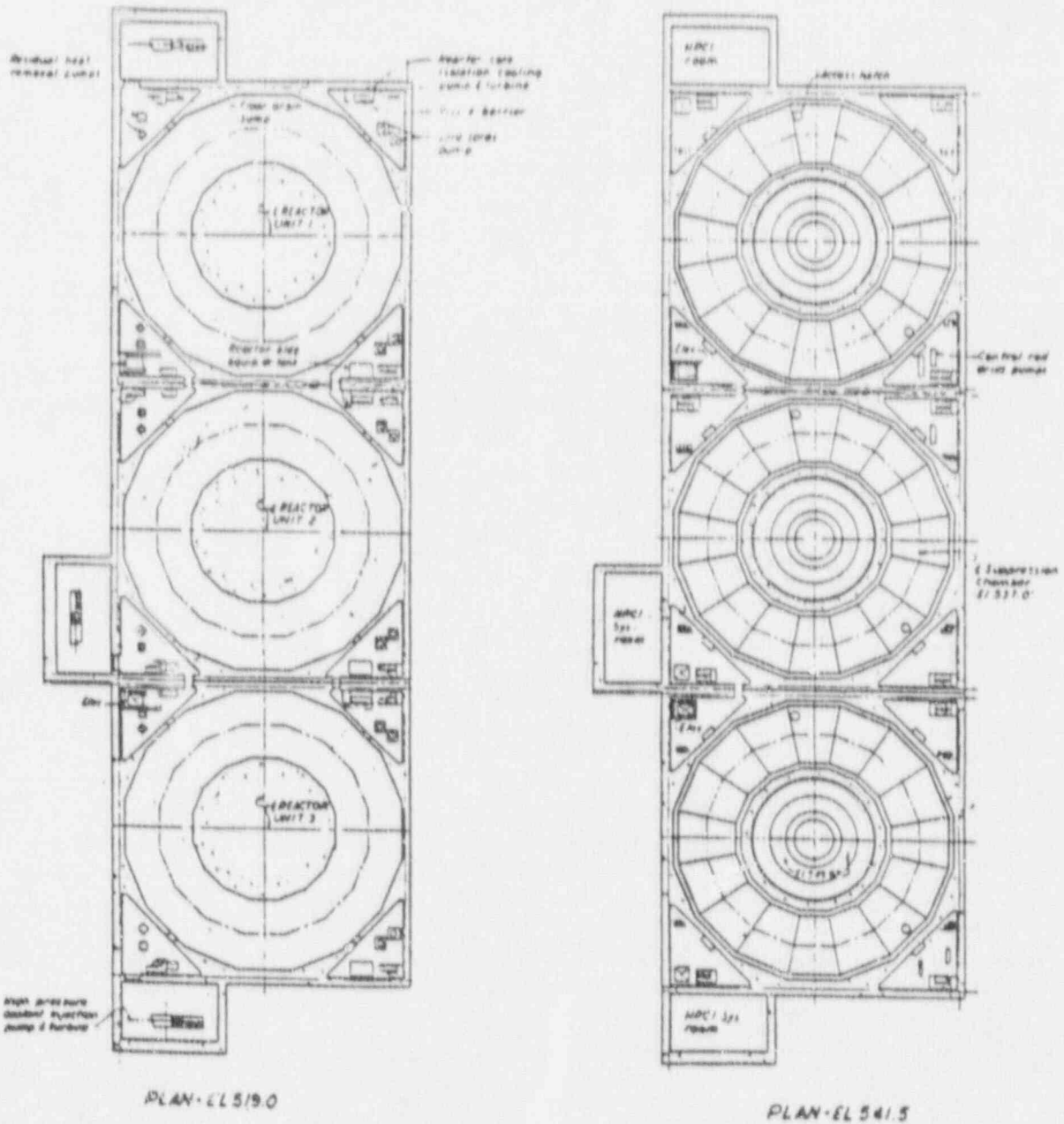
Figure 4-6. Overall Layout of the Browns Ferry Nuclear Plant, Elevations 519 ft. and 541.5 ft.
