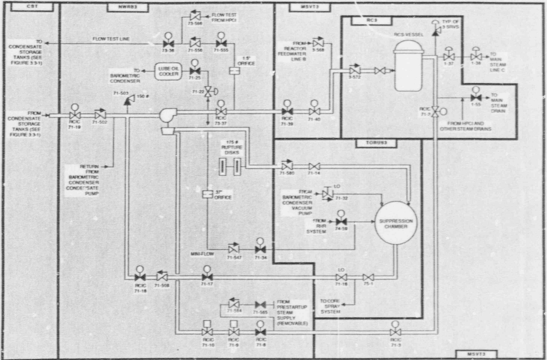
Figure 3.2-2. Browns Ferry 3 Reactor Core Isolation Cooling (RCIC) System Showing Component Locations
