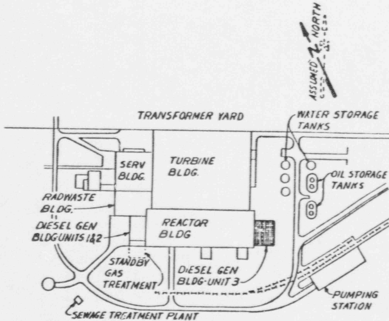
Figure 4-2. General Arrangement of Major Buildings at the Browns Ferry Site
