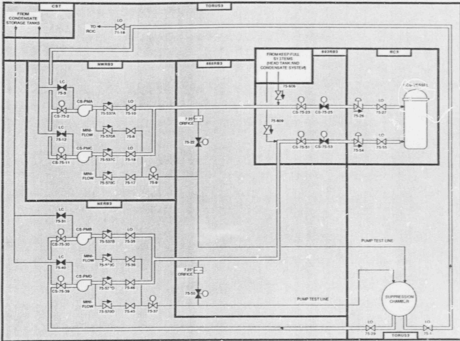
Figure 3.3-7. Browns Ferry 3 Core Spray System (CSS) Showing Component Locations
