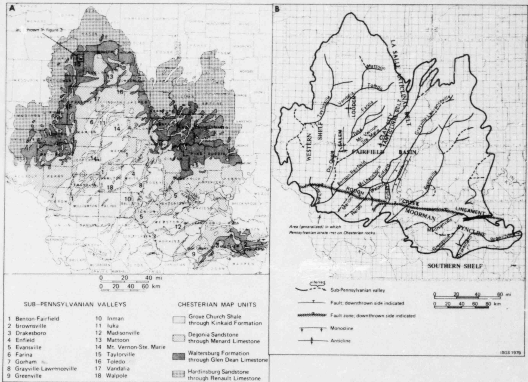
Figure 16. (A) Paleogeographic map of the sub-Pennsylvanian Chesterian surface in the Illinois Basin. (B) Relationship of sub-Pennsylvanian valleys to tectonic features of the Illinois Basin. (A) and (B) from Howard, 1979.
