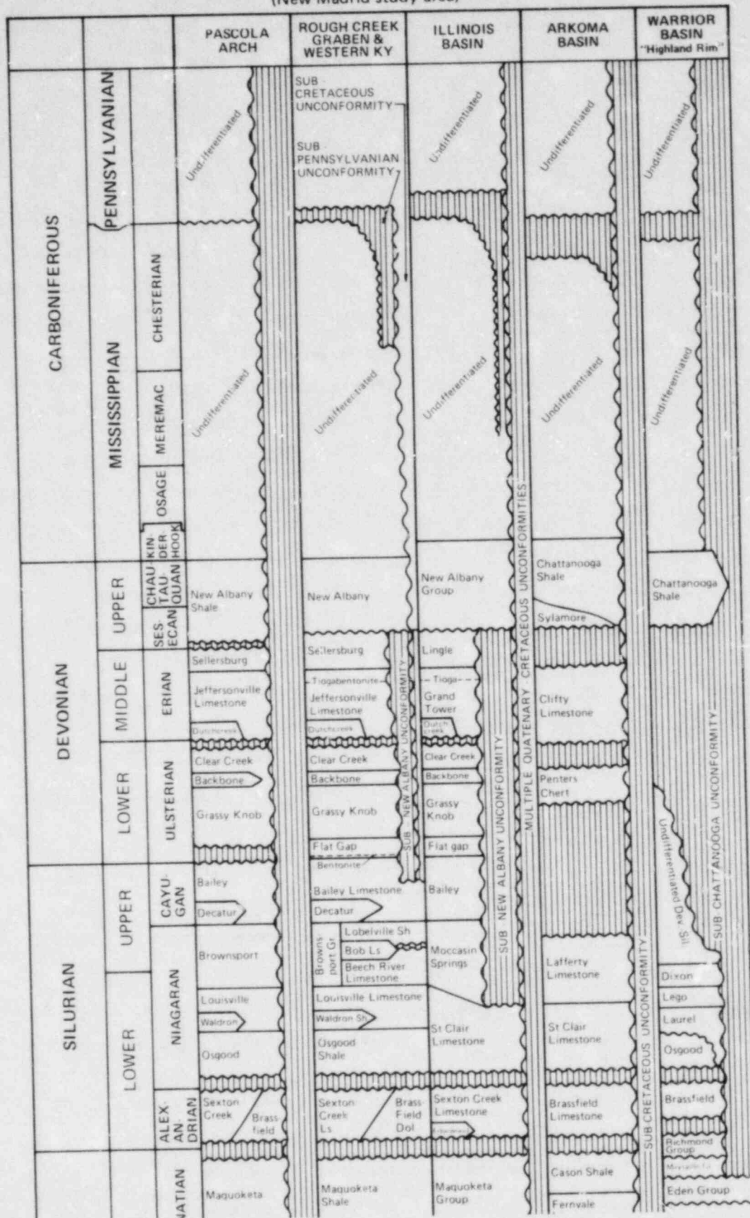
Figure 2. Geologic columns of study area.
