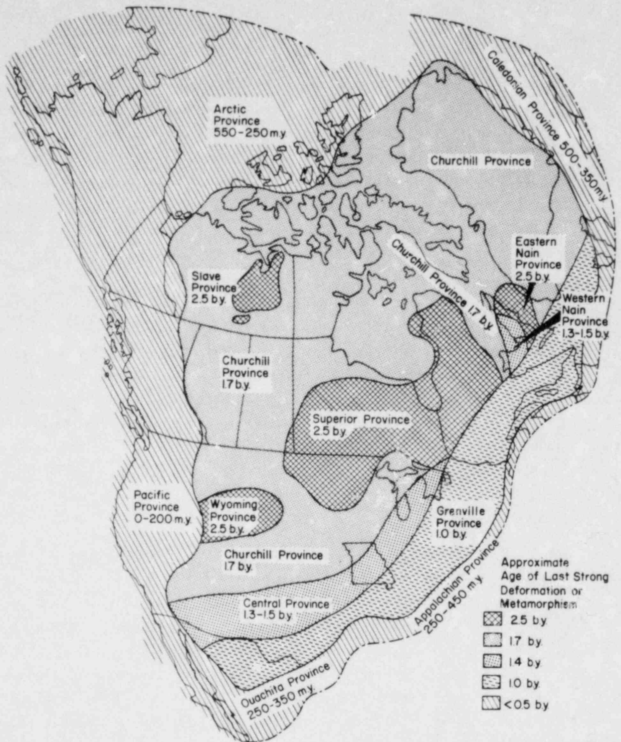
Figure 17. Tectonic provinces of Ancestral North America (from Seyfert and Sirkin, 1973; modified slightly by G. Kisvarsanyi, 1976).
