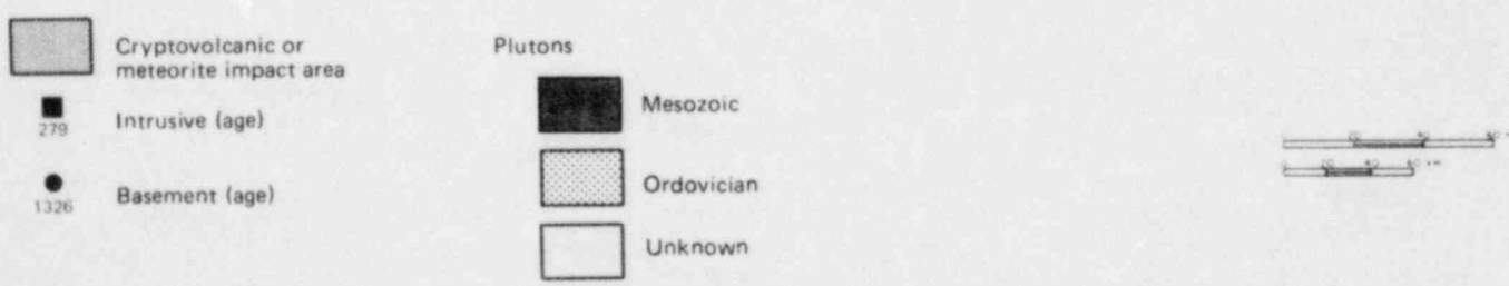
Figure 23. Locations of sampled intrusive rocks, interpreted plutons, and explosion structures. Radiometric dating shown where available.
