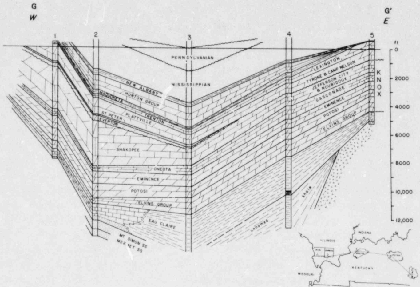
Figure 21. Cross section G-G'. Union County, Illinois, to Met... County, Kentucky.
