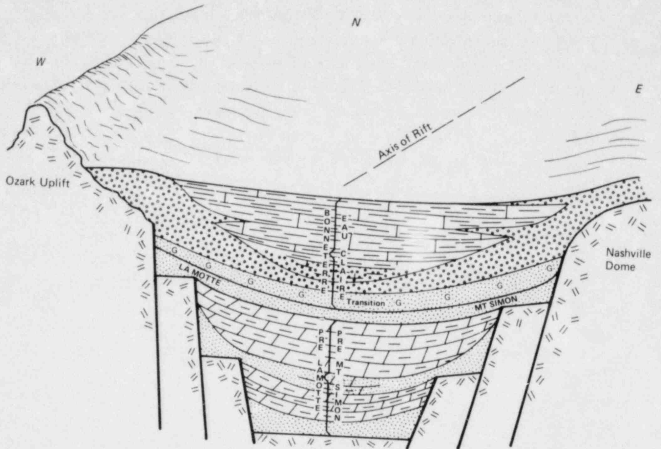
Figure 9. Schematic cross section showing interpreted growth faulting in the Rough Creek Graben.
