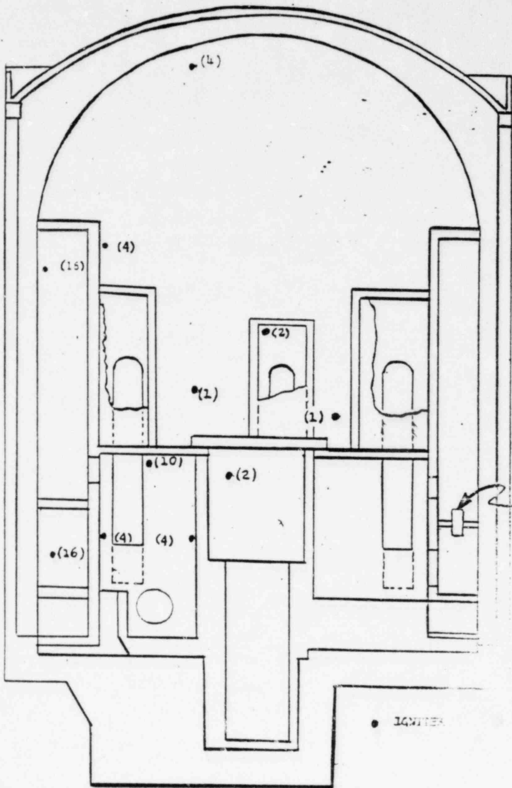
ICE CONDENSER CONTAINMENT ELEVATION VIEW SHOWING RELATIVE PHIS IGNITER LOCATIONS
