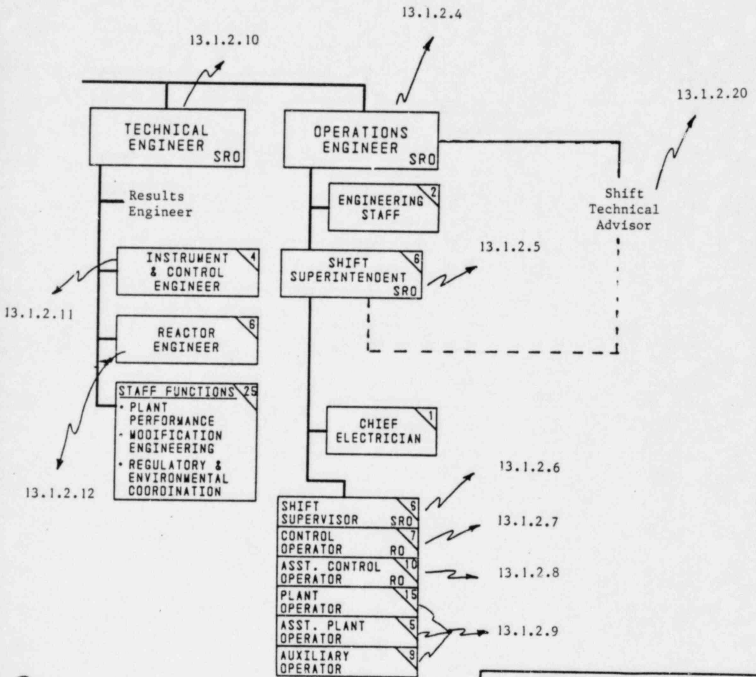
LIMERICK GENERATING STATION UNITS 1 AND 2 FINAL SAFETY ANALYSIS REPORT LIMERICK GENERATING STATION ORGANIZATION FIGURE 13.1-2
