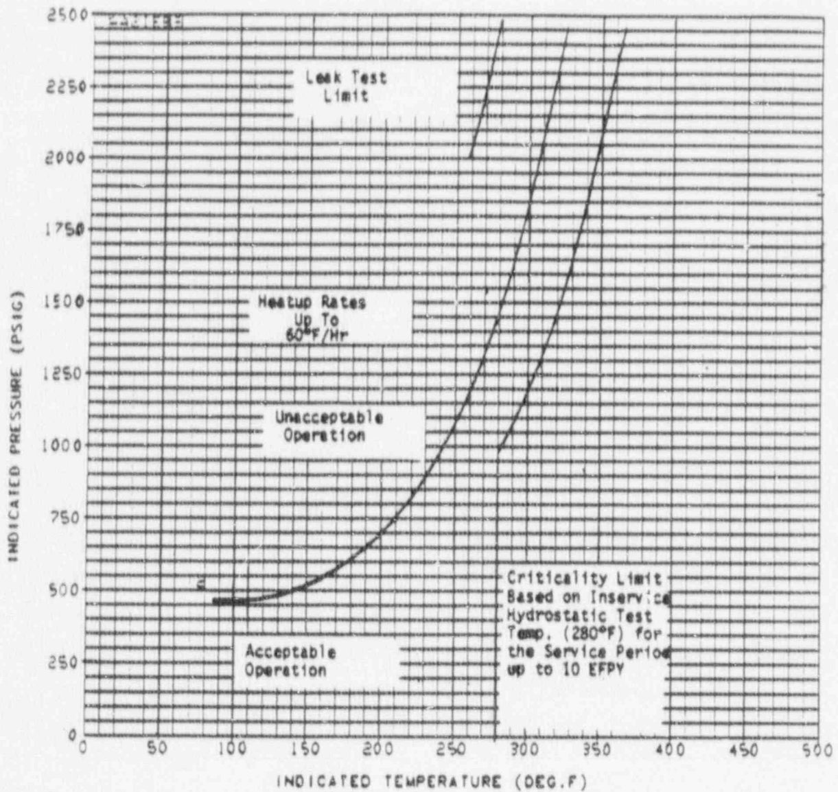
FIGURE 3.4-2 BEAVER VALLEY UNIT 2 REACTOR COOLANT SYSTEM HEATUP LIMITATIONS APPLICABLE FOR THE FIRST 10 EPFY
