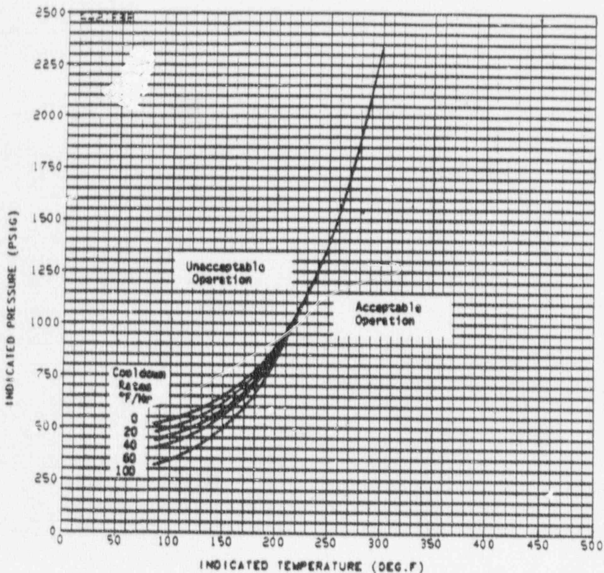
FIGURE 3.4-3 BEAVER VALLEY UNIT NO. 2 REACTOR COOLANT SYSTEM COOLDOWN LIMITATIONS APPLICABLE FOR THE FIRST 10 EPY
