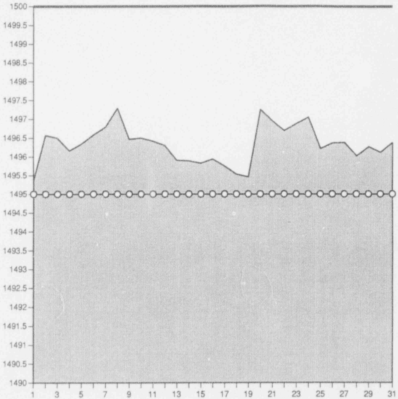
DAILY THERMAL OUTPUT
