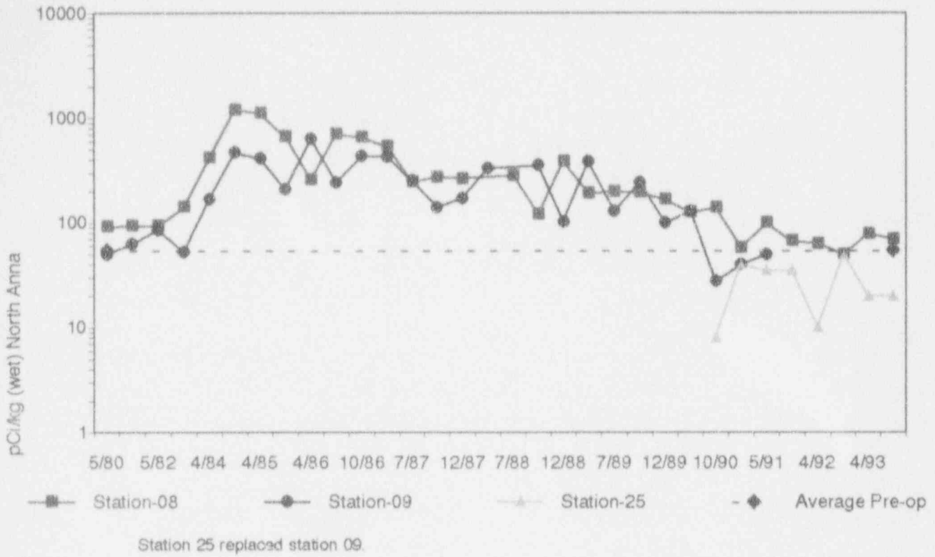
TRENDING GRAPH - 9: CESIUM-137 IN FISH
