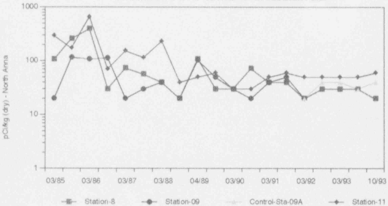
TRENDING GRAPH - 6: CESIUM-134 IN SEDIMENT SILT
