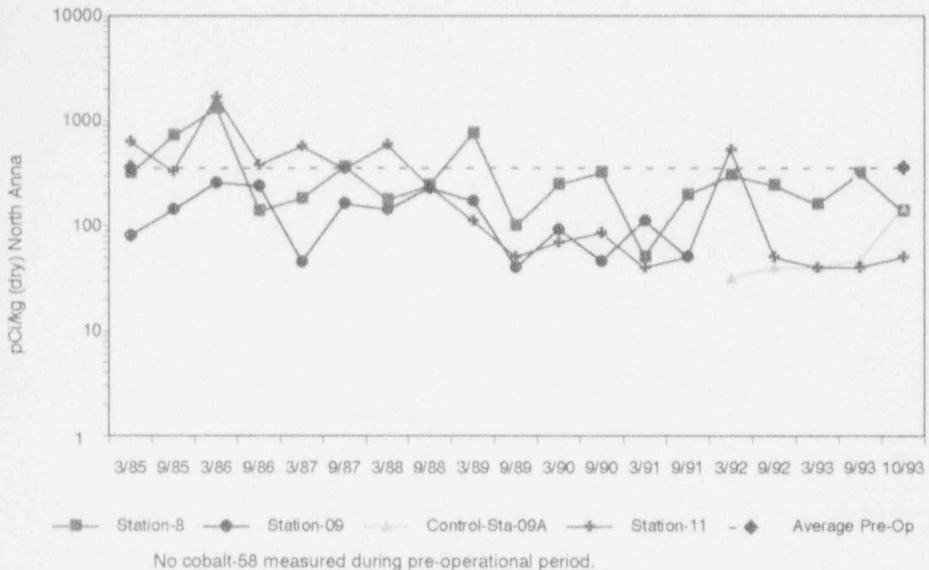
TRENDING GRAPH - 7: CESIUM-137 IN SEDIMENT SILT
