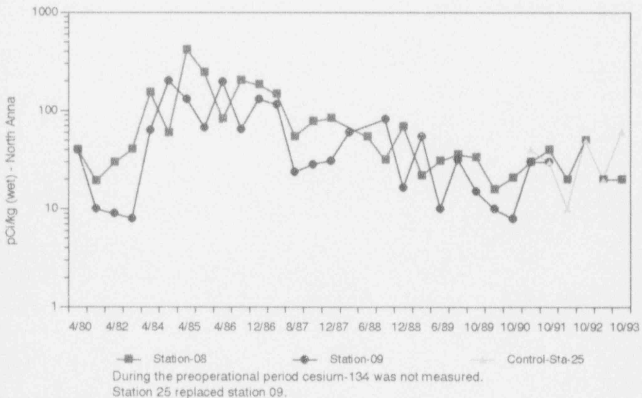
TRENDING GRAPH - 8: CESIUM-134 IN FISH
