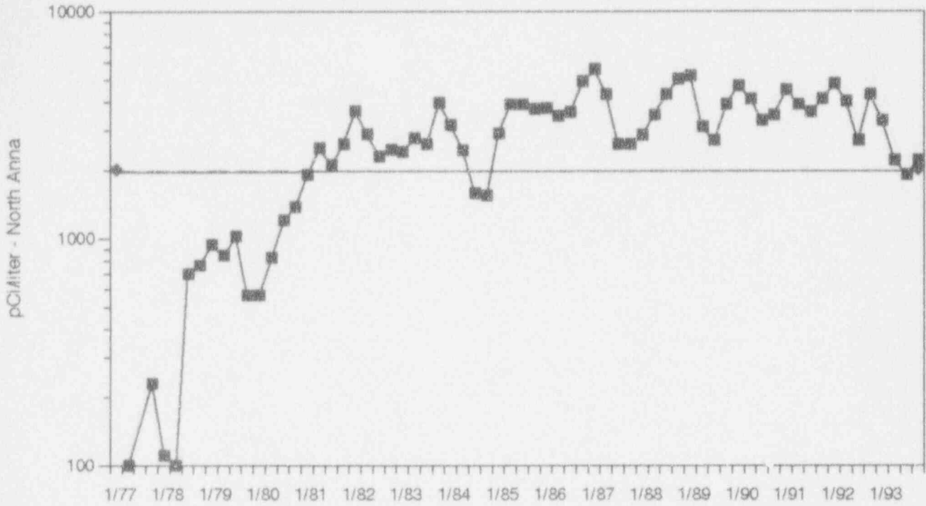
TRENDING GRAPH - 3: TRITIUM IN SURFACE WATER - STA 08
