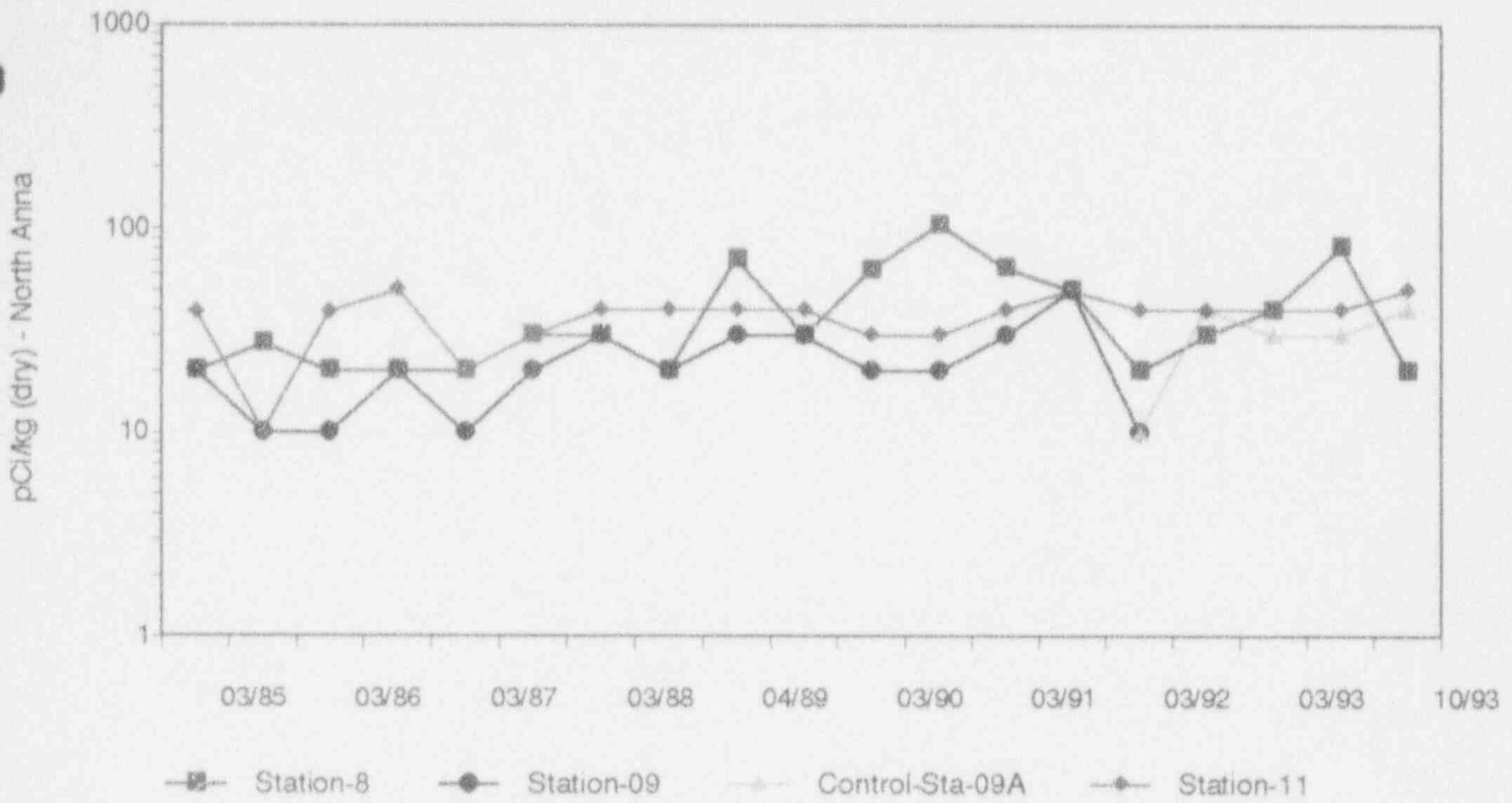
TRENDING GRAPH - 5: COBALT-60 IN SEDIMENT SILT
