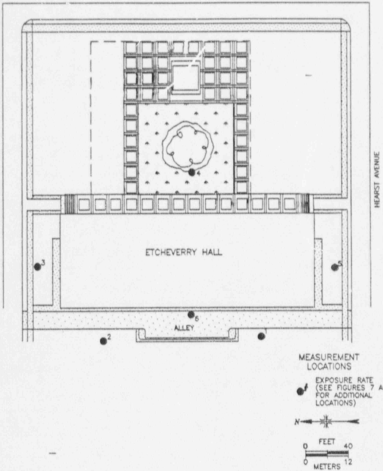
FIGURE 8: UC Berkeley—Etcheverry Hall Showing Exposure Rate Measurement Locations
