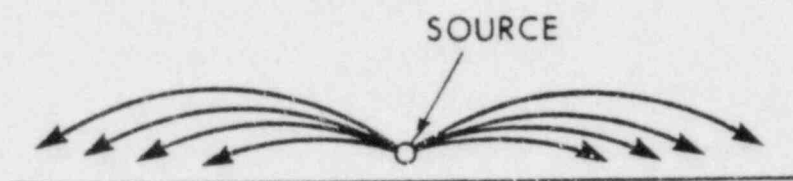
b. TEMPERATURE INCREASING WITH HEIGHT Typical Nighttime
