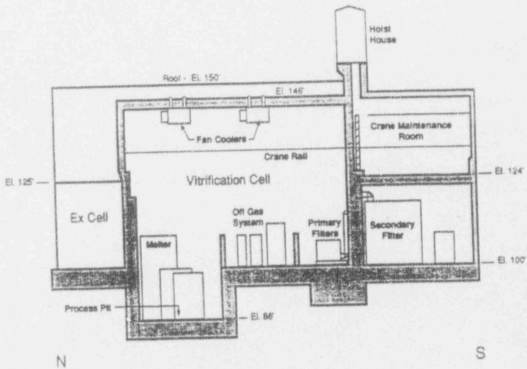
Vitrification Facility N-S Section
