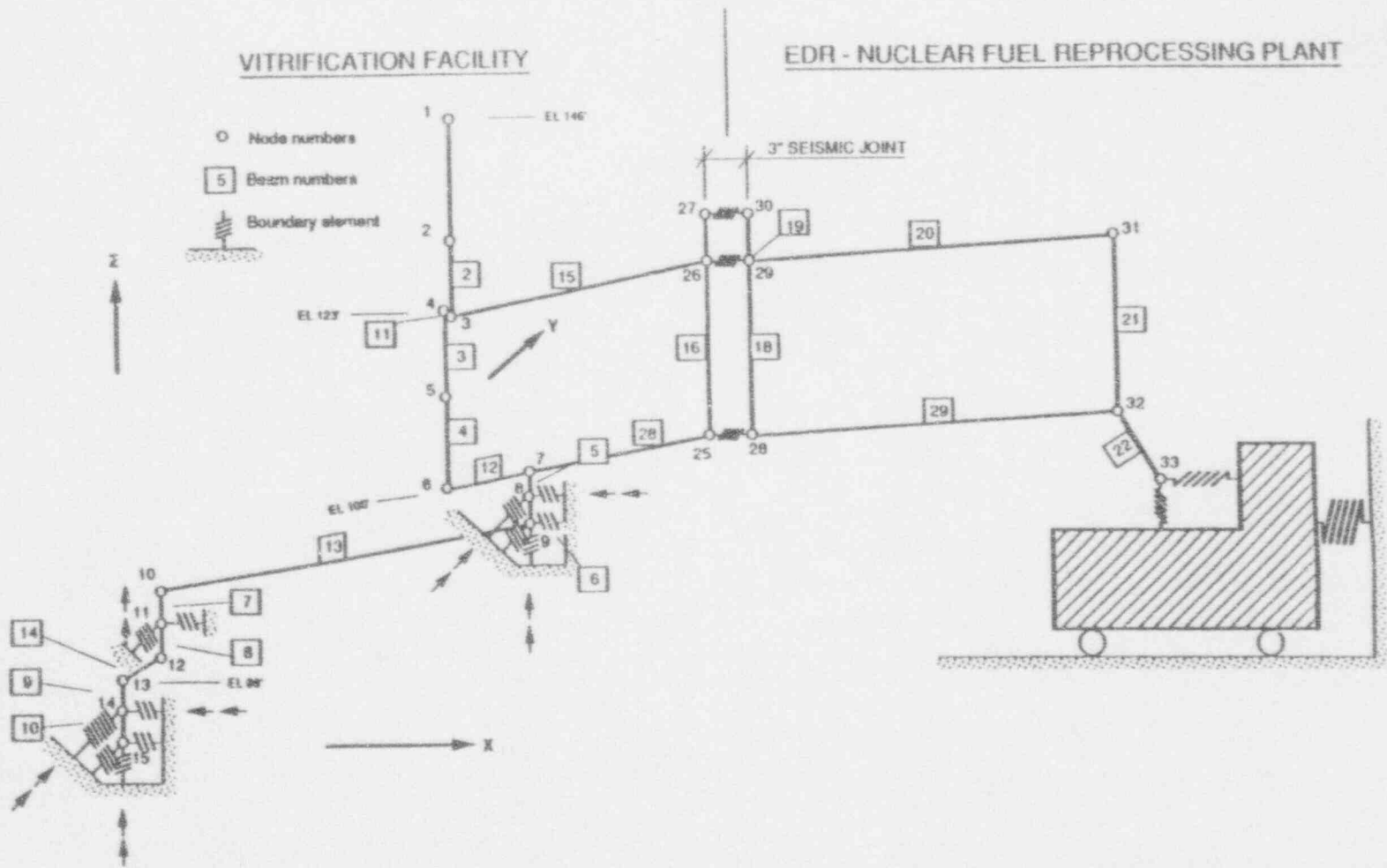
Figure 3-5. Coupled VF/EDR stick model used by Dames & Moore (Gates, 1993)
