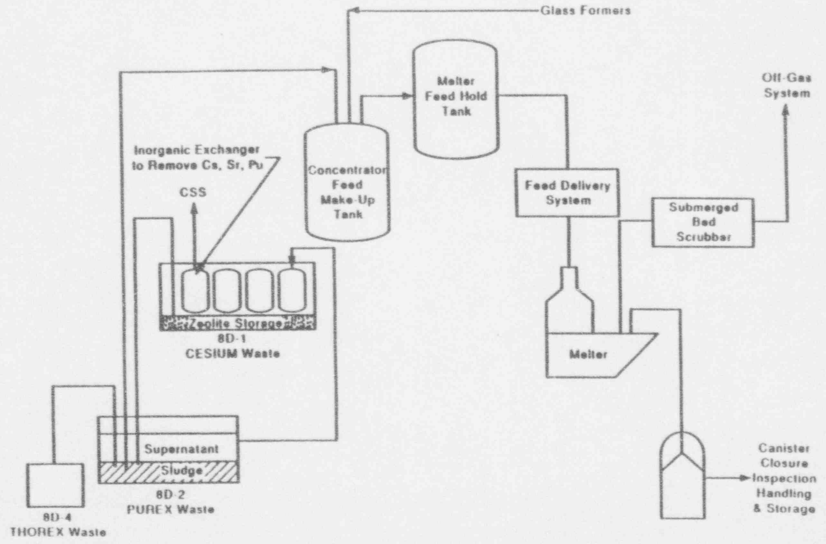
Figure 1-1. High-level waste processing flow diagram (Tschoepe et al., 1991)
