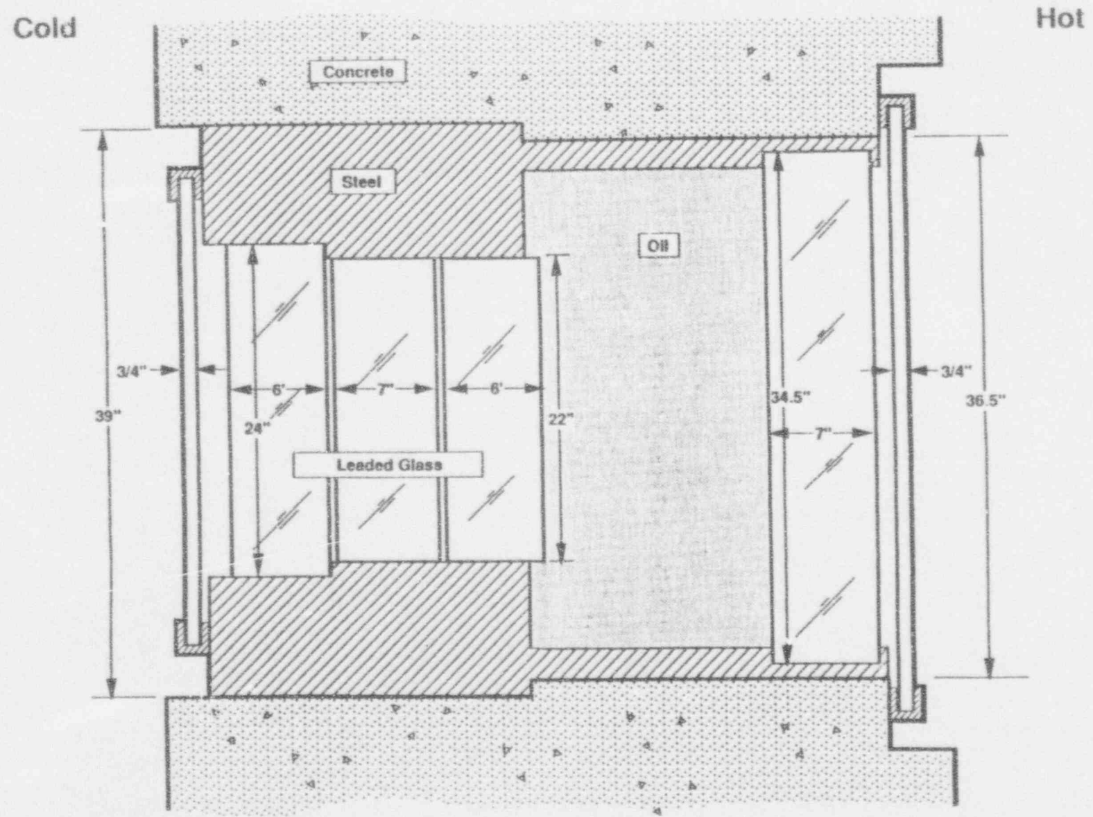
Figure 4-1. Geometry of the shield windows (Gates, 1993)
