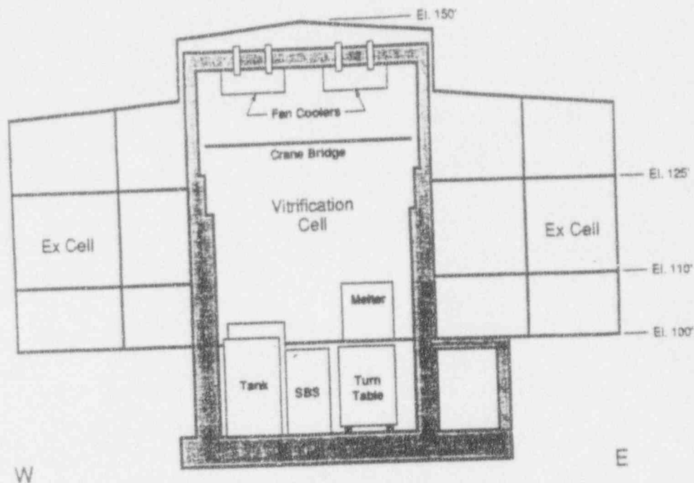
Vitrification Facility E-W Section
