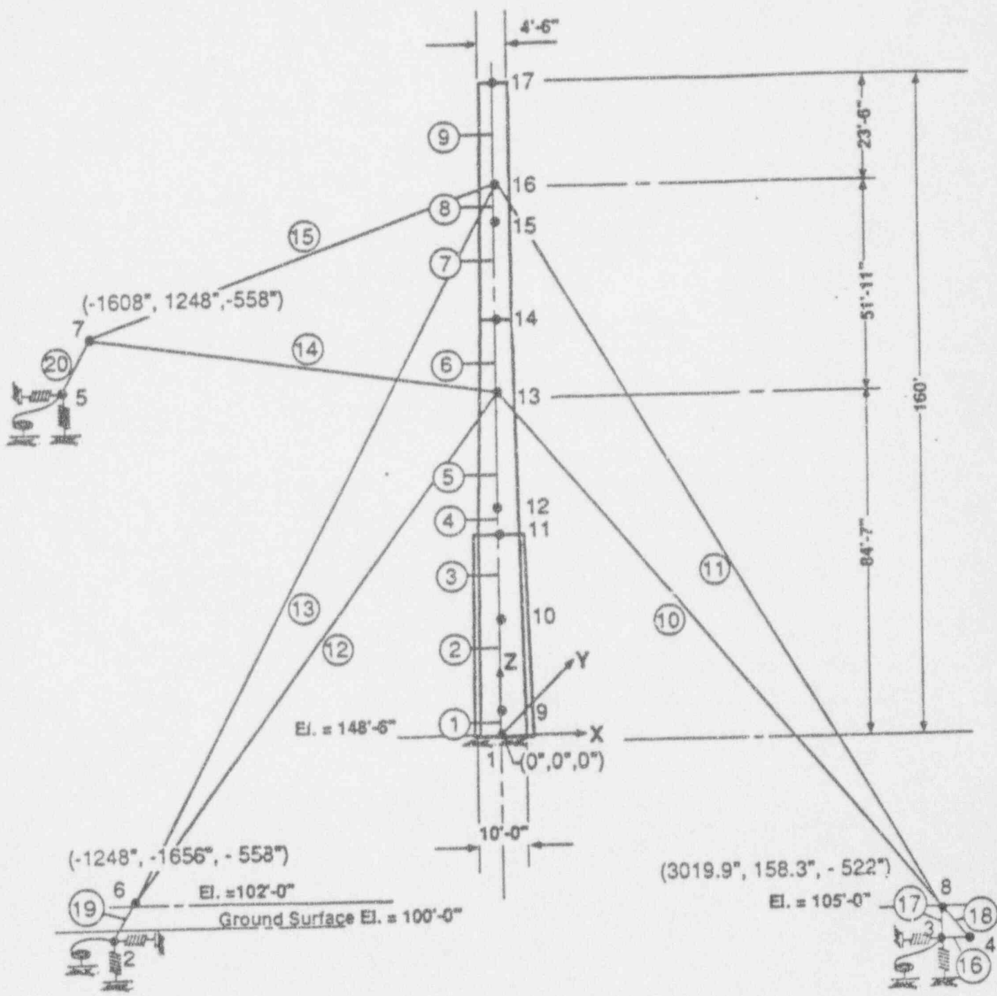
Figure 3-4. Dames & Moore FEA model of reprocessing plant guyed stack (Gates, 1993)
