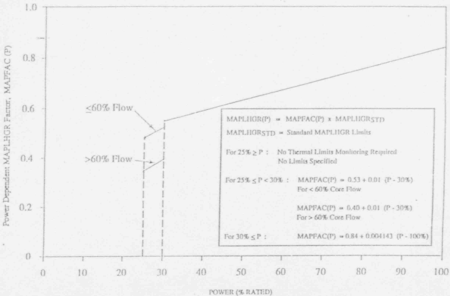
POWER DEPENDENT MAPLHGR MULTIPLIER MAPFAC(P) THIS FIGURE IS REFERRED TO BY TECHNICAL SPECIFICATION 3.2.1 THIS FIGURE IS VALID FOR THE RPTOOS AND/OR TBOOOS OPERATING DOMAINS
