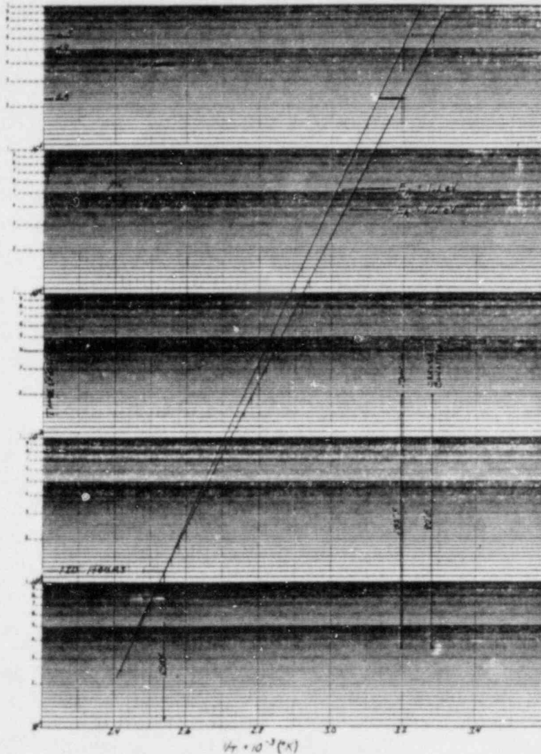
Figure 1. Sensitivity of Arrhenius Model to Small Changes in E_A
