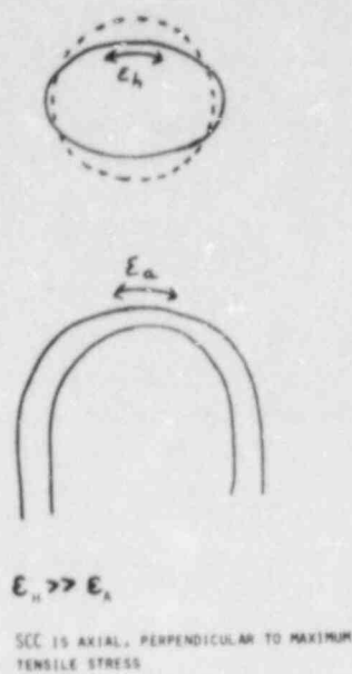
FIGURE 2: SKETCH OF OVALIZATION AT TOP OF U-BEND THAT OCCURS WHEN MOTION OF TUBE SUPPORT PLATE, RESULTING FROM DENTING, DECREASES THE DISTANCE BETWEEN THE HOT AND COLD LEGS
