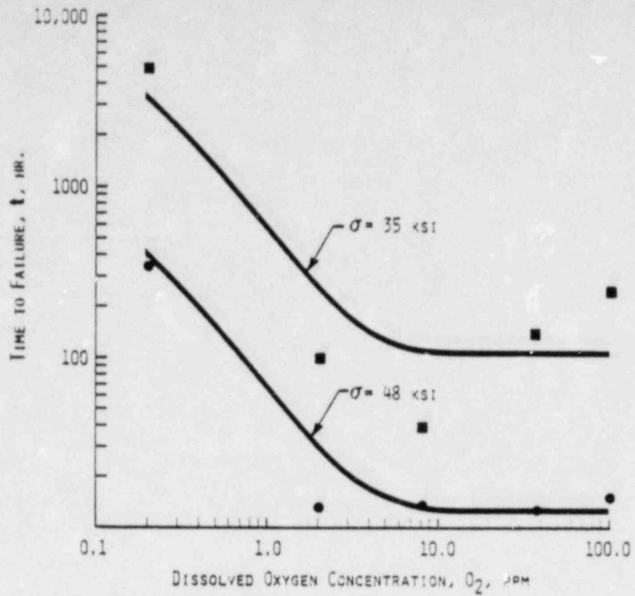
Figure 9 - Comparison of Oxygen Term and Constant Load Data at 288^\circ\text{C} , P_a = 40 \text{ C/cm}^2 , a = 0.01 Assumed.
