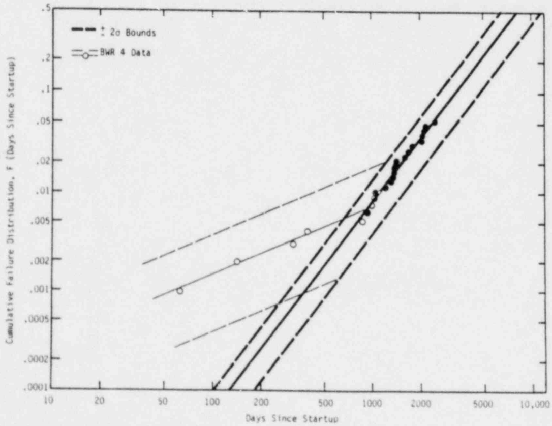
Figure 2 - Recirculation Bypass Failures, All Plants.
