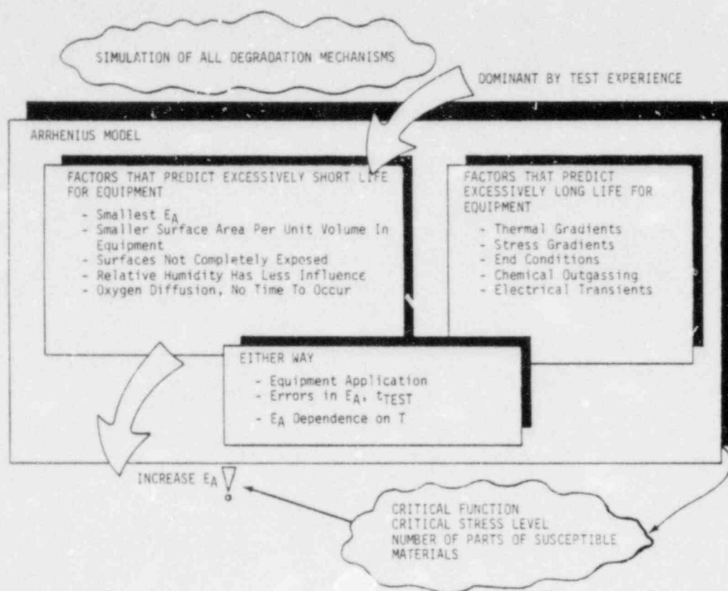
Figure 8. Accelerated Thermal Aging, Summary
