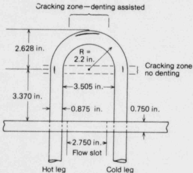
FIGURE 1B: SCHEMATIC OF U-END, SHOWING WHERE PRIMARY SIDE SCC HAS OCCURRED
