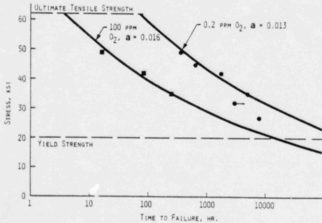
Figure 10 - Comparison of Stress Term with Furnace-Sensitized Constant Load Data, P_a = 40 , T = 288^\circ\text{C} .
