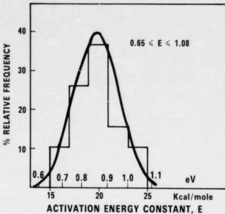
FIGURE 3. TGA DATA ON FORMVAR, DISTRIBUTION IN SLOPE
