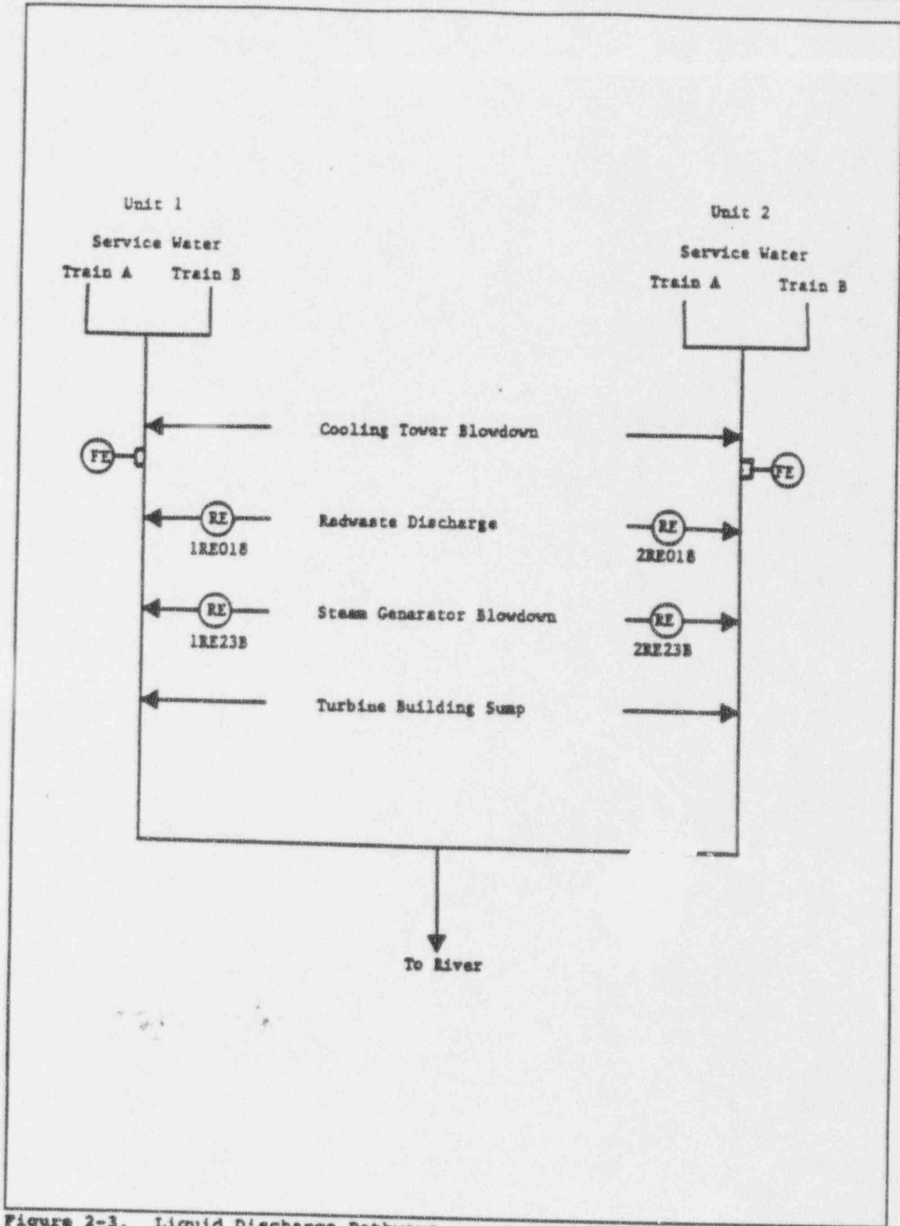
Figure 2-3. Liquid Discharge Pathways
