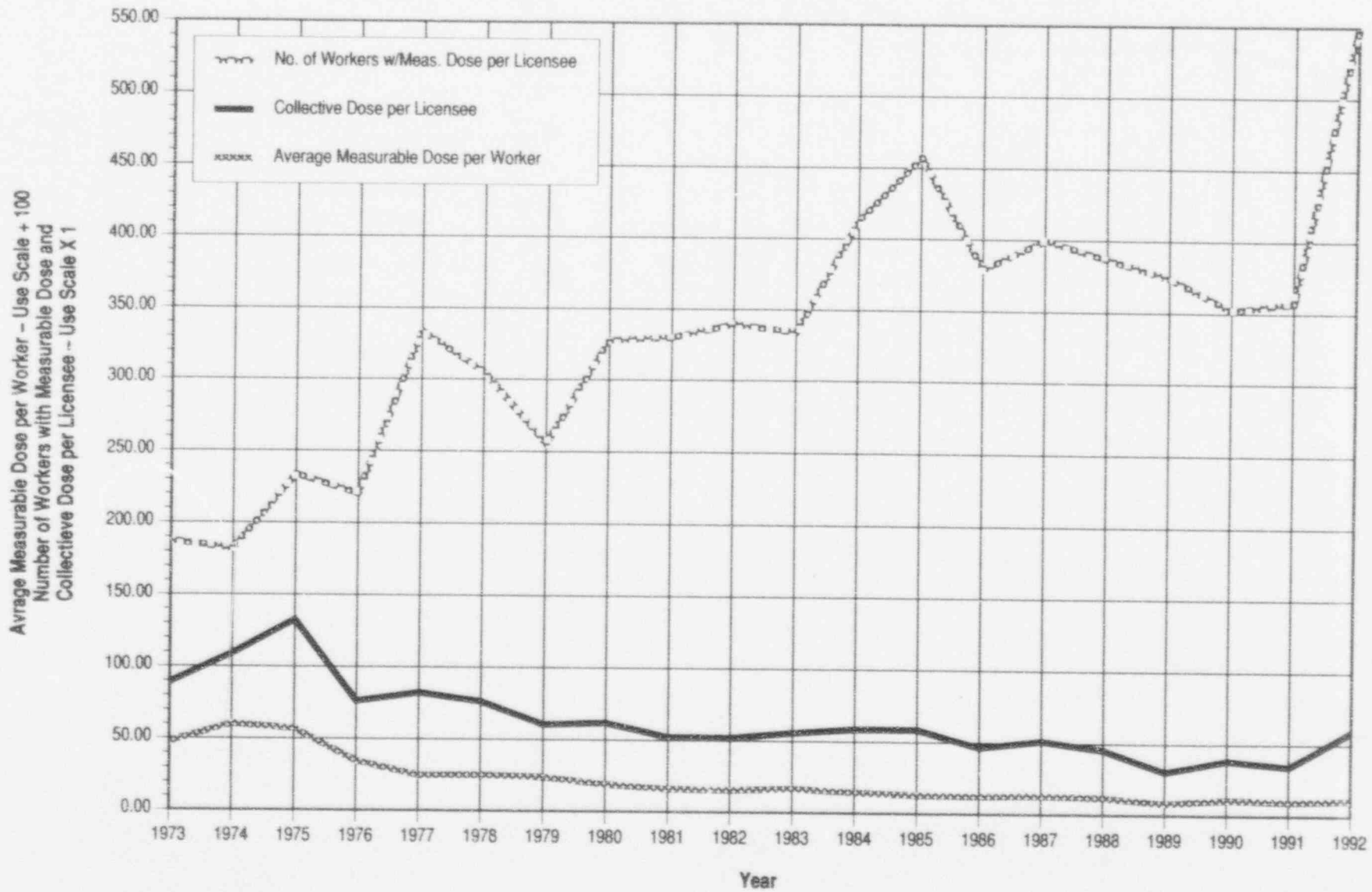
Figure 3.6 Average Annual Values at Fuel Fabrication and Processing Facilities 1973 - 1992
