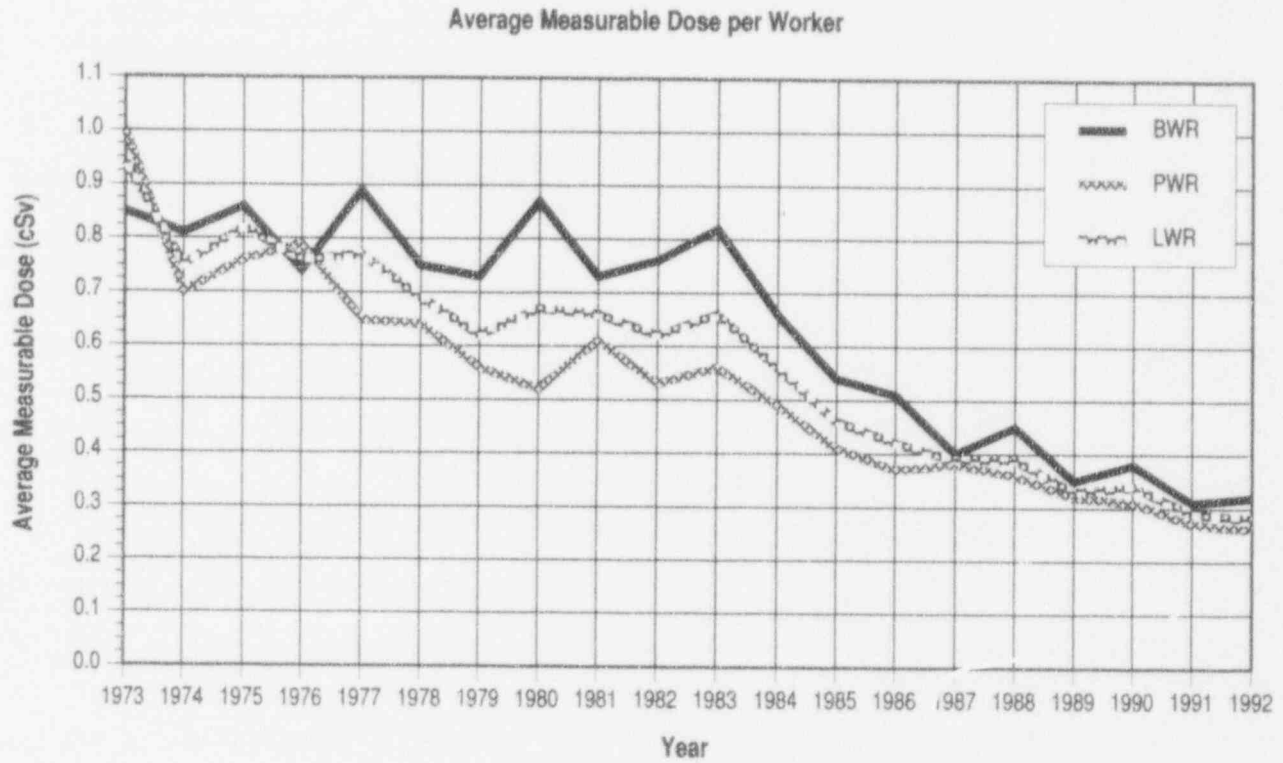
Figure 4.3 Average Measurable Dose per Worker and Collective Dose per Megawatt-Year 1973 – 1992
