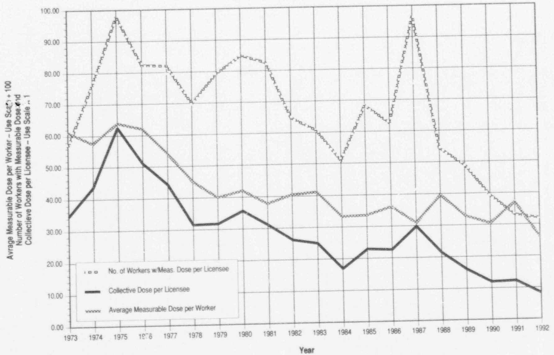
Figure 3.3 Average Annual Values at Manufacturing and Distribution Facilities 1973 - 1992
