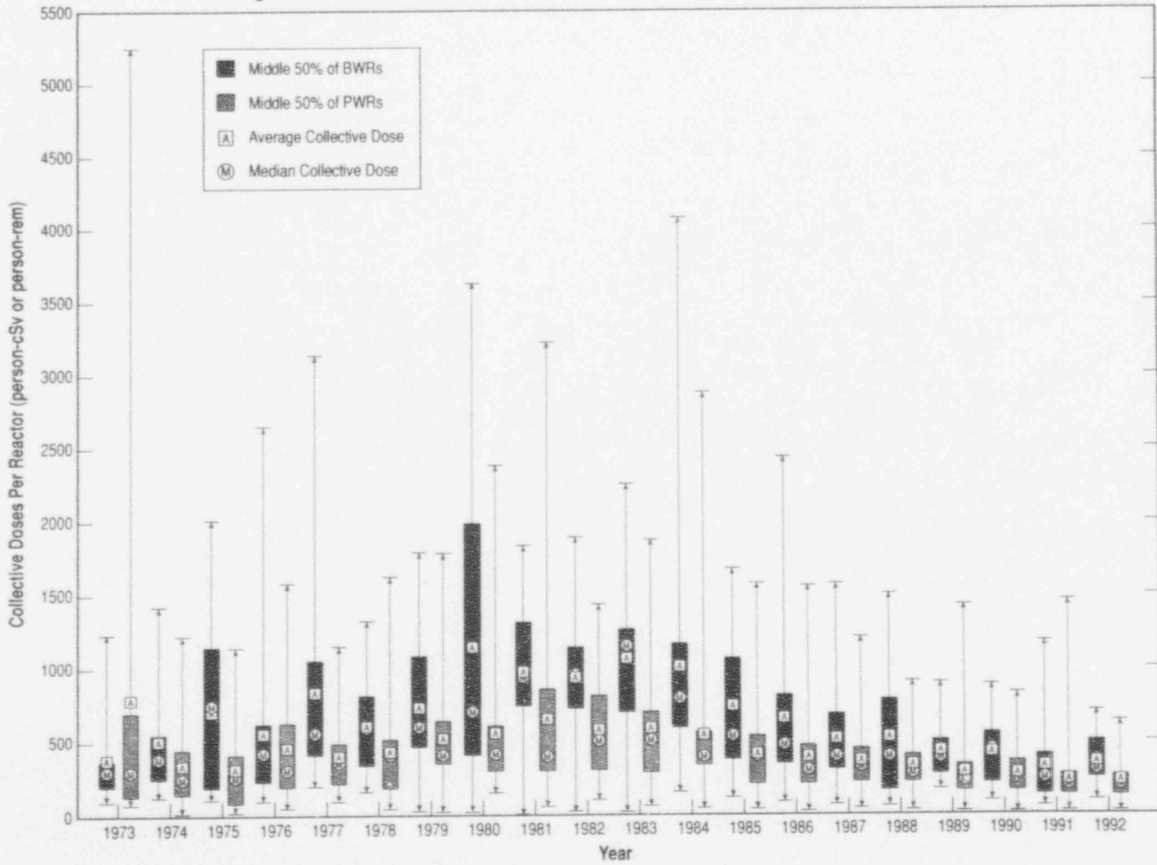
Average, Median, and Extreme Values of the Collective Dose Per Reactor 1973 - 1992
