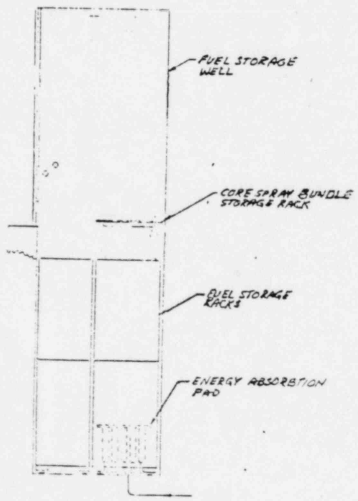
PROPOSED ARRANGEMENT
