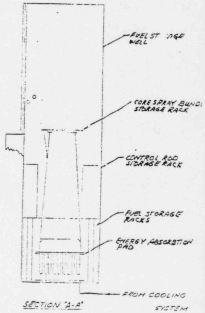
PRESENT ARRANGEMENT
