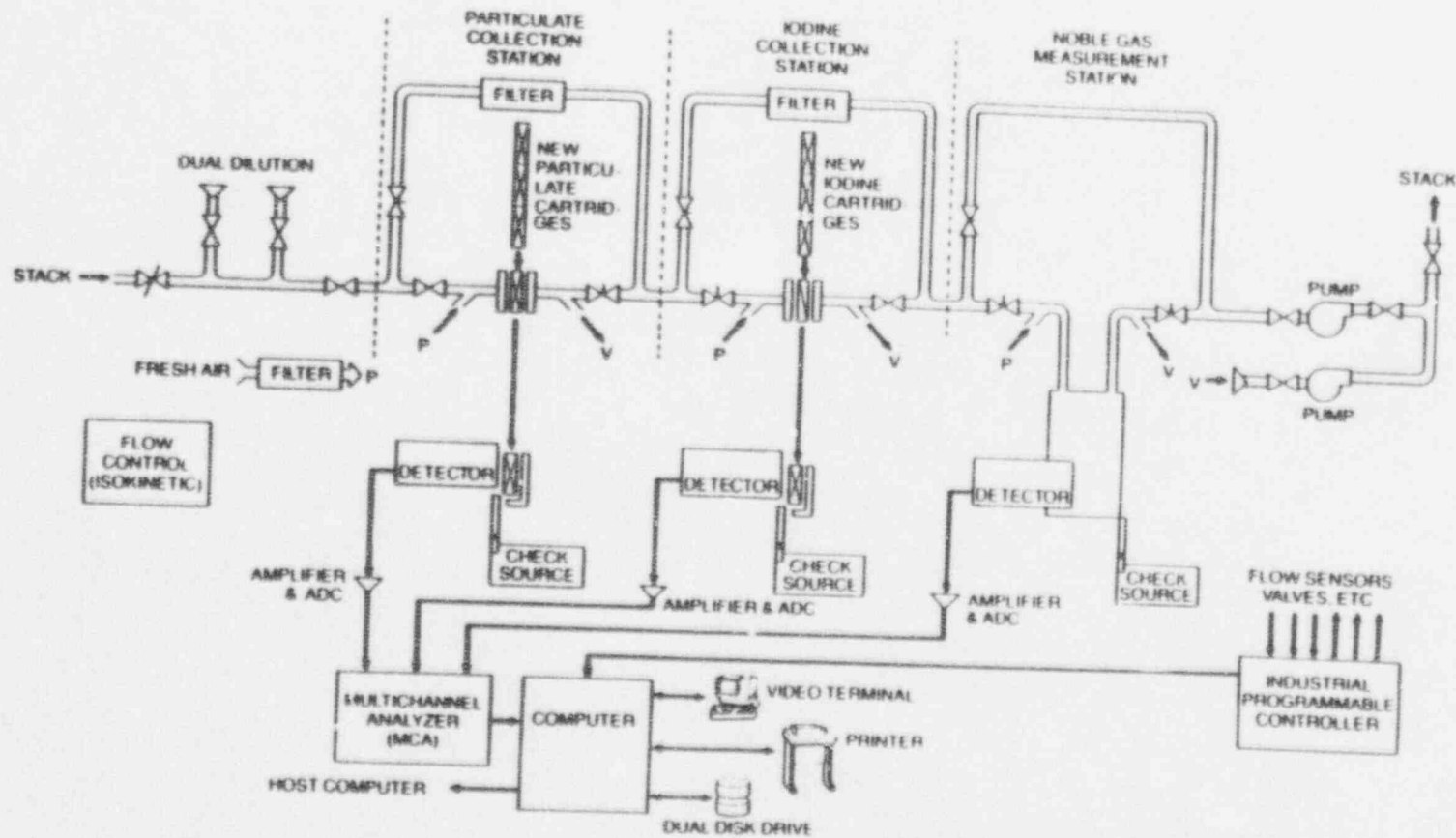
BLOCK DIAGRAM TYPICAL GASEOUS EFFLUENT MONITORING SYSTEM
