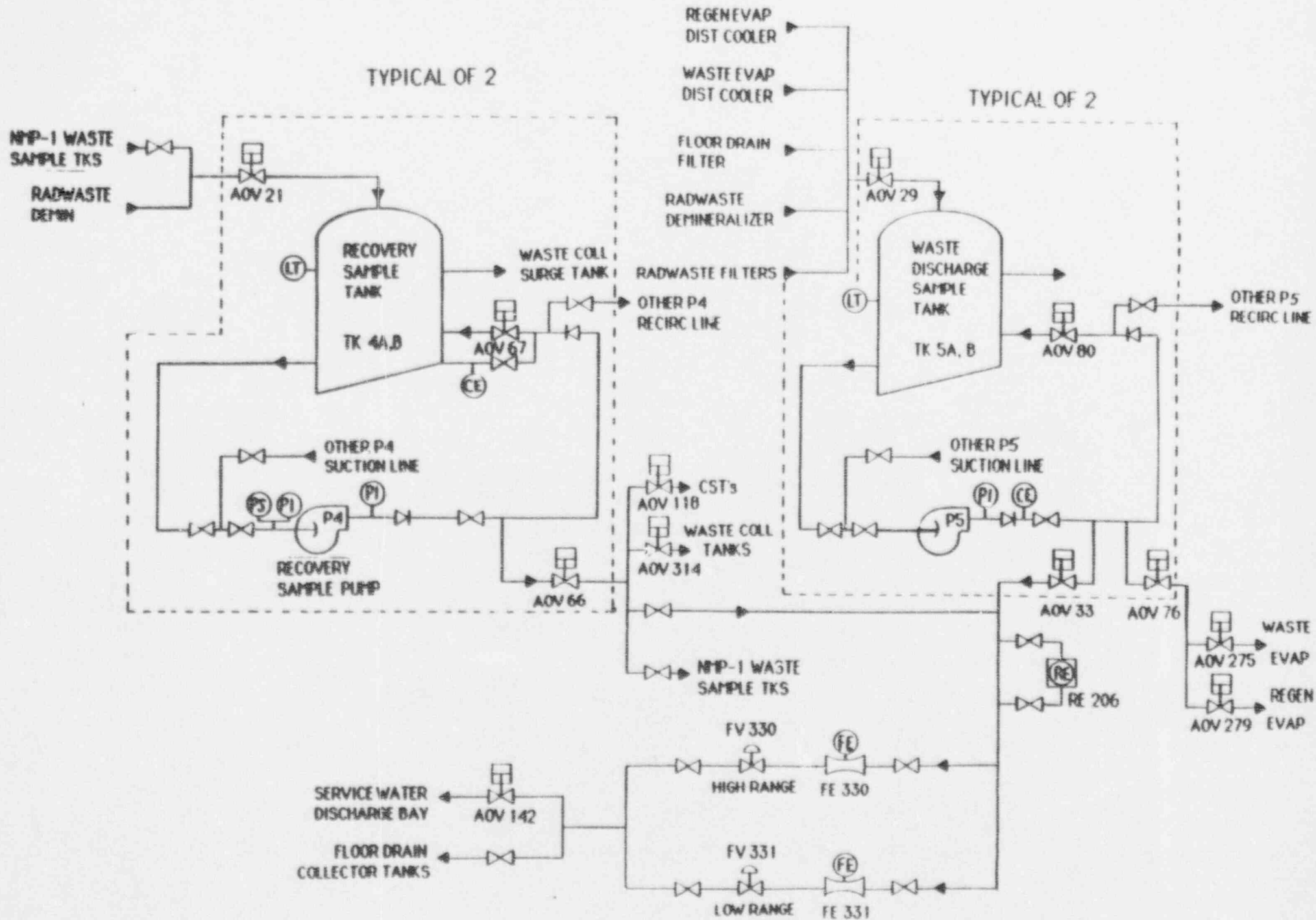
RECOVERY SAMPLE SYSTEM and
