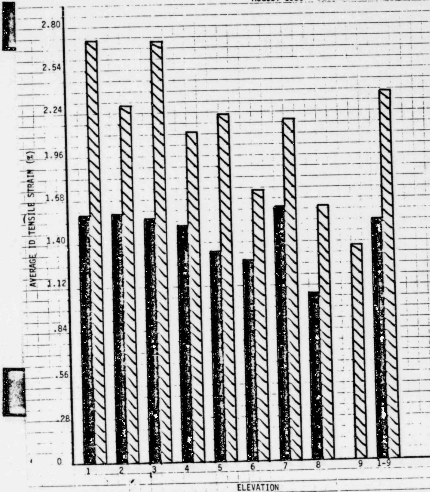
FIGURE 5 COMPARISON OF AVERAGE ID TENSILE STRAIN VERSUS ELEVATION MILLSTONE UNIT No. 2 (HL) AUGUST 1980 - DECEMBER 1981
