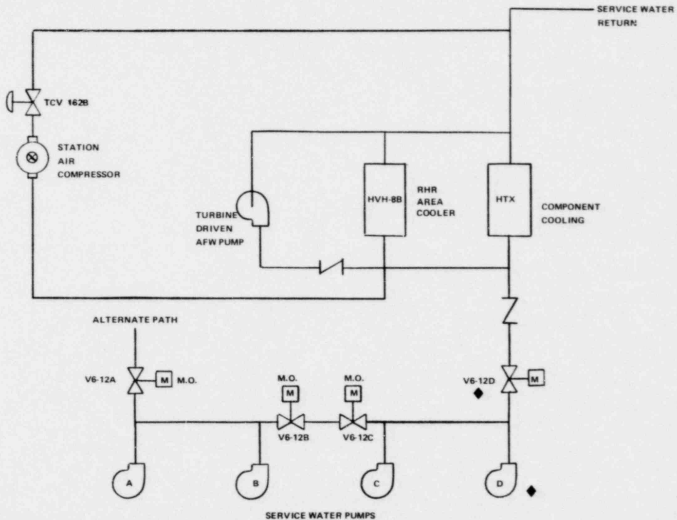
SERVICE WATER SYSTEM FIGURE 1, SHEET 6
