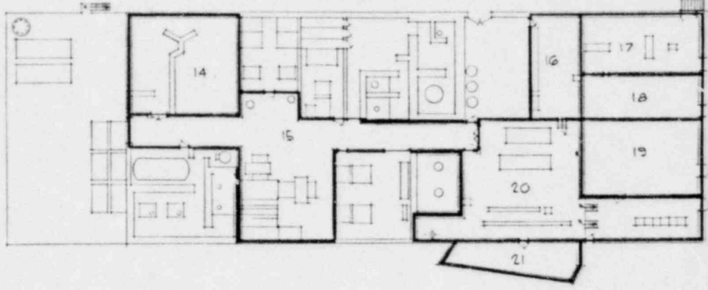
AUXILIARY BUILDING FLOOR EL. 242-0 N 246-0
