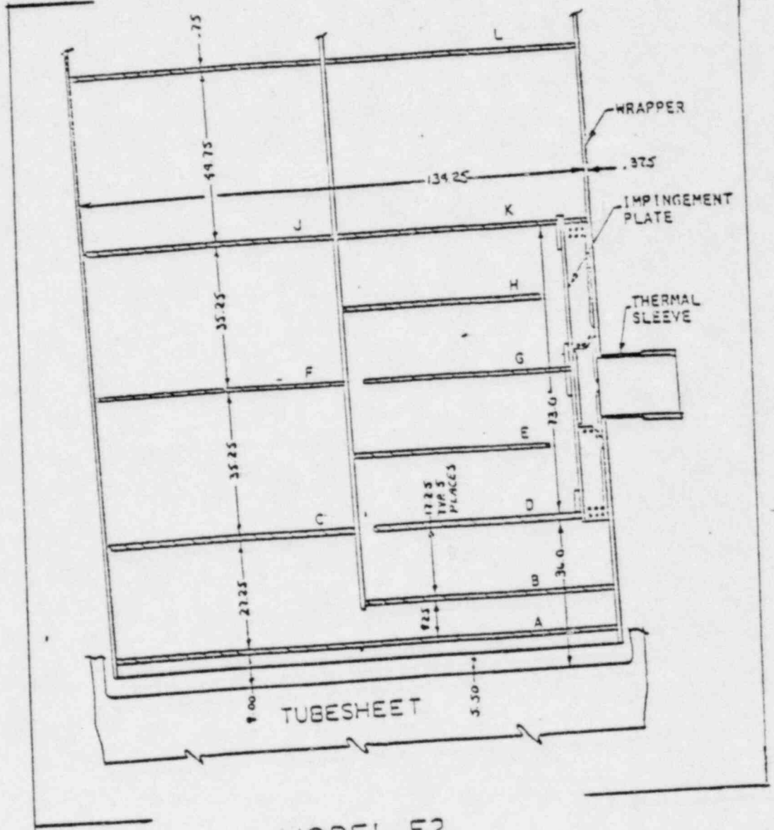
MODEL E2 PREHEATER INTERNALS
