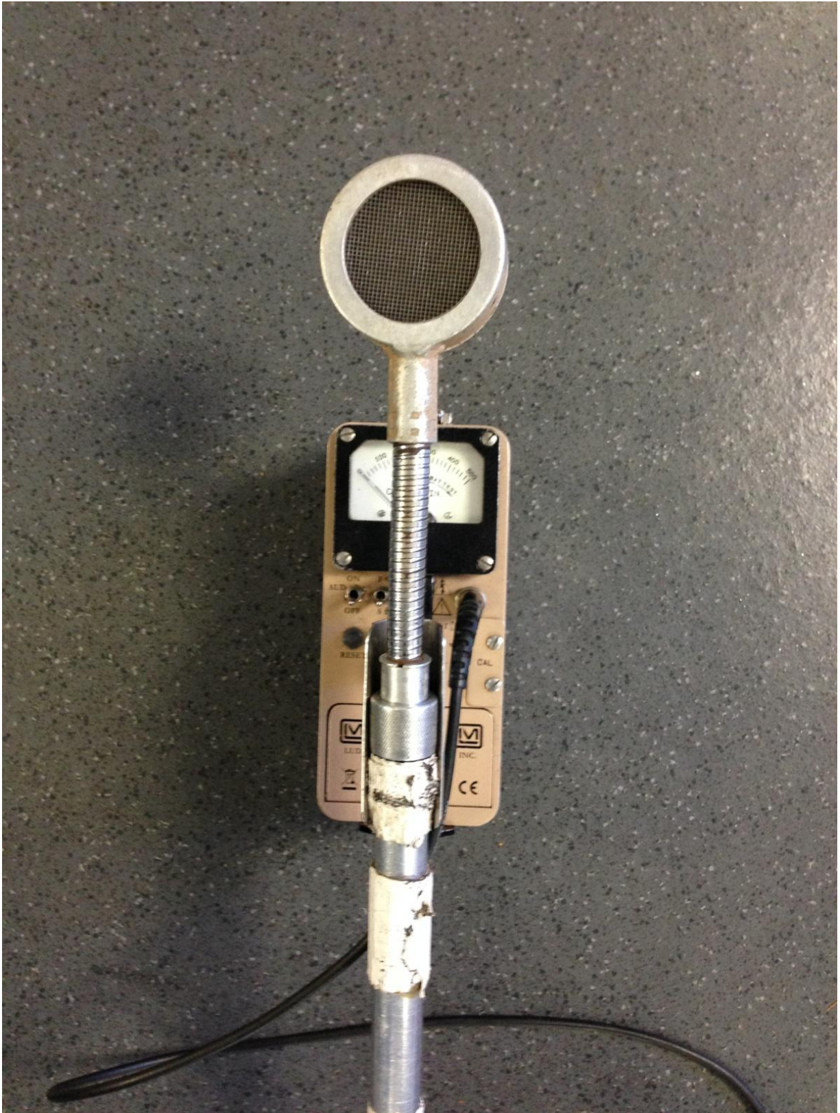
Ludlum Model 21 Ratemeter with GM Probe
