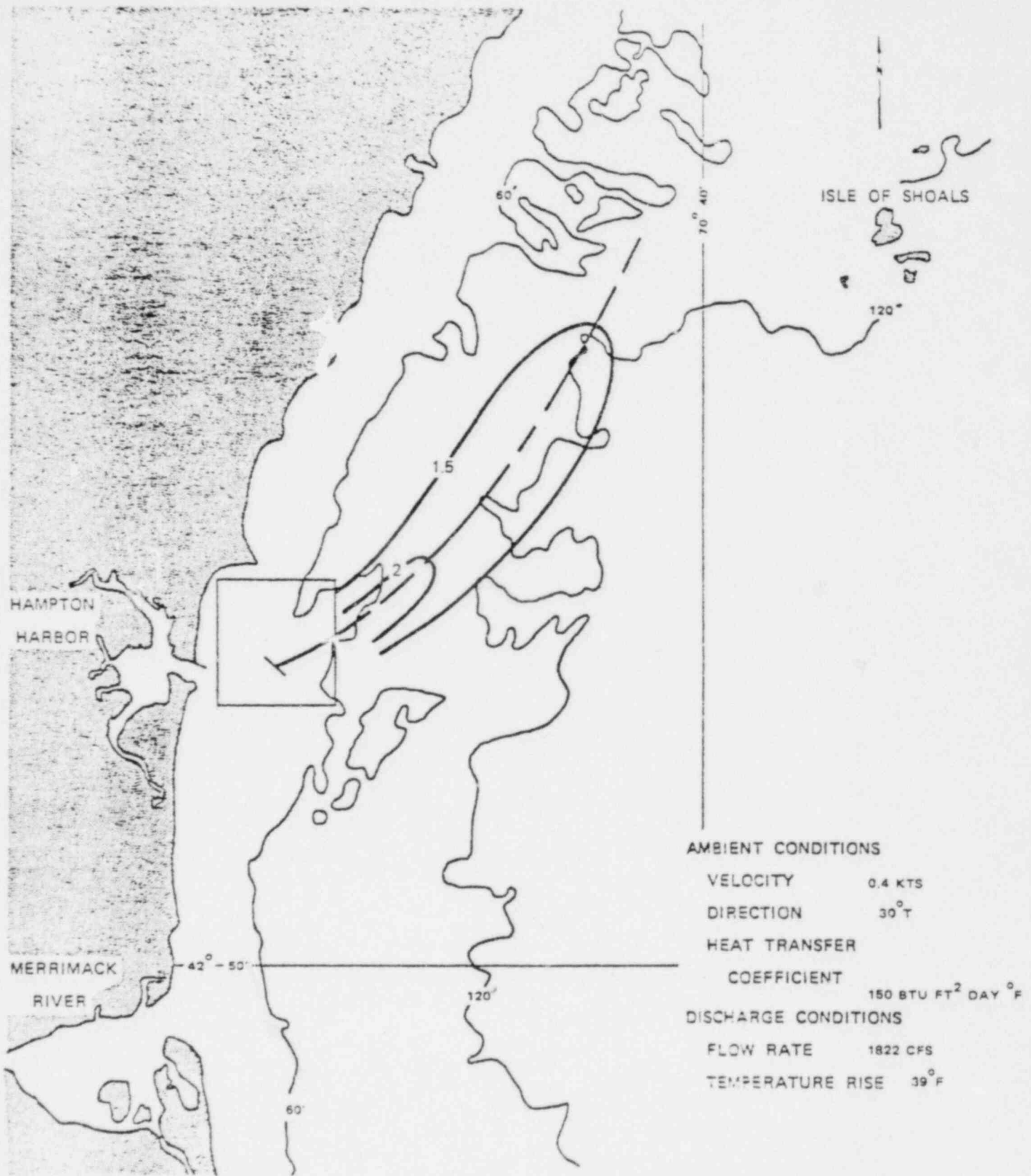
ISOTHERMS - FLOW TO NORTH
