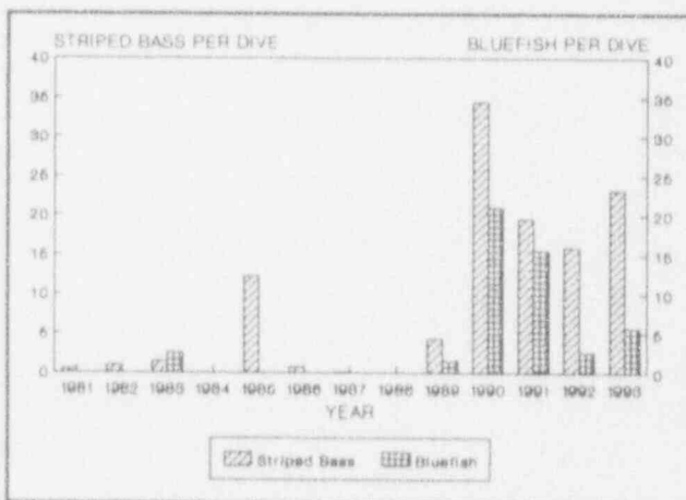
Figure 8. Index of relative abundance (fish per dive) for striped bass and bluefish observed by divers at Pilgrim Station, 1981 to 1993.
