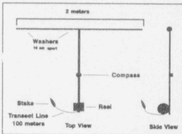
Figure 2. Survey tool used by divers for abundance and size estimation along trawl transects in the Pilgrim Station area.
