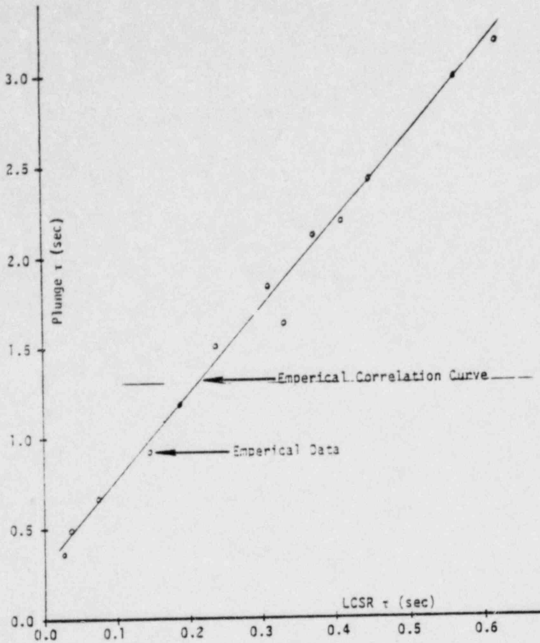
Figure 3.2 Empirical Correlation Curve for Plunge \tau versus LCSR \tau for Rosemont RTD Model 176KF. (Westinghouse RTD)
