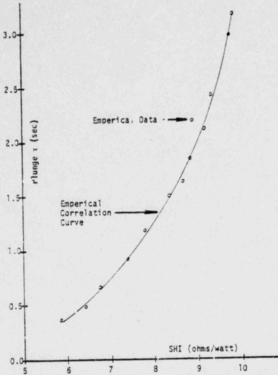
Figure 3.4 Emperical Correlation Curve for Plunge \tau versus SHI for Rosemont RTD Model 176KF. (Westinghouse RTD)
