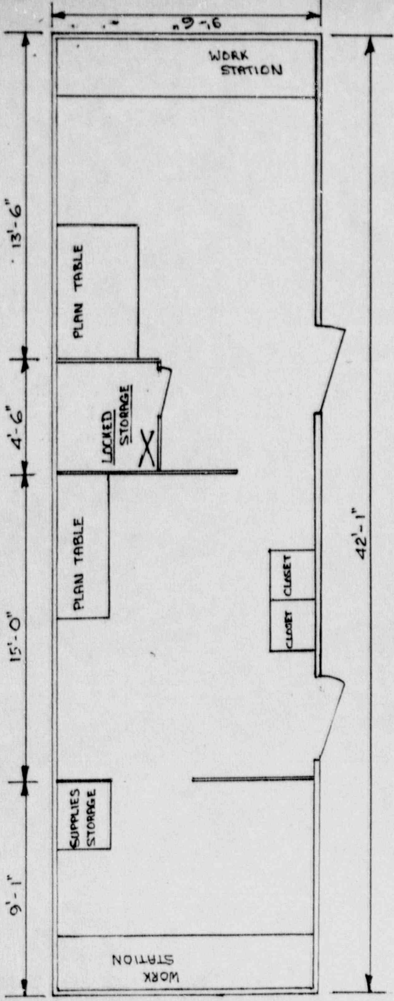
PLAN OF TRAILER USED FOR STORING GAUGING DEVICE
