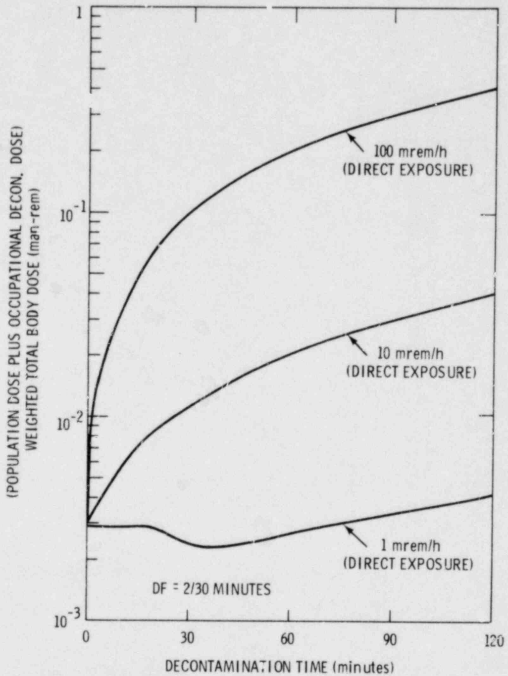
FIGURE 3.4-2 Total Dose Versus Decontamination Time for Spent Fuel Beta-Gamma Mixture - Starting at a Level of 10^{-4} \mu\text{Ci}/\text{cm}^2 - DF = 2/30 Minutes
