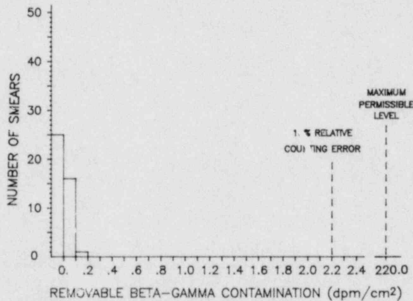
FIGURE 5.7-4 Frequency Distribution for Industrial Sources - Beta-Gamma Contamination
