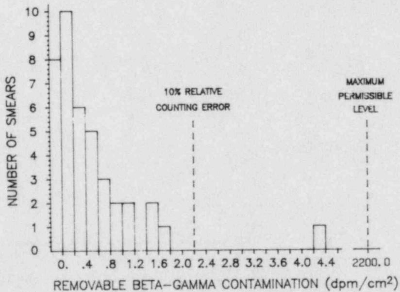
FIGURE 5.7-6 Frequency Distribution for Uranium Shipments - Beta-Gamma Contamination
