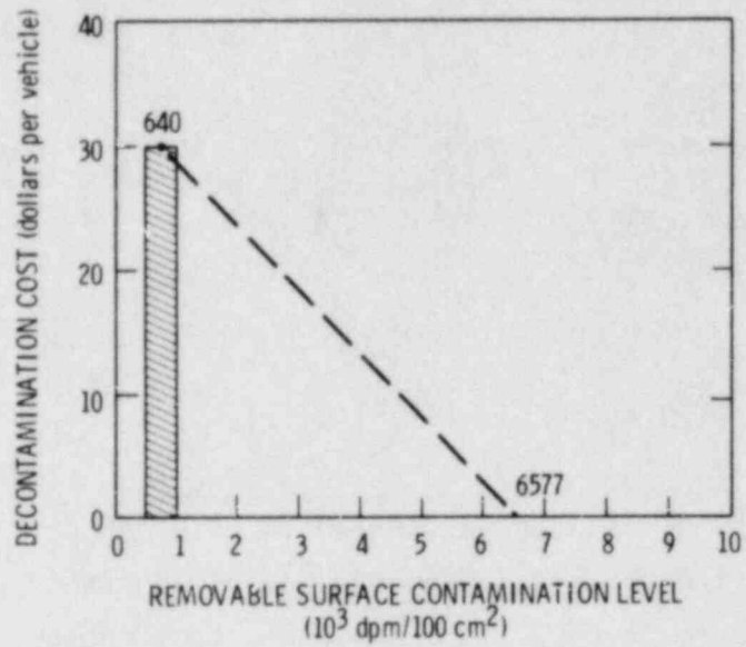
FIGURE 4.5-1 Cost-Contamination Relationship for Vehicles with One Decontamination
