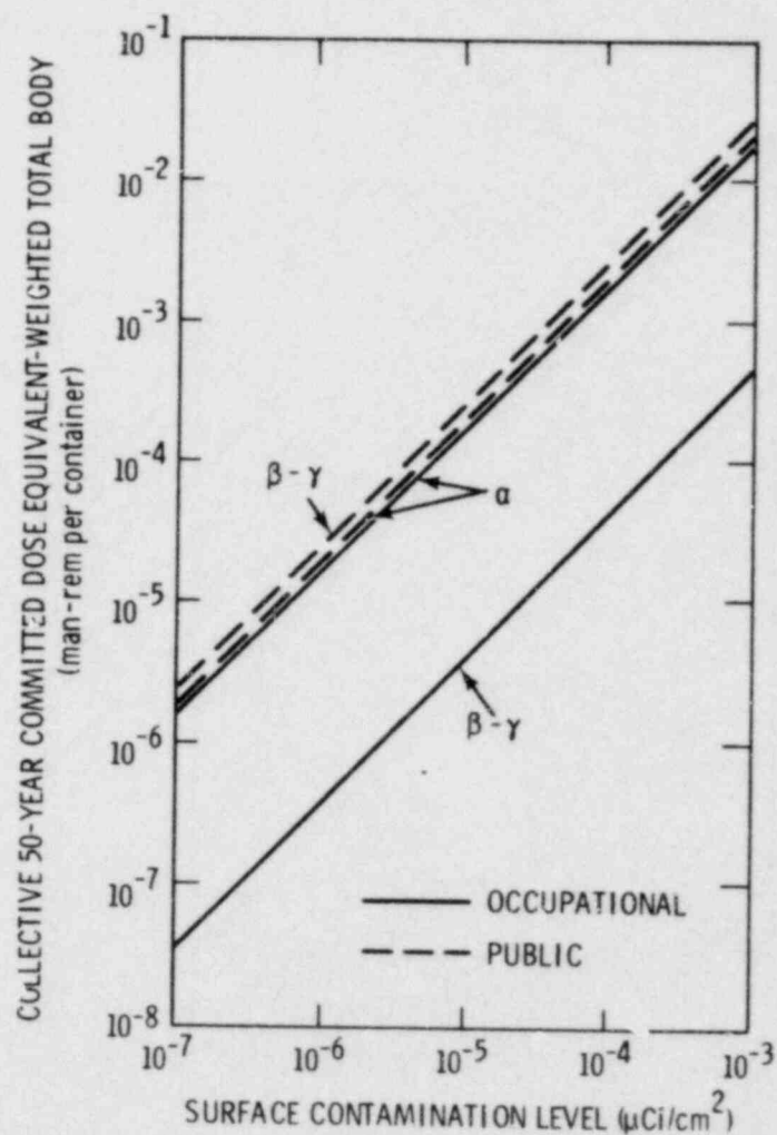
FIGURE 3.6-4 Collective Doses from Surface Contamination on Spent Fuel Transportation Containers
