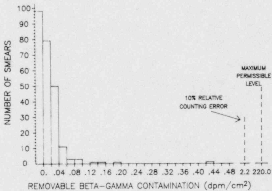
FIGURE 2.2-5. Frequency Distribution for Radiopharmaceuticals - Beta-Gamma Contamination
