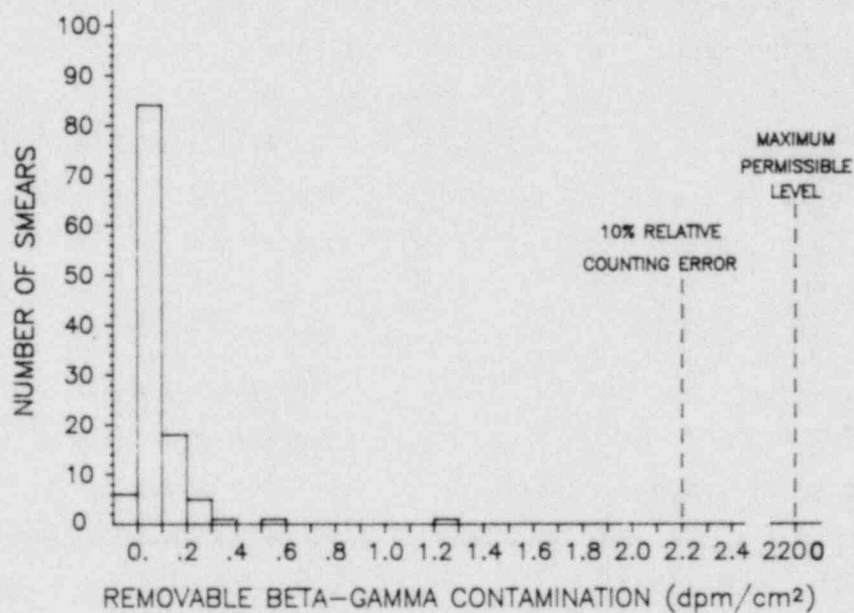
FIGURE 5.7-10 Frequency Distribution for Low-Level Radioactive Waste - Beta-Gamma Contamination (Exclusive Use Shipments)
