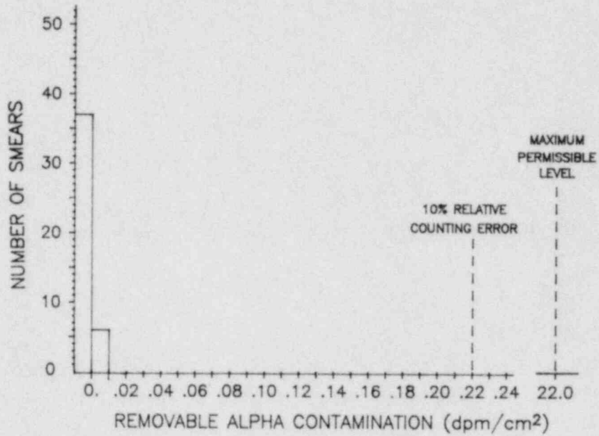
FIGURE 5.7-3 Frequency Distribution for Industrial Sources - Alpha Contamination
