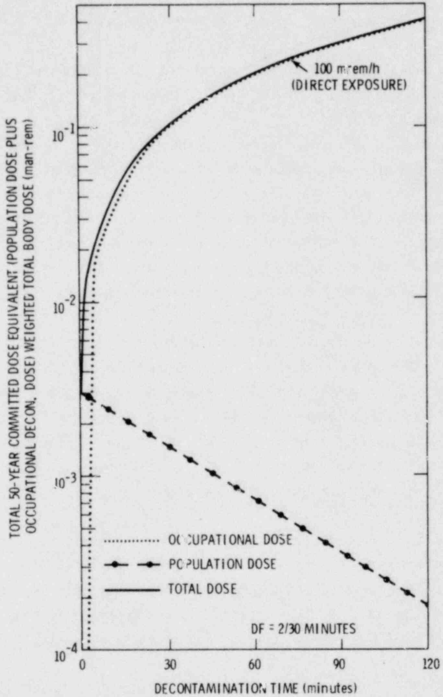
FIGURE 3.4-3 Population and Occupational Dose Comparison For Spent Fuel Cask Decontamination
