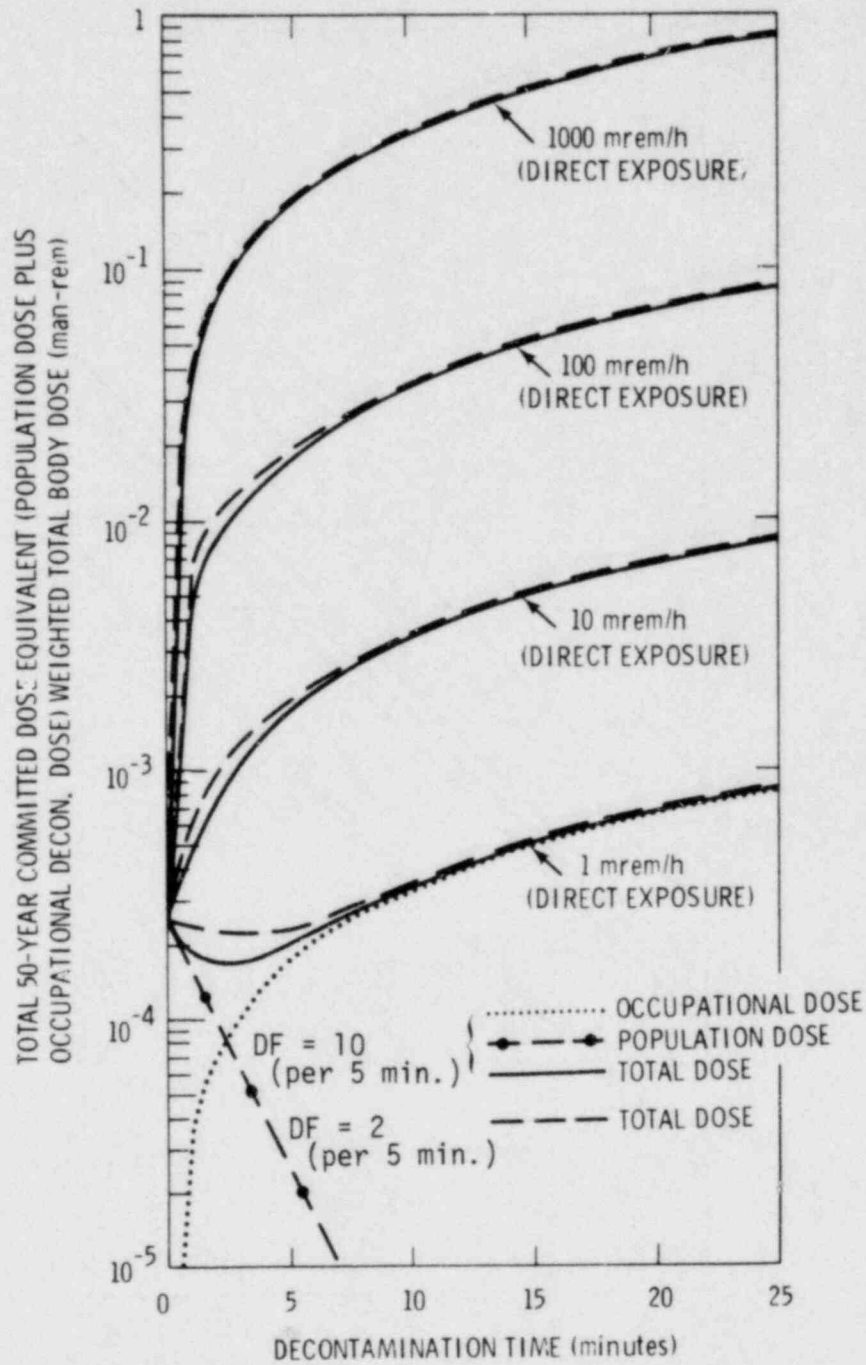
FIGURE 2.2-c Example Total Dose Versus Decontamination Time for ^{129}\text{I} Starting at a Level of 10^{-4} \mu\text{Ci}/\text{cm}^2 - Low Level Radioactive Waste Transportation Containers
