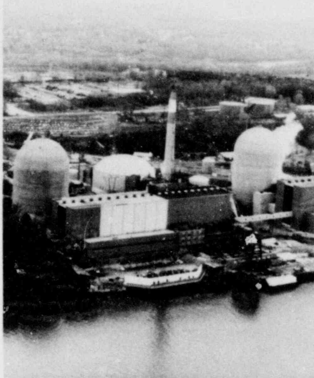
Indian Point Station in New York. The inoperative Unit 1 is at center, flanked by Unit 2 on the left and Unit 3 at right.
