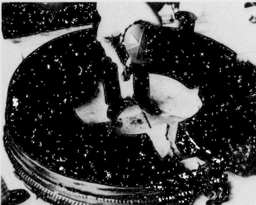
A turbine disc that failed at the Yankee Nuclear Power Station, Rowe, Mass., in January 1980. Preliminary analysis indicated the cause was stress corrosion cracking.
