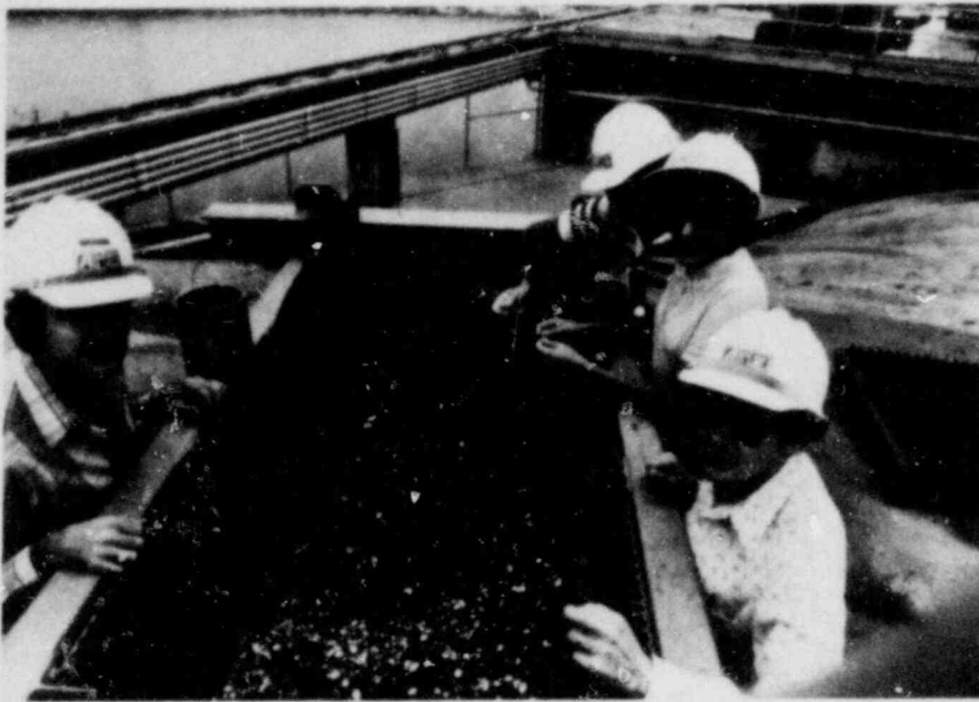
Employees of Arkansas Power & Light Co., at Unit 2 of the Arkansas Nuclear One station, near Russellville, are shown with thousands of Asiatic clams being removed from the intake bay of the plant's cooling water system. The unit had to be shut down because of inadequate flow of service water through the containment air coolers. The freshwater clams, attracted by the slightly warmer water, had gotten into the system, grown and caused the blockage. First discovered in the United States on the West Coast in 1938, the clams have spread rapidly into at least 33 States, and have been found at virtually all of the Tennessee Valley Authority's generating stations.
