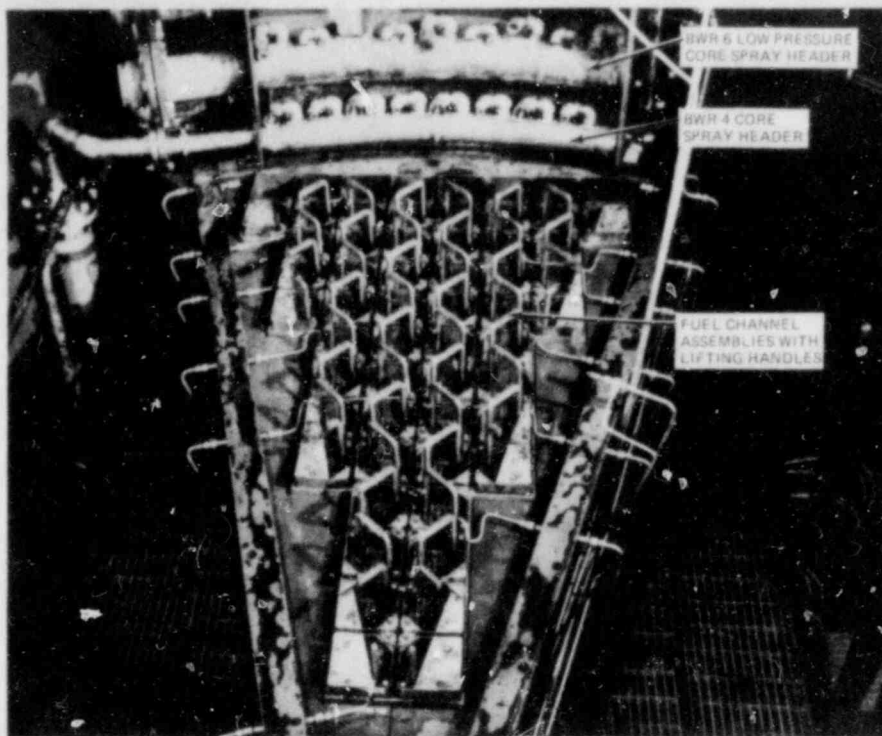
An important feature of the Sector Steam Test Facility in Lynn, Mass., is a full-scale model of a 30-degree sector of a boiling water reactor upper plenum. Experiments with this sector, which is shown here from the center of the core looking down and outward, include investigations of the distribution of cooling water sprayed over the top of a core and how the cooling water penetrates fuel bundles.
