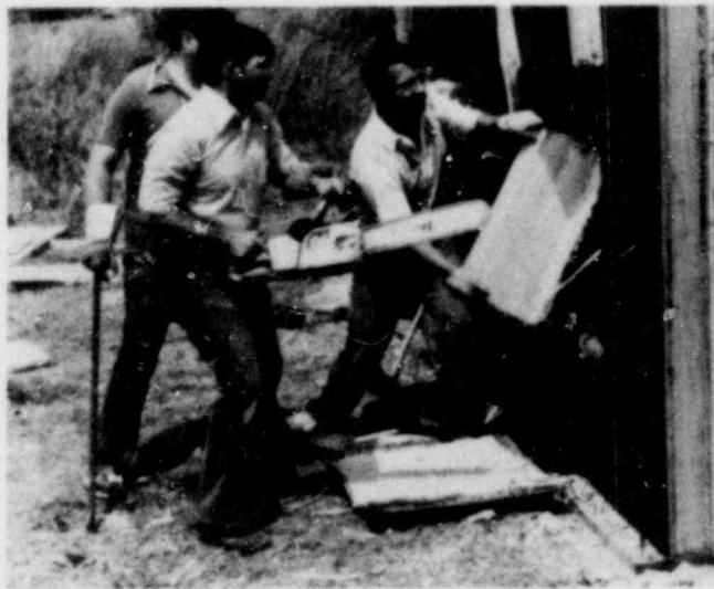
In support of the new requirements set forth in NRC's Physical Upgrade Rule, the Army Materiel Systems and Analysis Activity at Aberdeen Proving Grounds, Md., conducted a research program aimed at developing cost-effective barrier systems. The U.S. Army personnel shown here are testing the penetration resistance of a hardened barrier.
