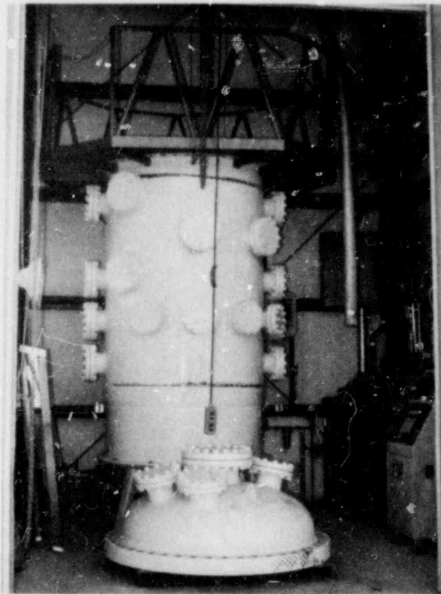
The Sandia Laboratories (N. Mex.) Steam Explosion Fully Instrumented Test chamber is used to assist in developing and validating the TRAP code, now nearing completion. The facility is shown here with the vessel head removed. Just to the right of the vessel is the induction melting power supply. Volume of the vessel is 5640 litres. Its inside diameter is about 1.5 meters. Height to the cat-walk is approximately 12 feet.
