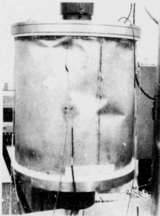
To establish safety margins for steel containments during routine operation or accident condition, the Los Alamos Scientific laboratory is performing buckling tests. Photo shows a steel containment that buckled in a preliminary high pressure test.
