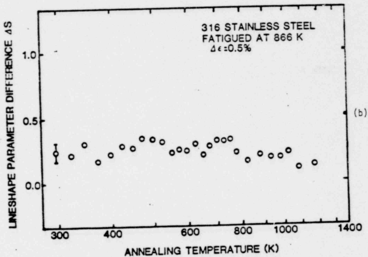
FIGURE 3. Isochronal annealing response of fatigued 316 stainless steel:
