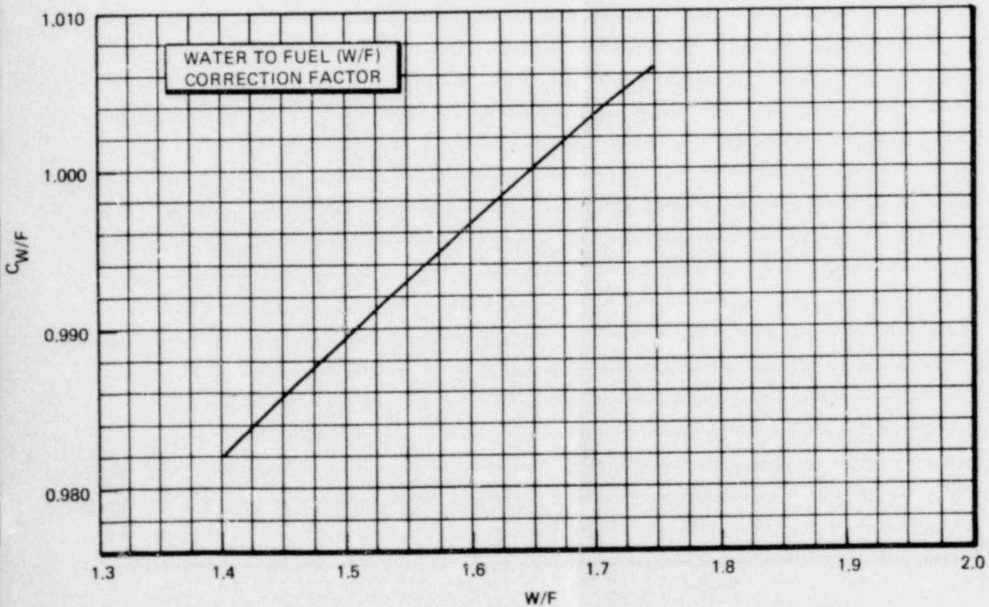
Figure 2-1. Rod Lattice k_{\infty} - PWR Fuel k_{\infty} = k_1 \times C_{WF} \times C_{PD} \times C_{CL}
