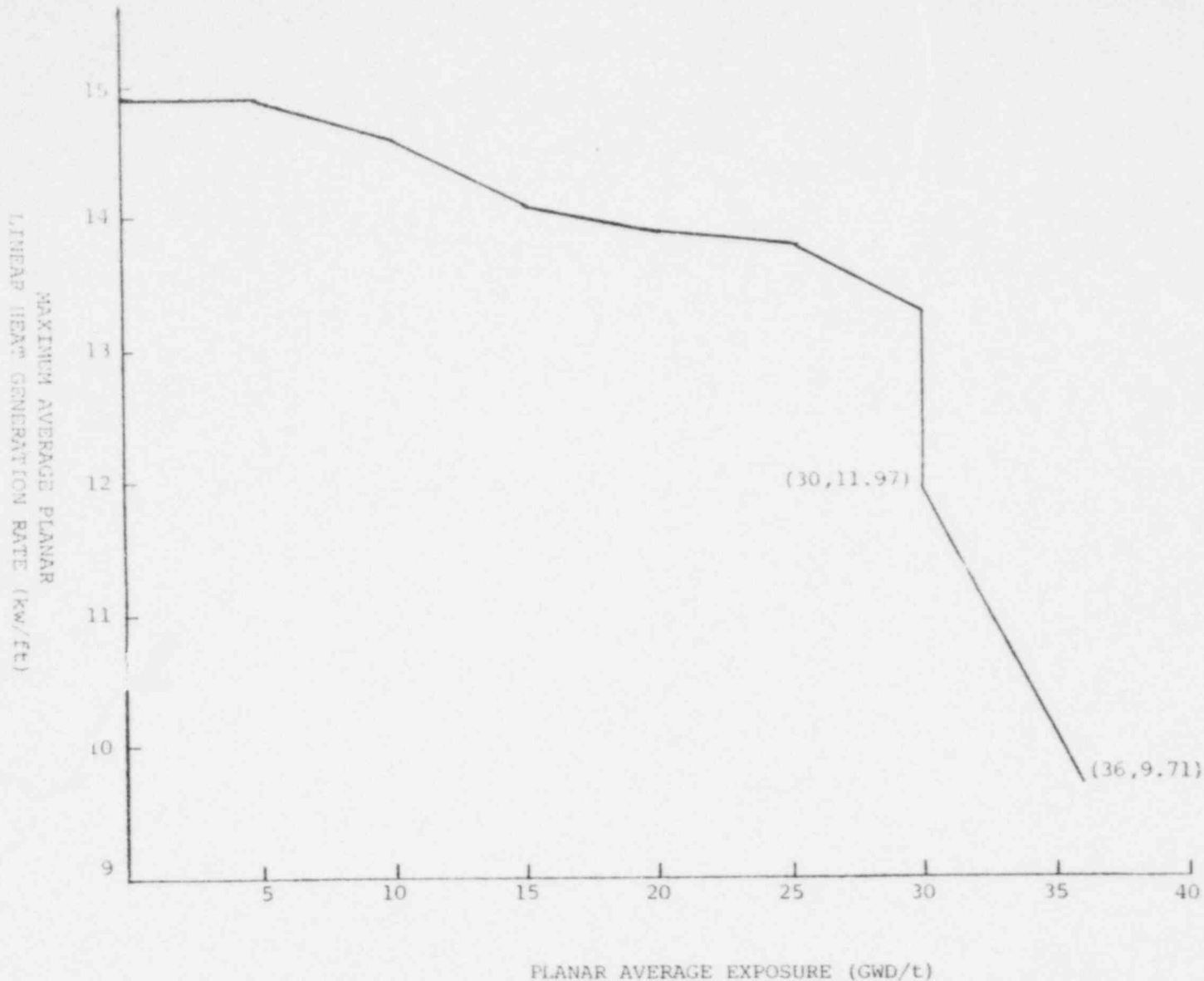
FIGURE 3.5-1 MAXIMUM AVERAGE PLANAR LINEAR HEAT GENERATION RATE (MAPLHGR) VERSUS PLANAR AVERAGE EXPOSURE
