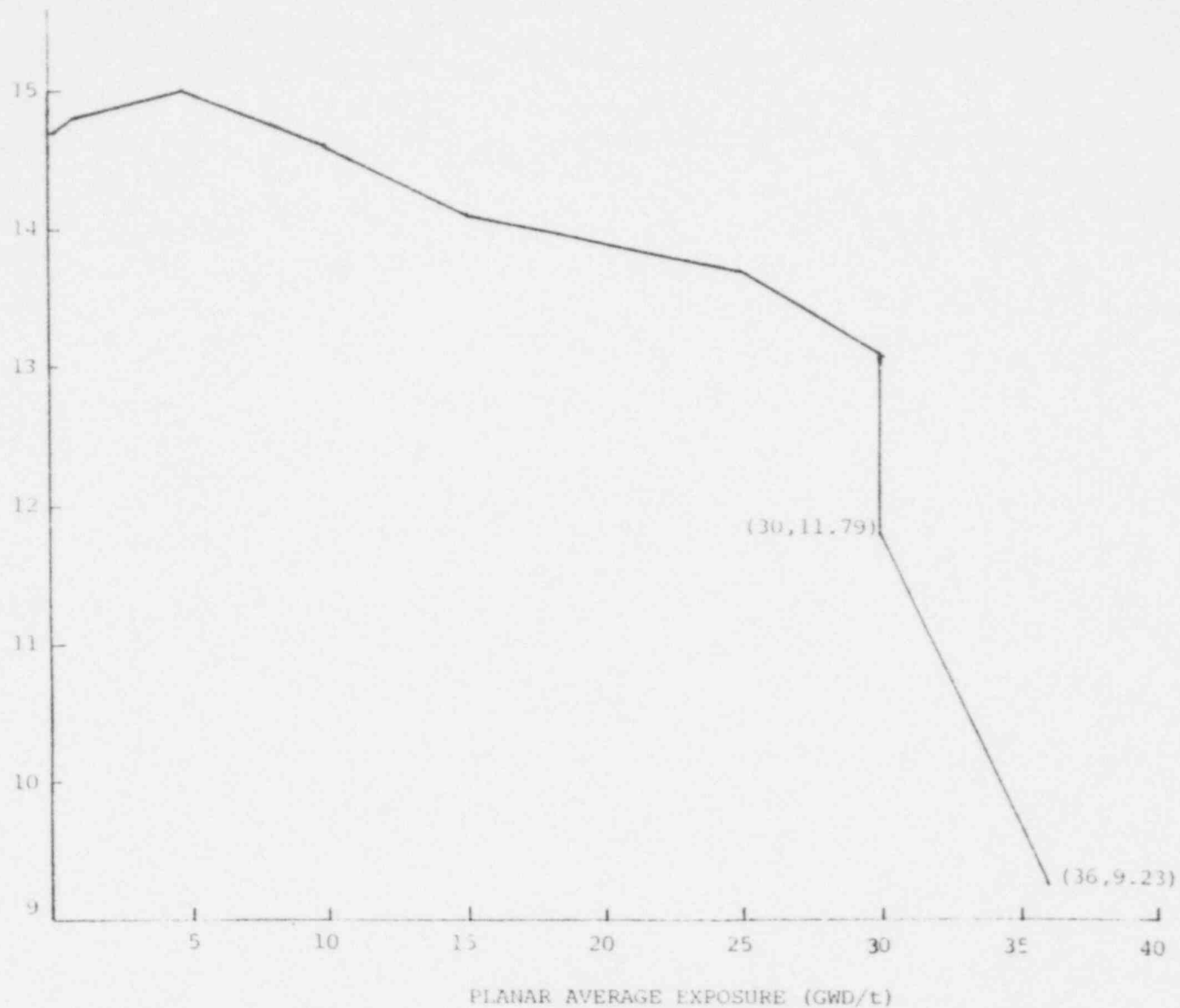
FIGURE 3.5-2 MAXIMUM AVERAGE PLANAR LINEAR HEAT GENERATION RATE (MAPLHGR) VERSUS PLANAR AVERAGE EXPOSURE
