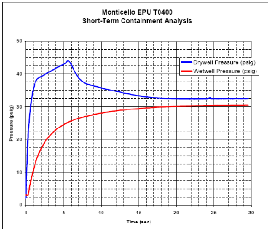
Figure 5.2-oa Drywell and Wetwell Response DBA-LOCA-Short Term
