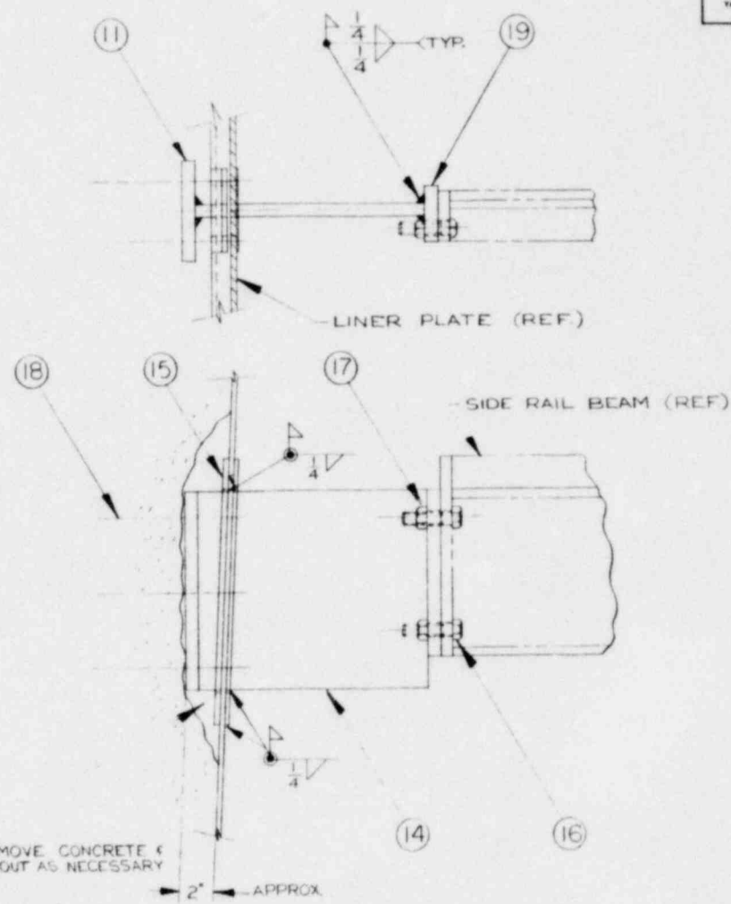
DETAIL "D" SEE SH 4
