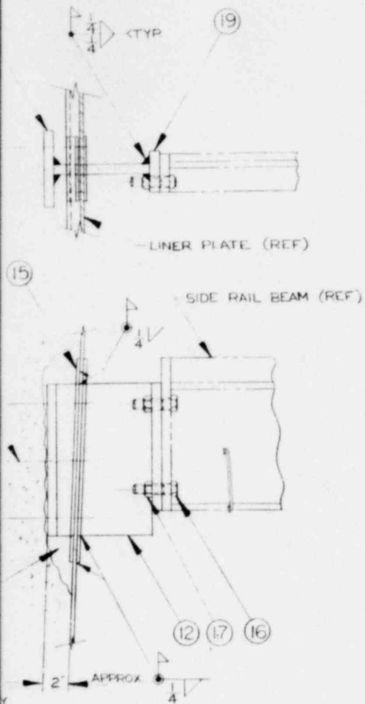
DETAIL "C" SEE SH 2,4
