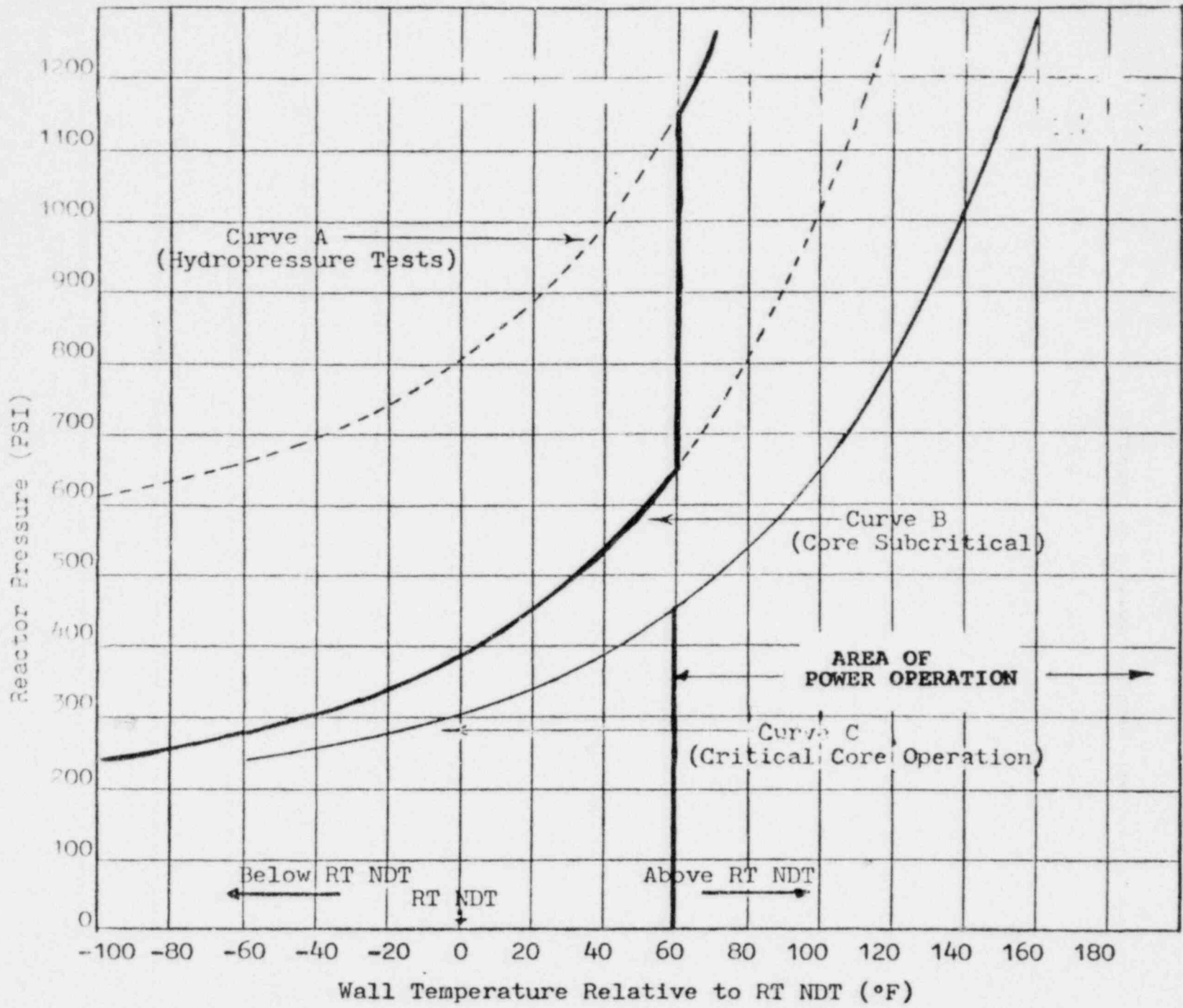
Figure 4.6.2 Pressure-Temperature Relationships for Dresden 1 Per 10CRF50 Appendix G
