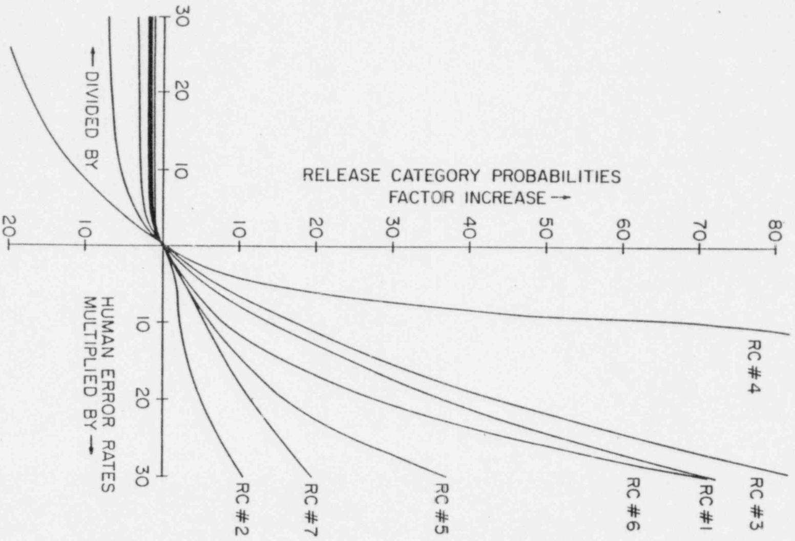
Fig. 2. Sensitivity of release category probabilities to changes in all the human error rates.
