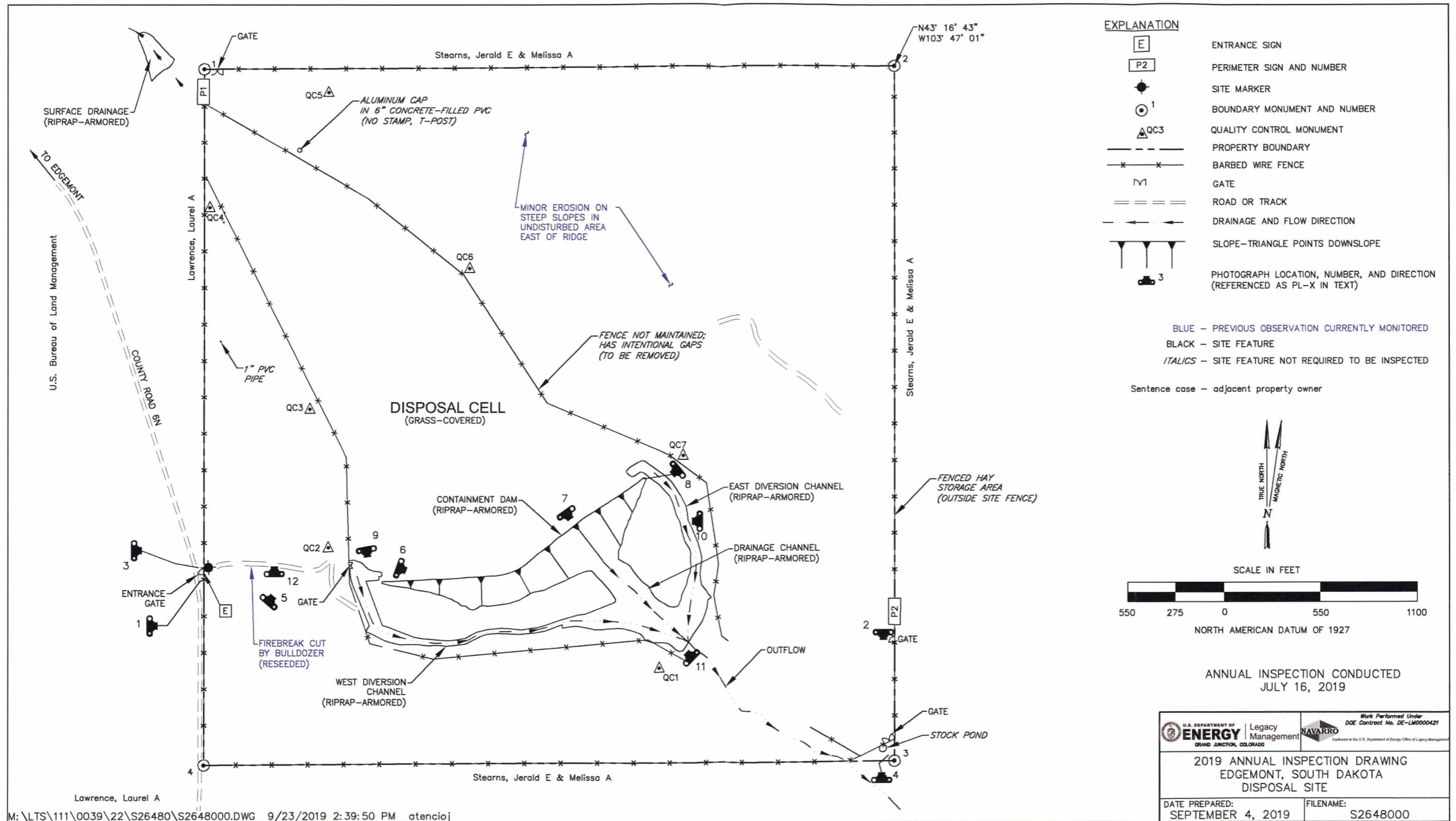
Figure 2-1. 2019 Annual Inspection Drawing for the Edgemont, South Dakota, Disposal Site
