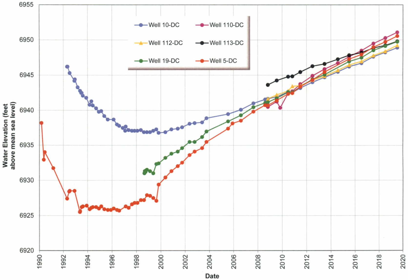
Figure 6-13. Hydrographs for Main Sand Aquifer Wells at the Shirley Basin South, Wyoming, Disposal Site
