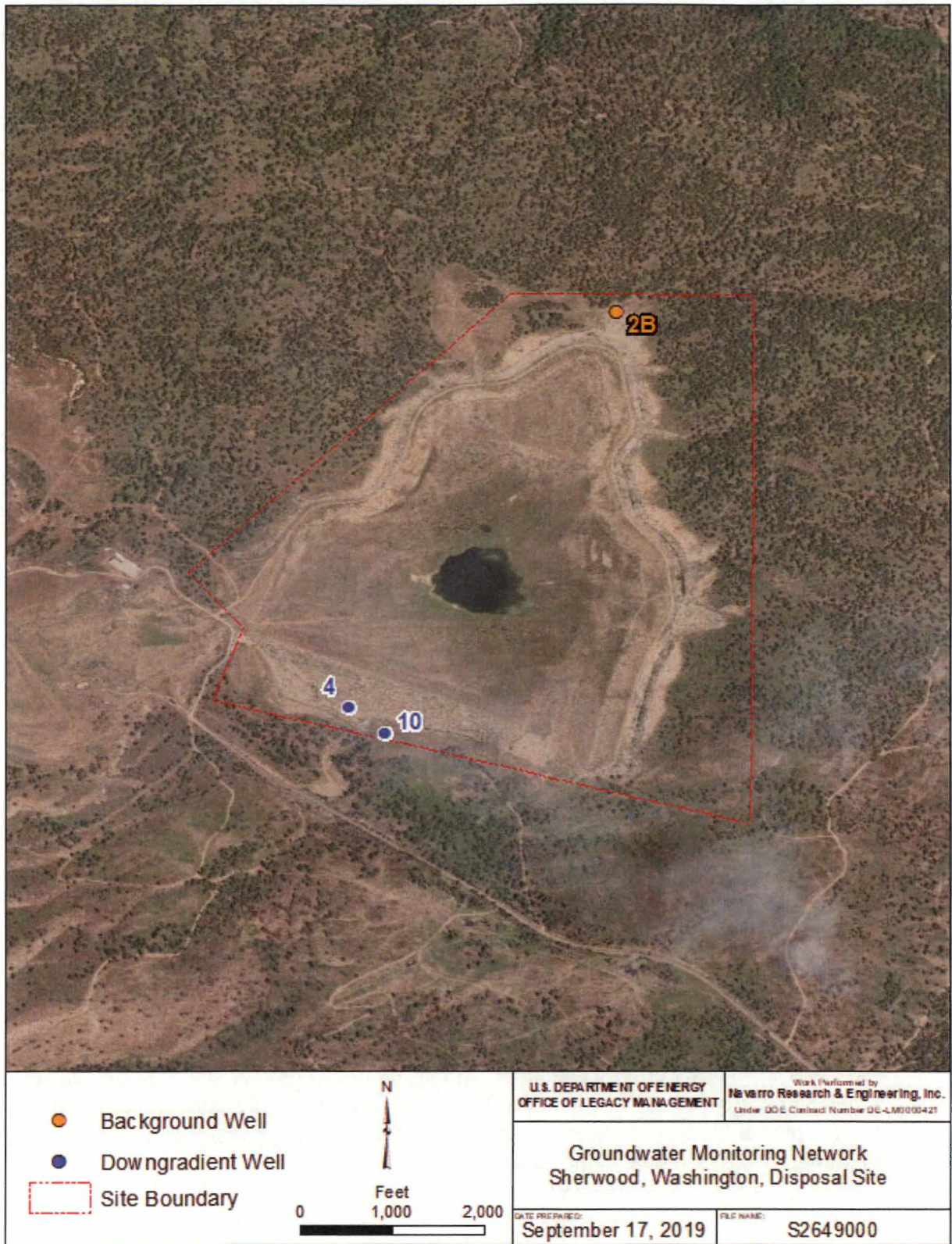
Figure 5-2. Groundwater Monitoring Network at Sherwood, Washington, Disposal Site
