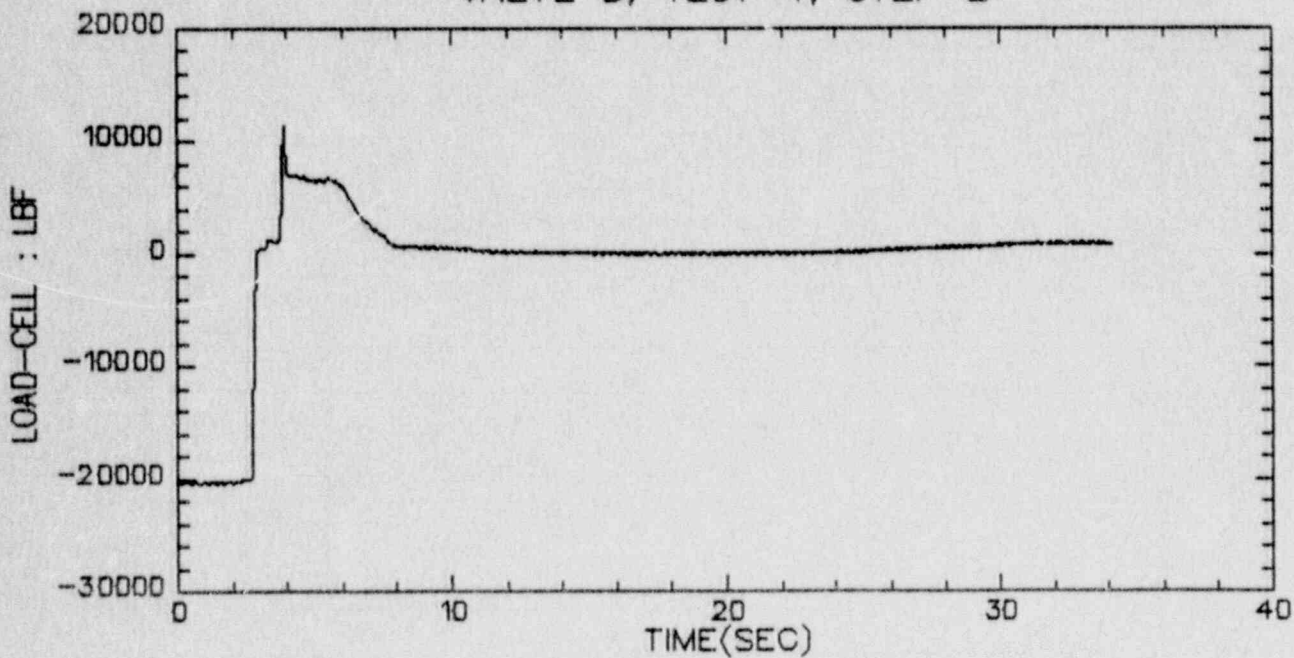
VALVE B, TEST 4, STEP 2
