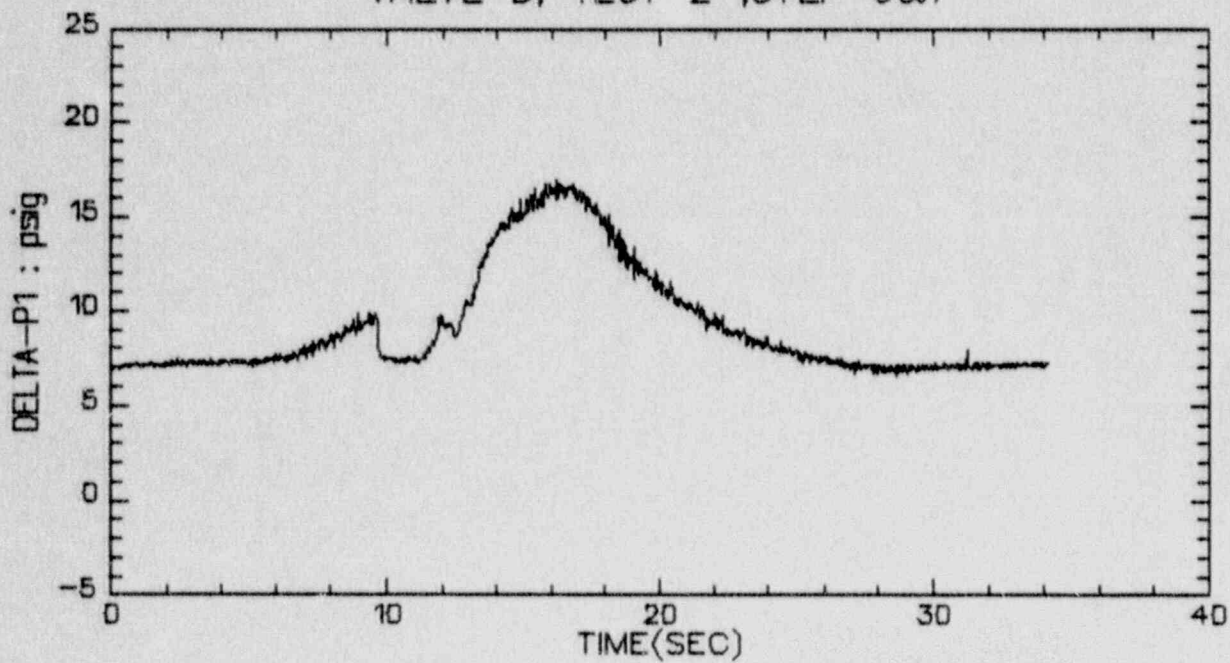
VALVE B, TEST 2 ,STEP 6&7
