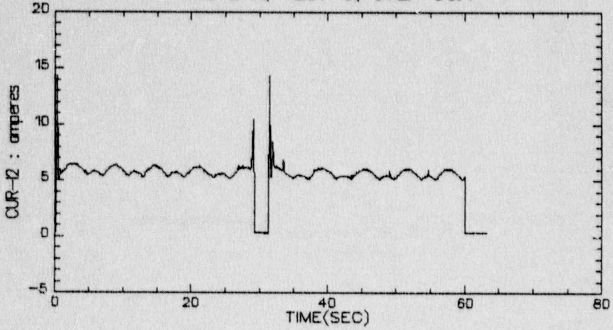
VALVE A, TEST 5, STEP 3&4
