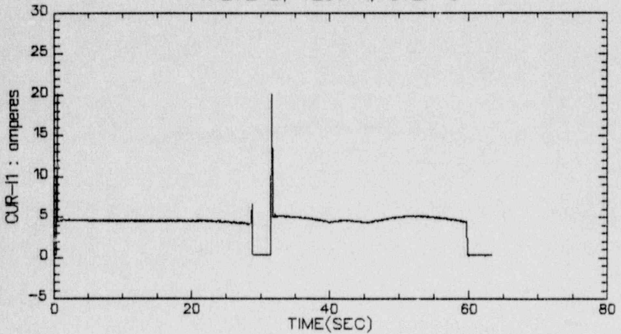
VALVE B, TEST 1, STEP 9
