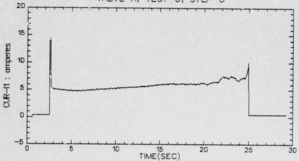
VALVE A, TEST 5, STEP 5
