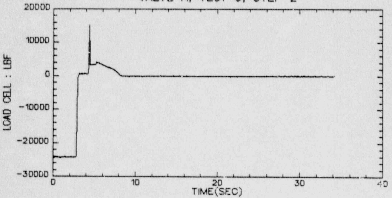
VALVE A, TEST 9, STEP 2
