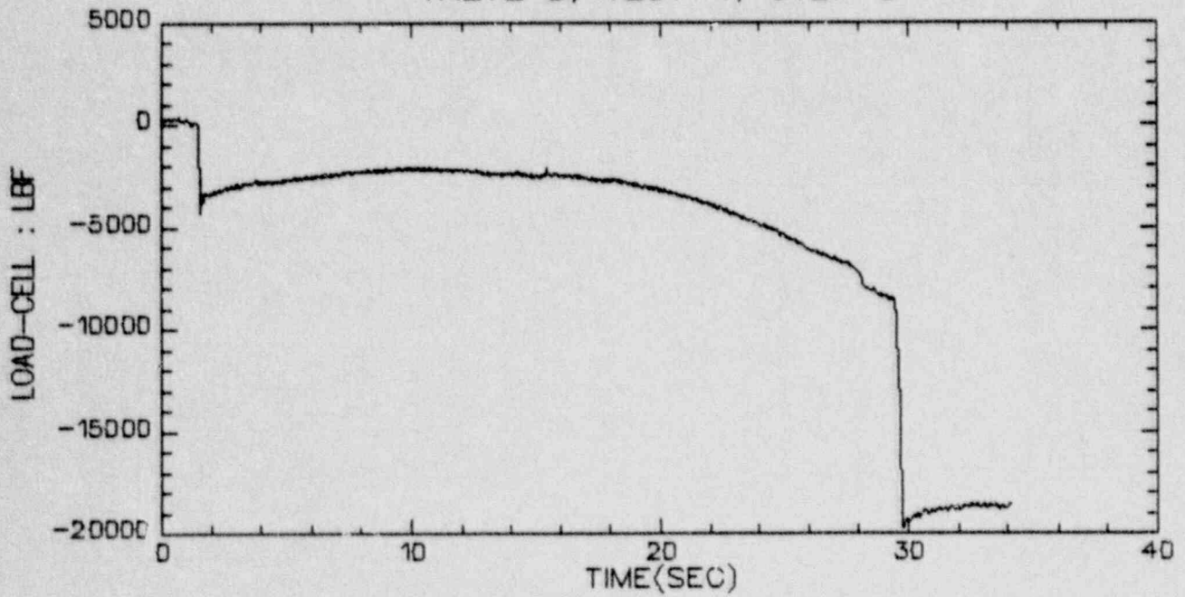
VALVE B, TEST 4, STEP 5
