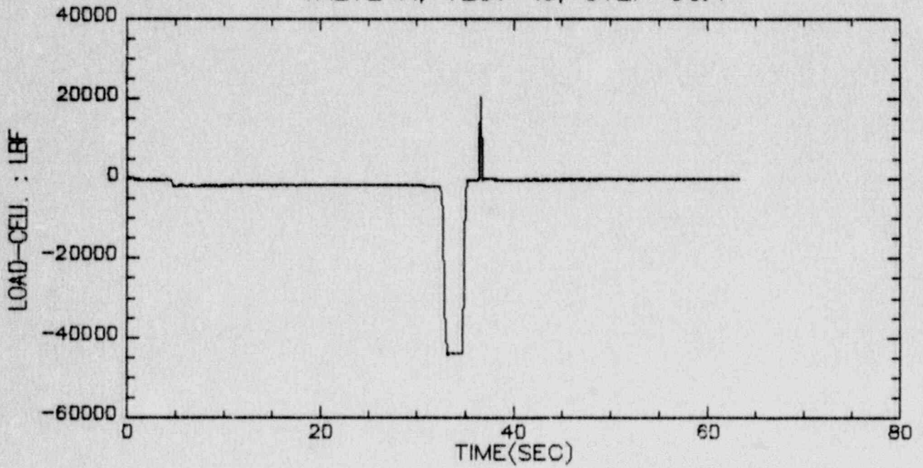
VALVE A, TEST 10, STEP 3&4
