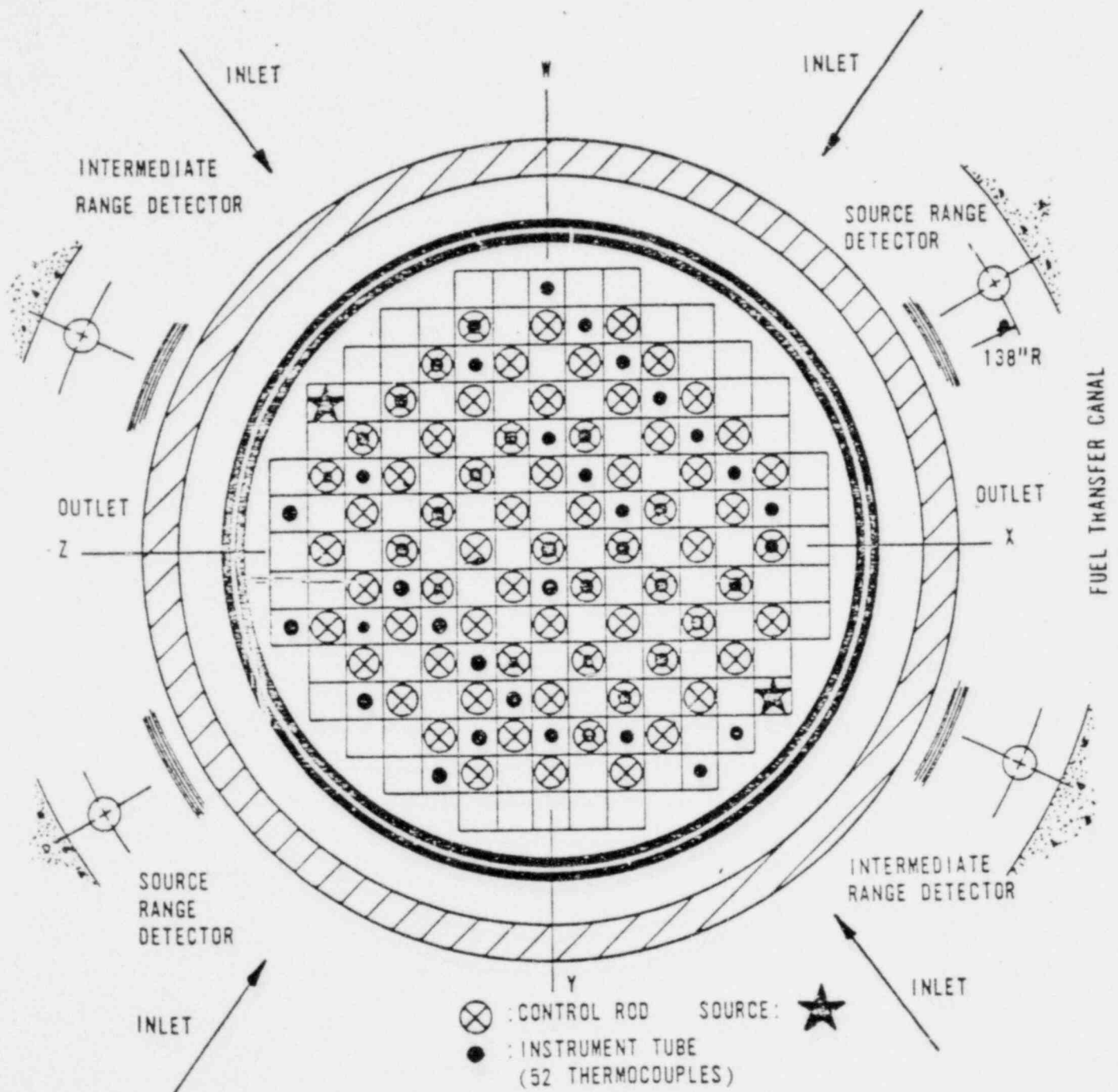
Figure 4.1-1 Layout of Core Thermocouples
