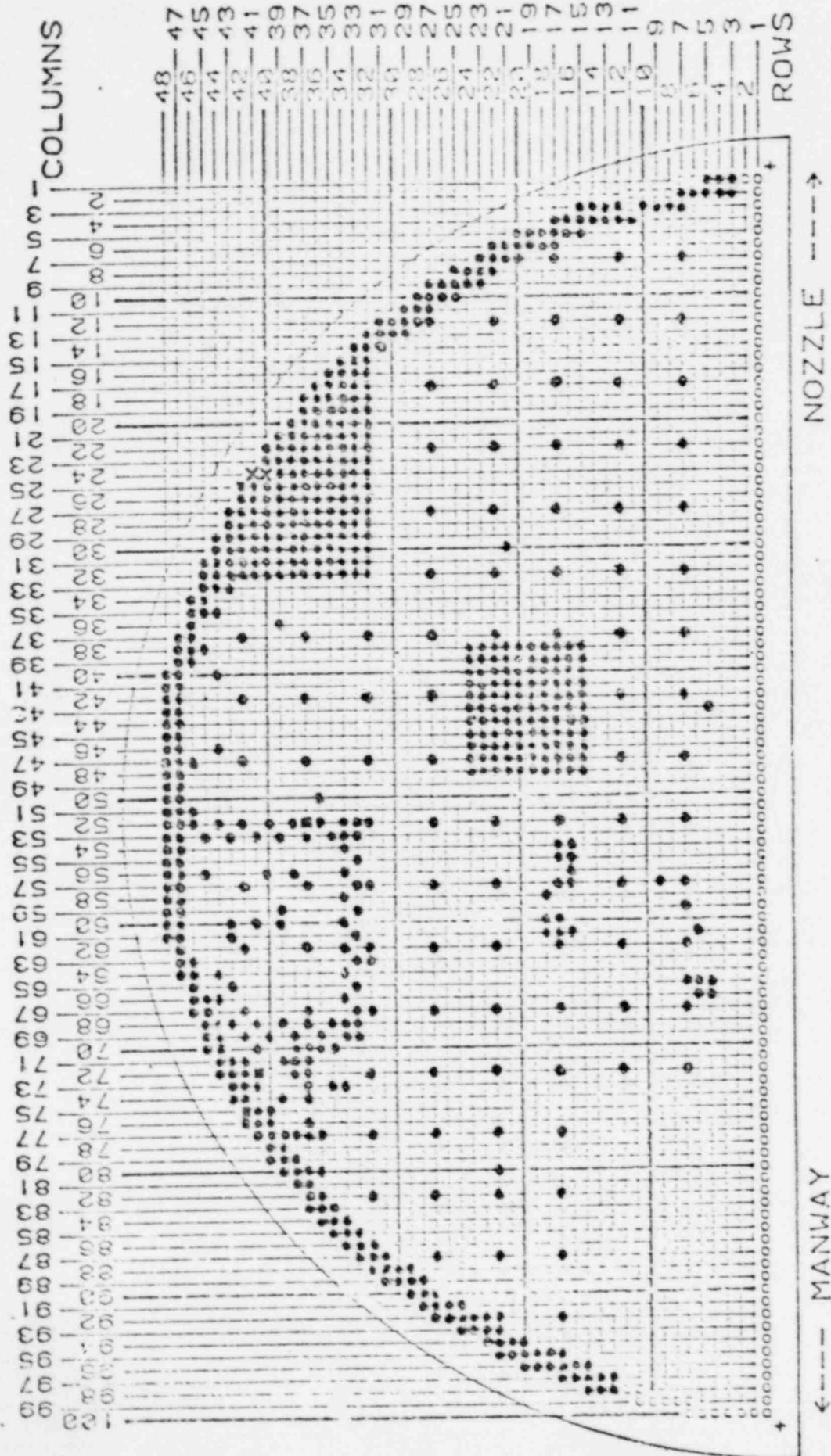
FIGURE NO. 2 Steam Generator No. 2 Examination Pattern
