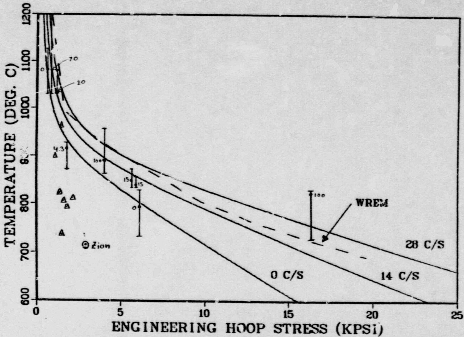
Fig. 4. WREM model and GRNL correlation of rupture temperature as a function of engineering hoop stress and ramp rate, with PBF LBLOCA test results. Numbers adjacent to test data points are ramp rates in ^{\circ}\text{C}/\text{sec} . TREAT data points are shown as triangles. The Zion high burnup pin estimate is given by a circle.
