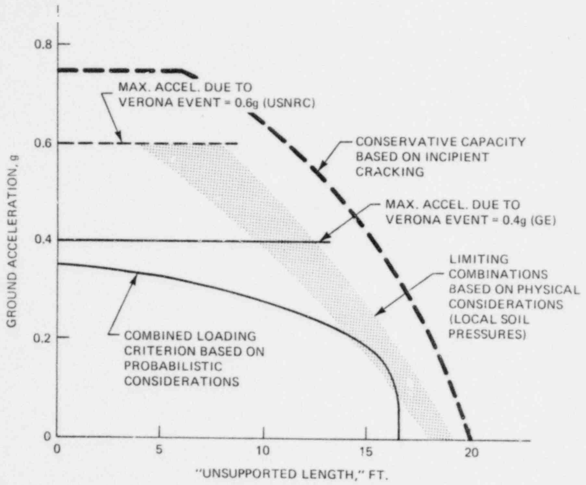
FIGURE 6. LOADING VS. CAPACITY
